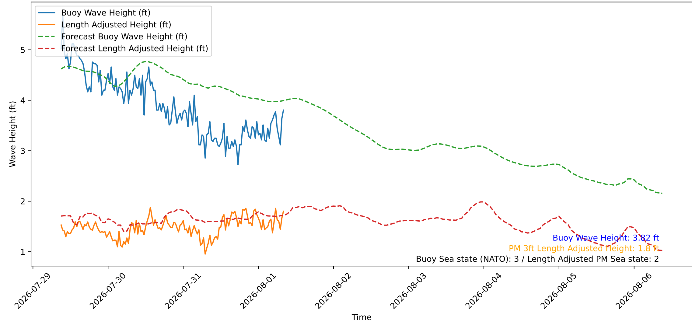
Wave Heights over Time for Oceanside Harbor at 2026-08-01 09:10:26
