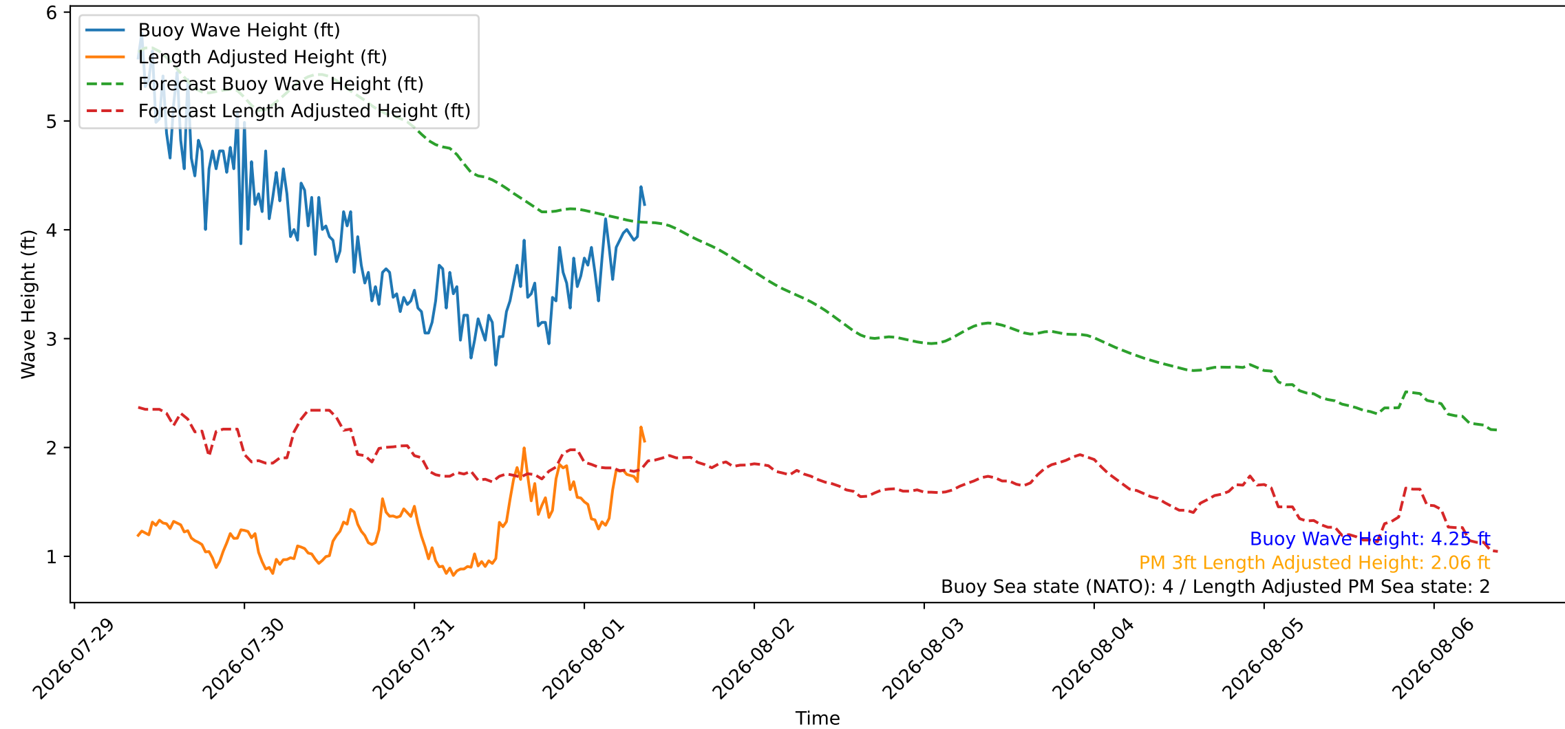
Wave Heights over Time for Green Beach at 2026-08-01 09:11:08
