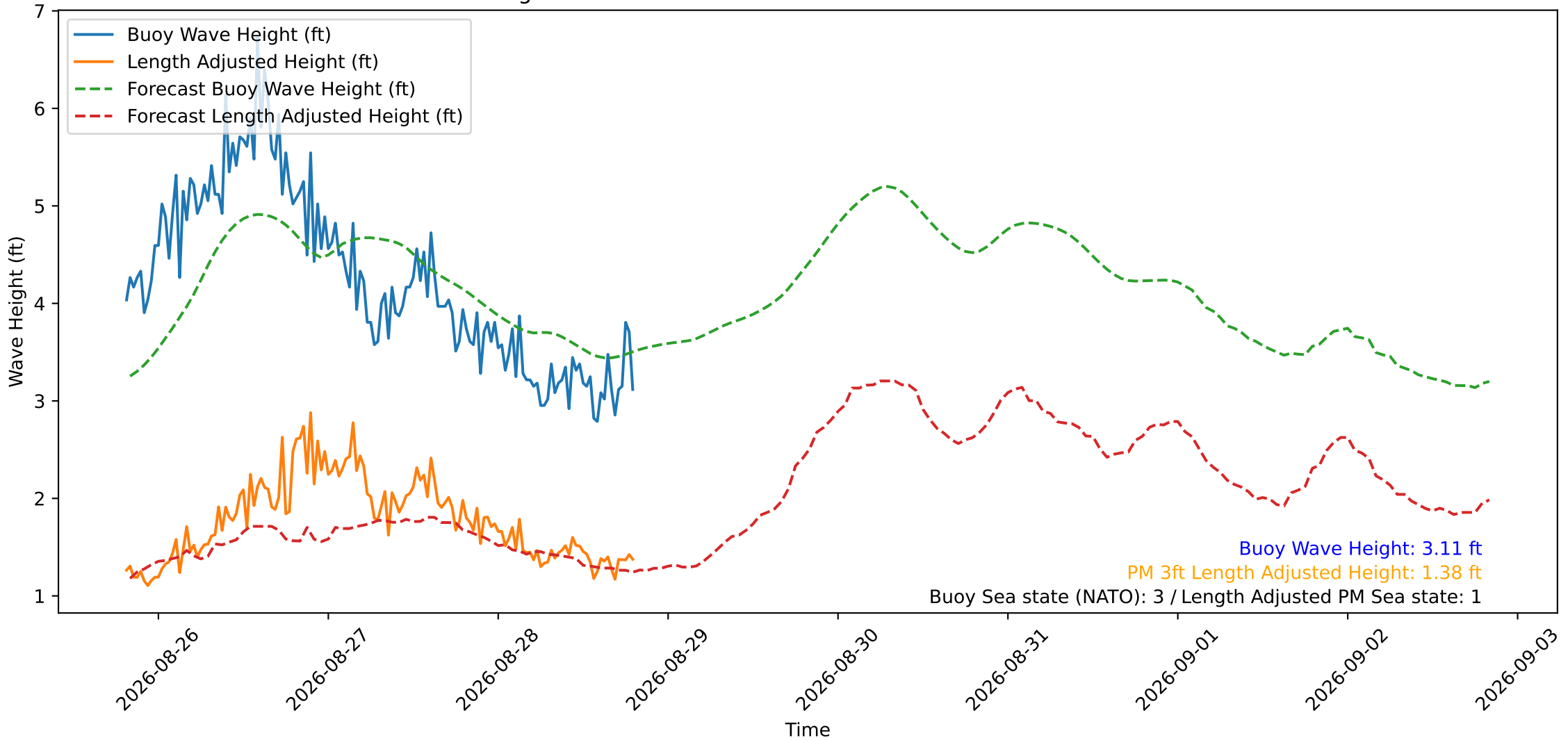
Wave Heights over Time for Oceanside Harbor at 2026-08-28 19:40:29
