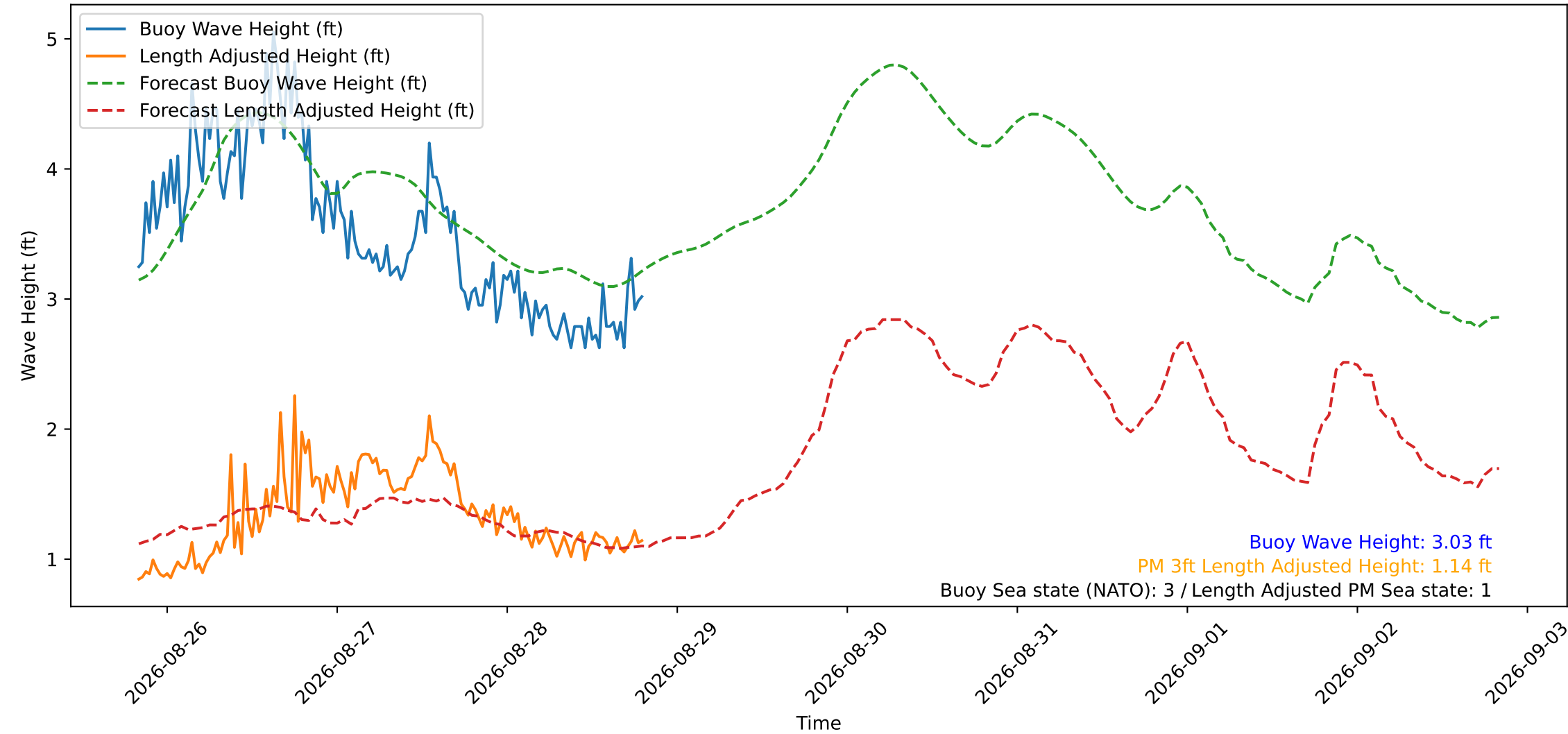
Wave Heights over Time for Red Beach at 2026-08-28 19:40:49
