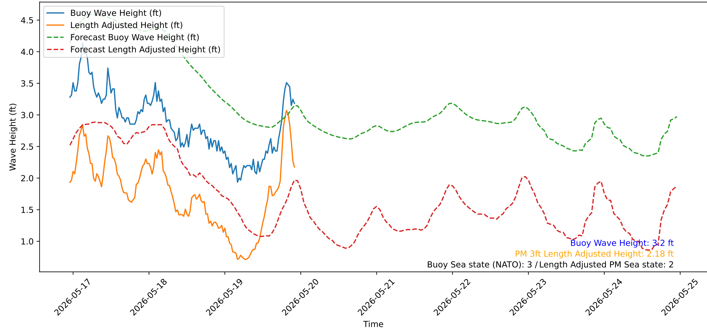
Wave Heights over Time for Red Beach at 2026-05-19 22:50:52
