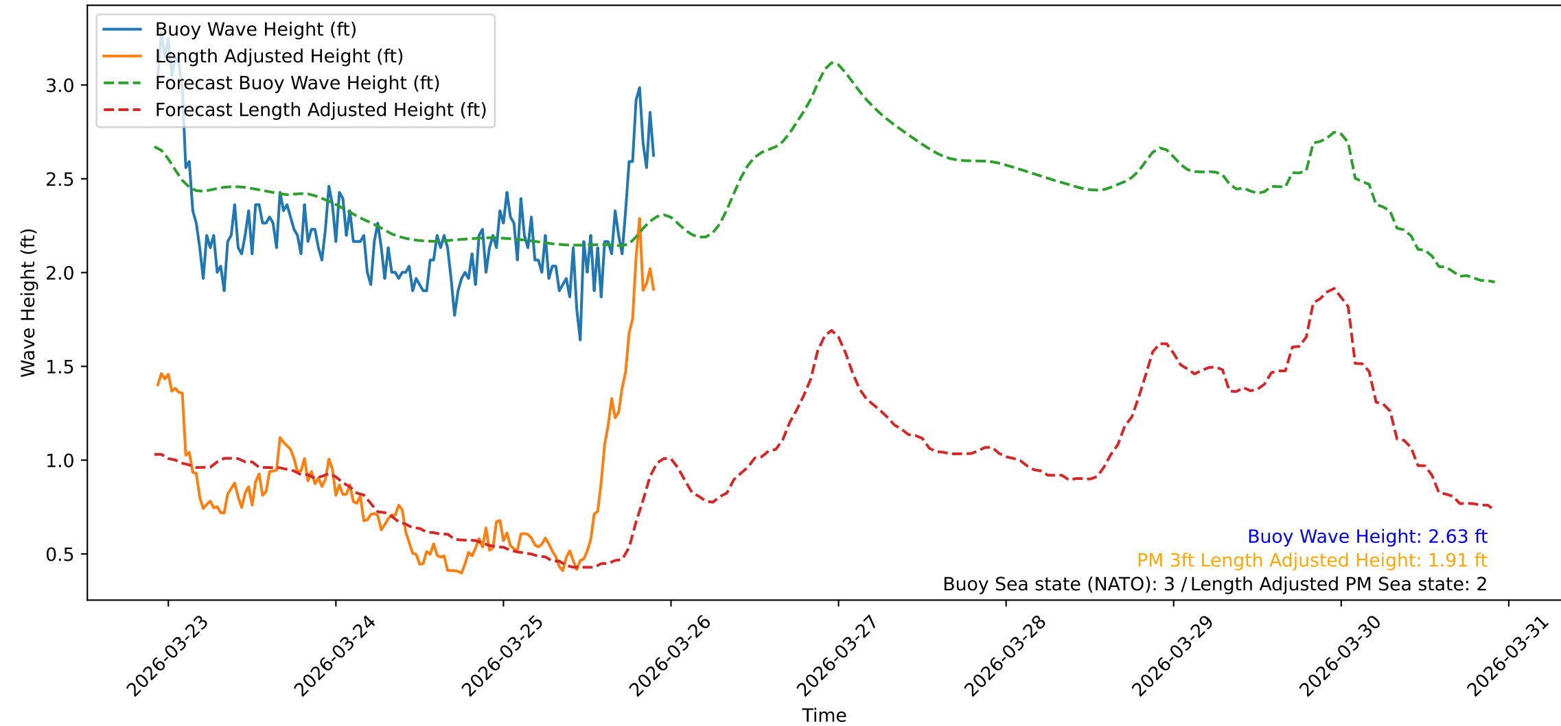
Wave Heights over Time for Green Beach at 2026-03-25 22:21:10
