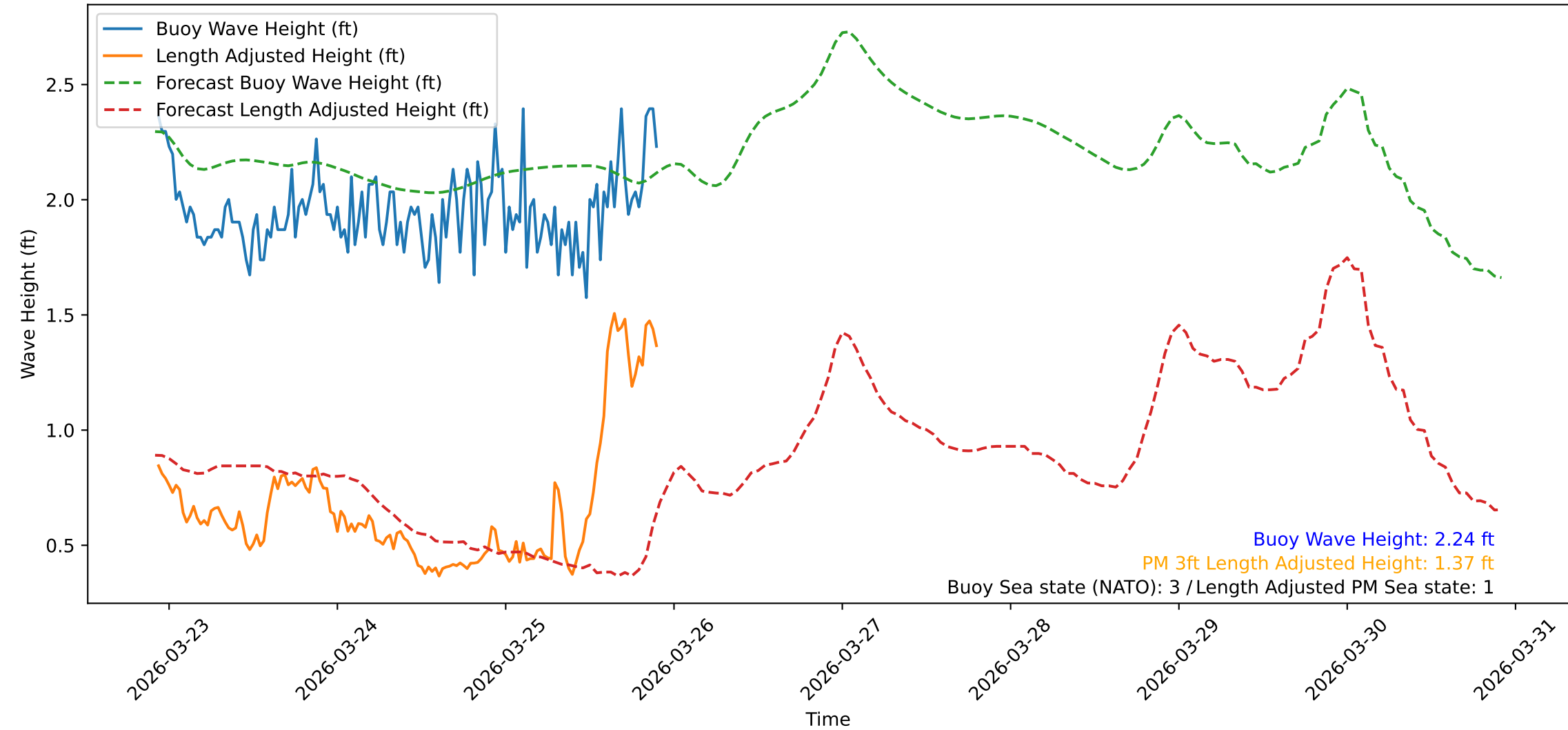
Wave Heights over Time for Red Beach at 2026-03-25 22:20:48
