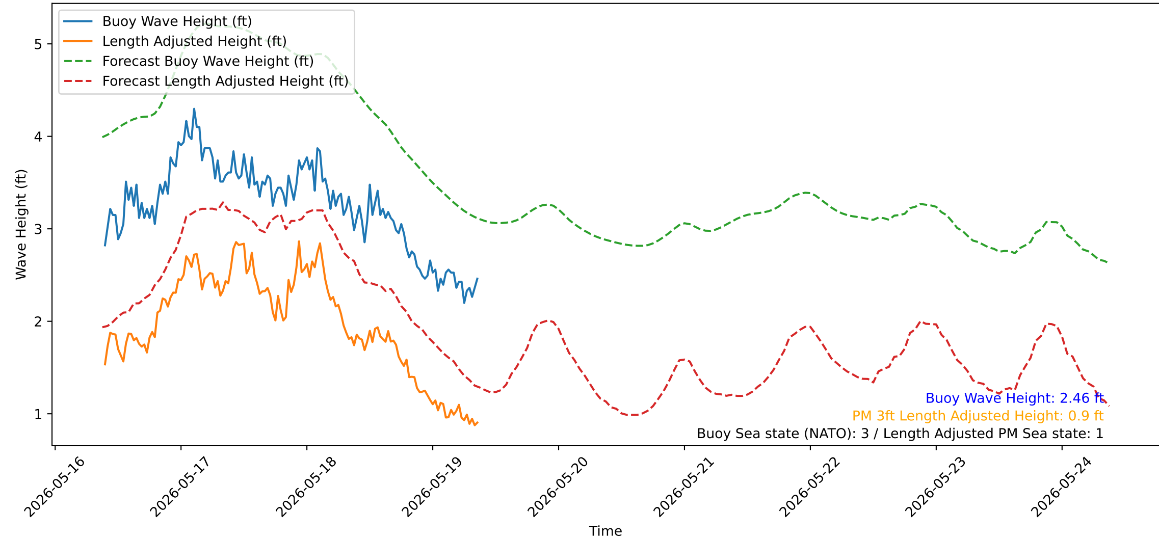
Wave Heights over Time for Oceanside Harbor at 2026-05-19 09:20:32
