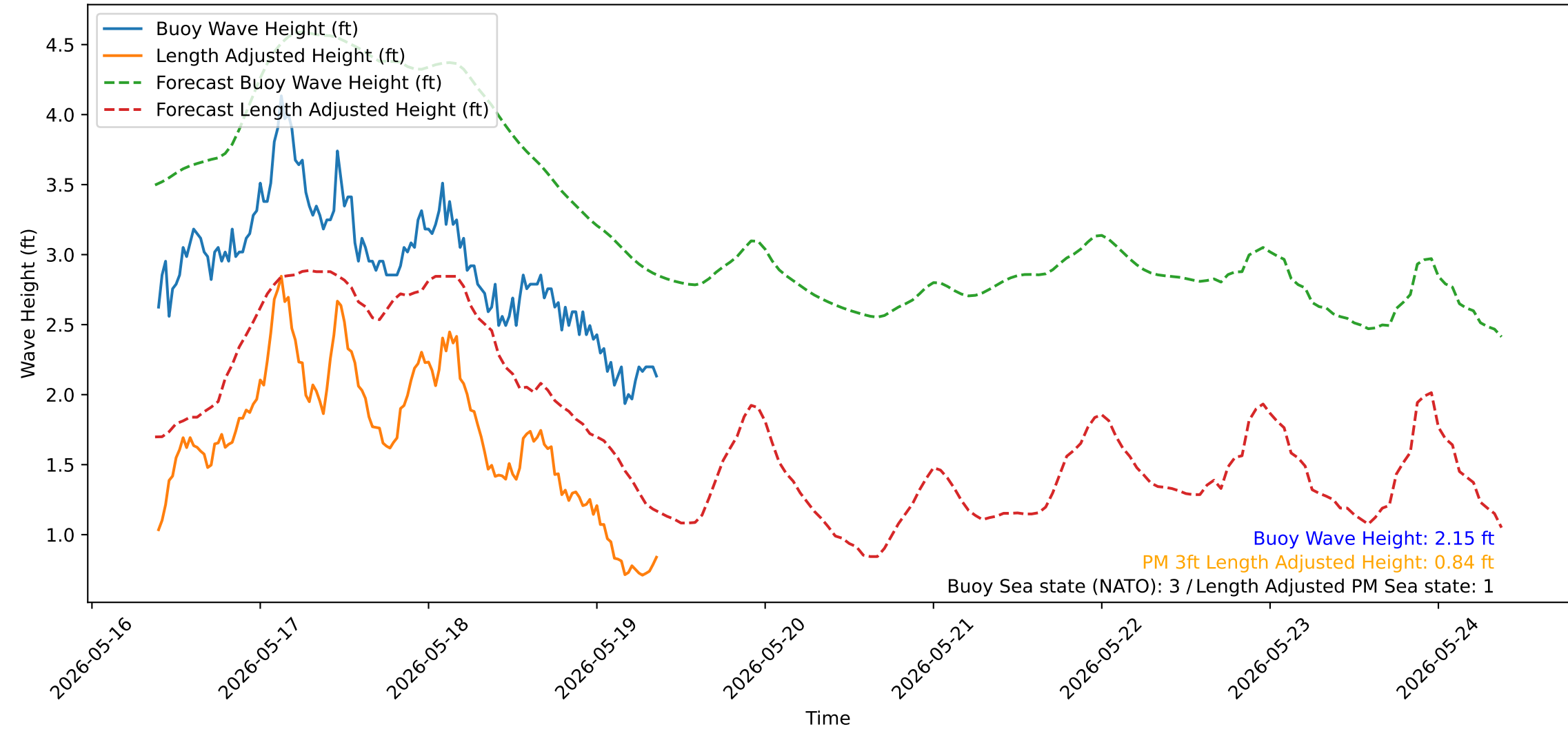
Wave Heights over Time for Red Beach at 2026-05-19 09:20:52
