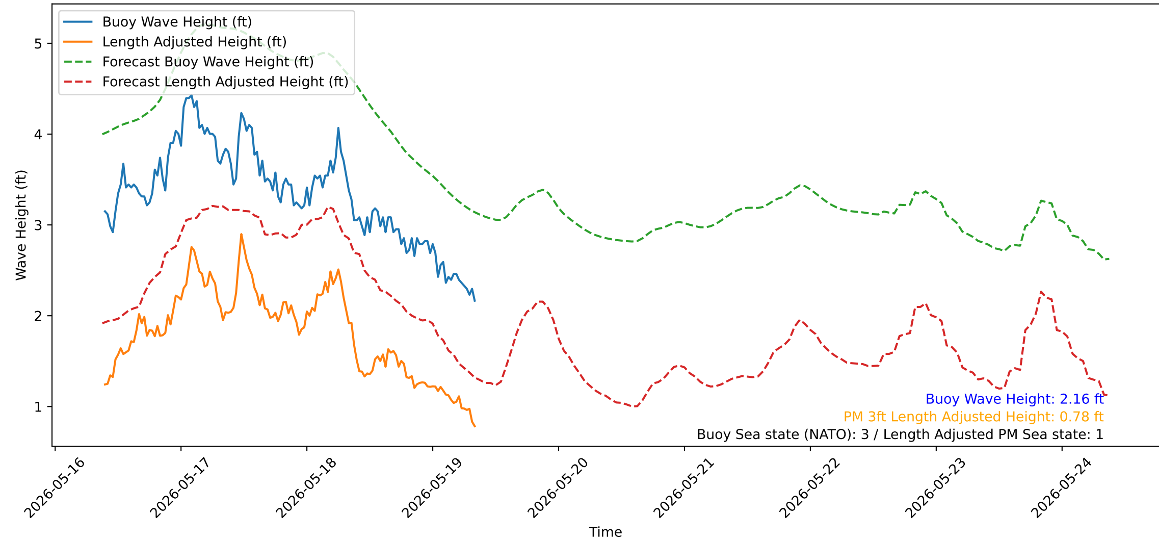
Wave Heights over Time for Green Beach at 2026-05-19 09:21:15
