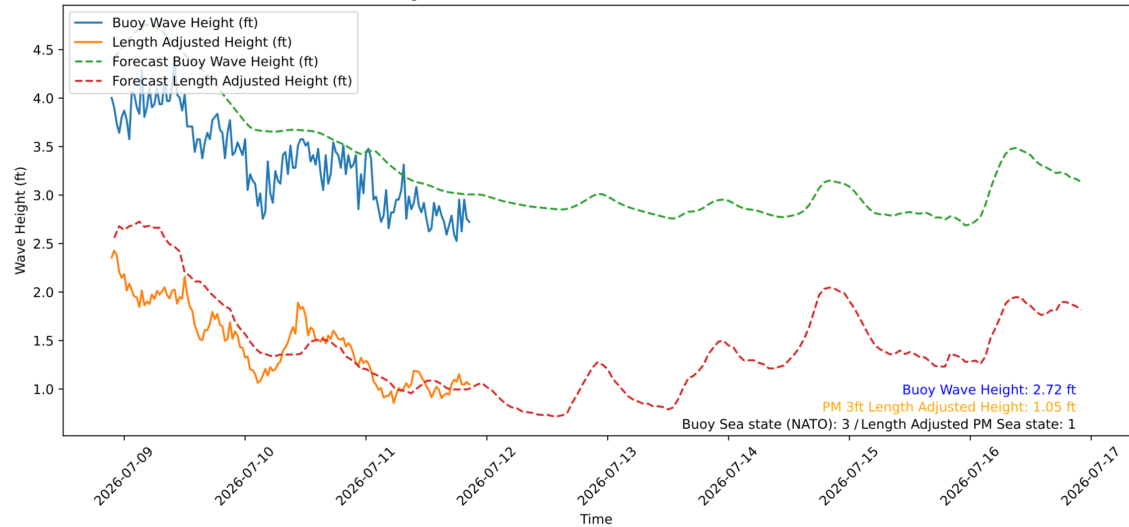
Wave Heights over Time for Green Beach at 2026-07-11 21:31:07
