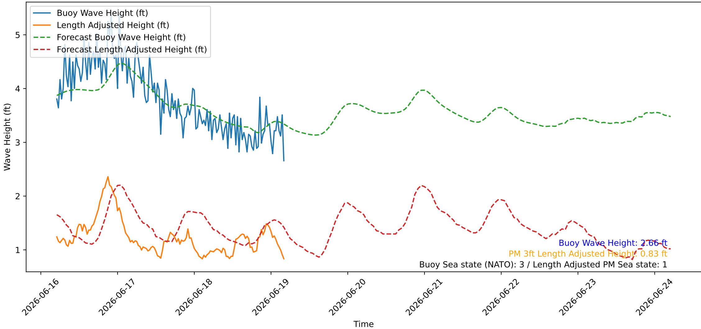
Wave Heights over Time for Red Beach at 2026-06-19 04:40:46
