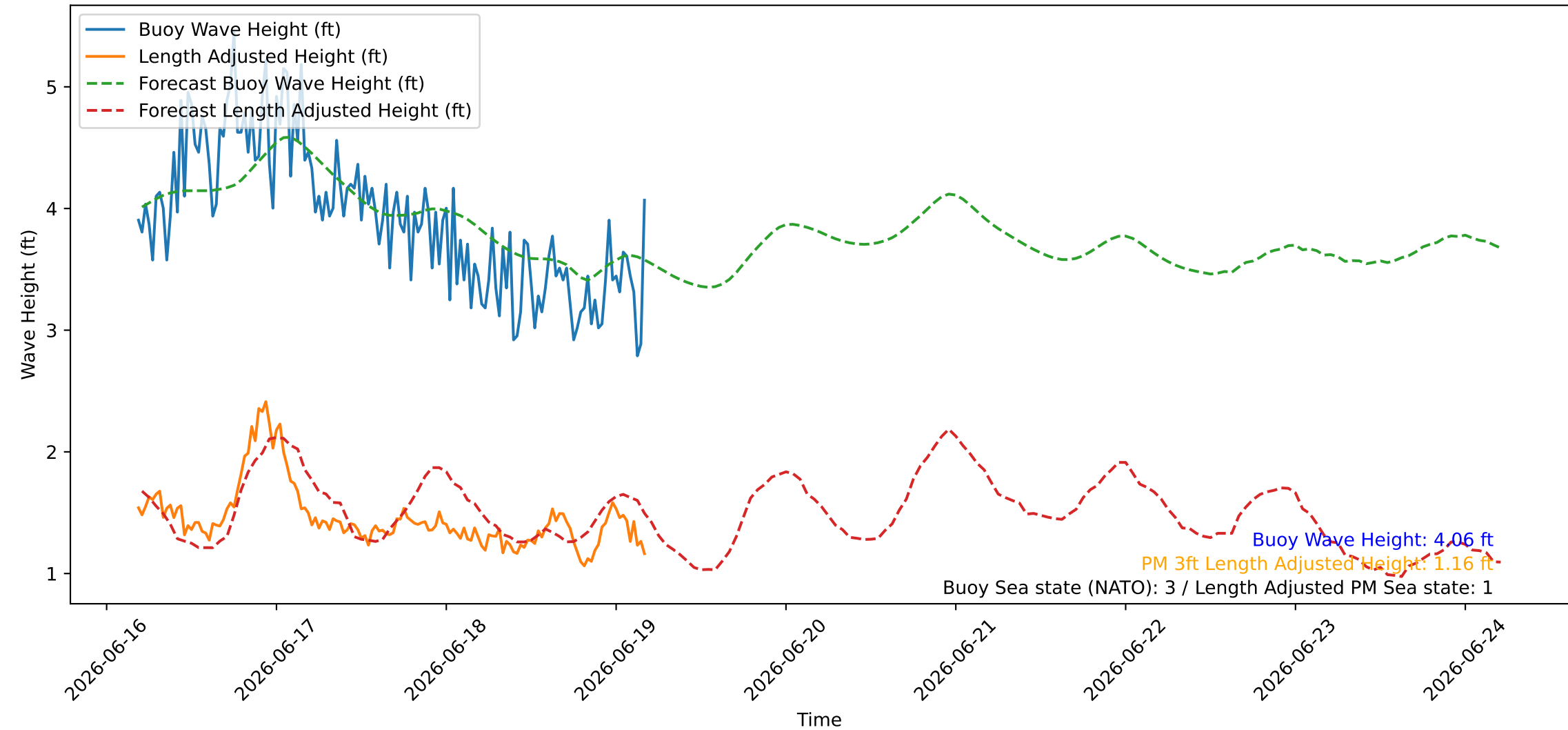
Wave Heights over Time for Oceanside Harbor at 2026-06-19 04:40:26
