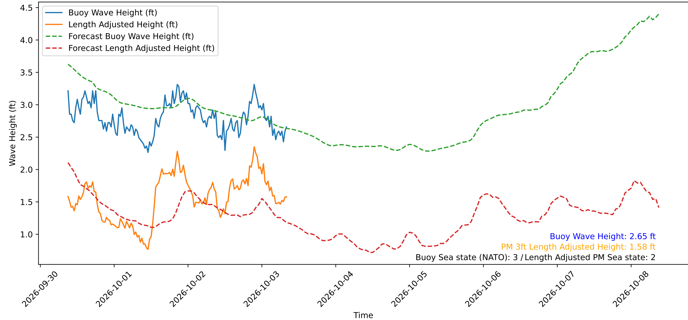
Wave Heights over Time for Oceanside Harbor at 2026-10-03 08:50:30
