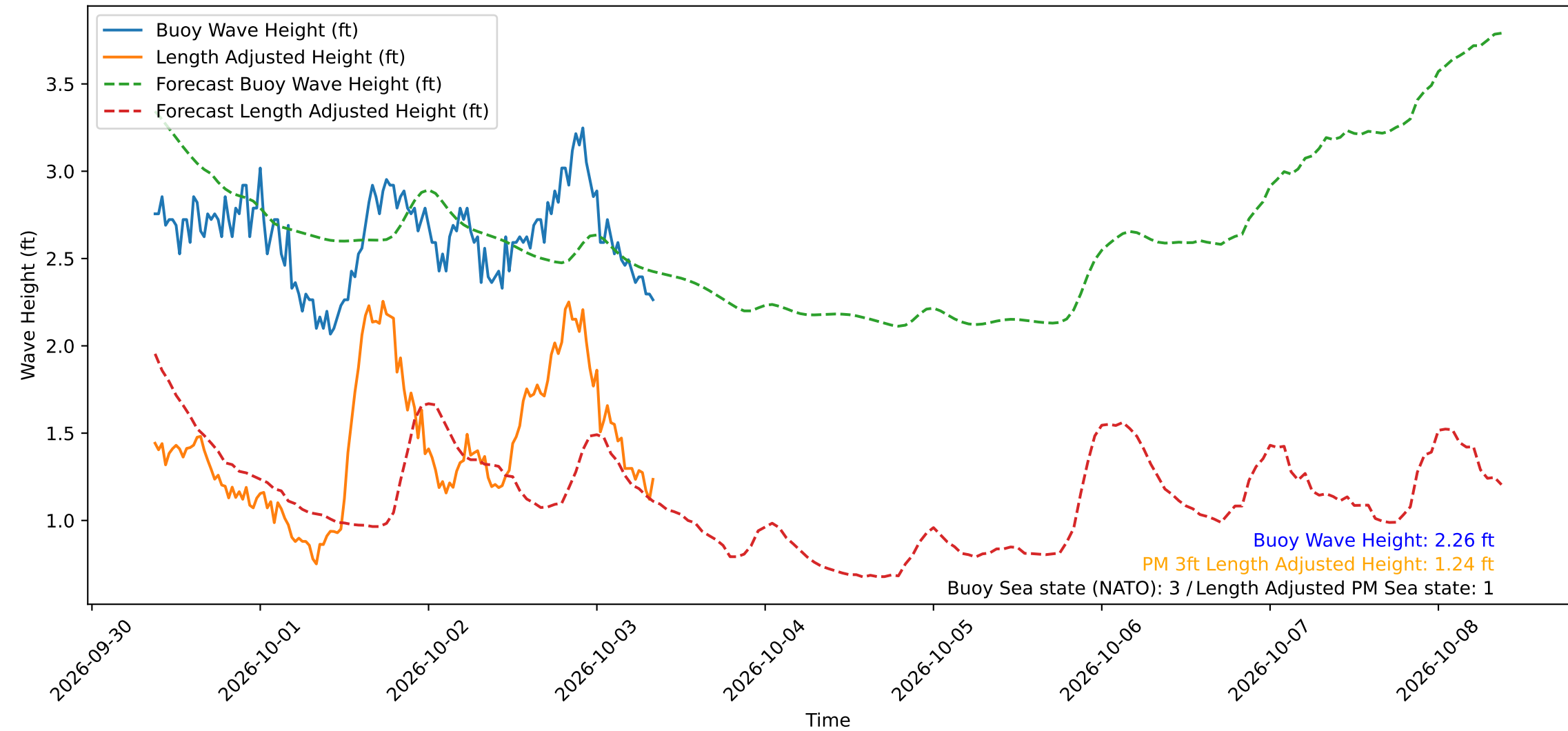
Wave Heights over Time for Red Beach at 2026-10-03 08:50:51
