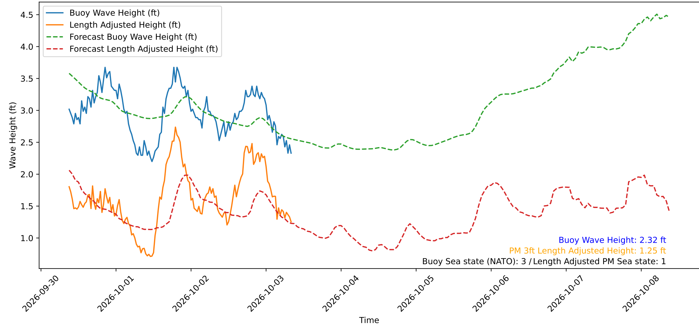
Wave Heights over Time for Green Beach at 2026-10-03 08:51:15
