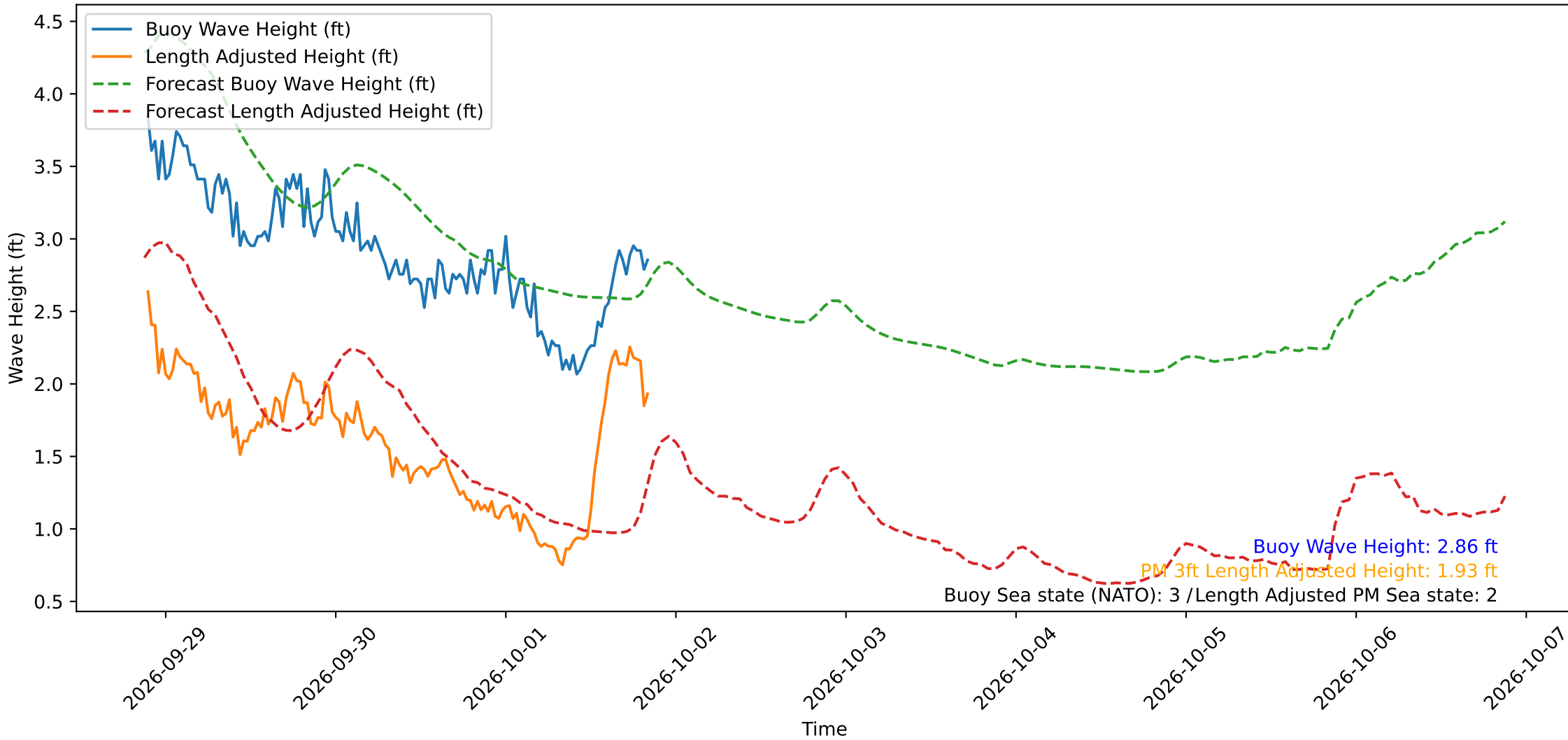
Wave Heights over Time for Red Beach at 2026-10-01 21:00:50
