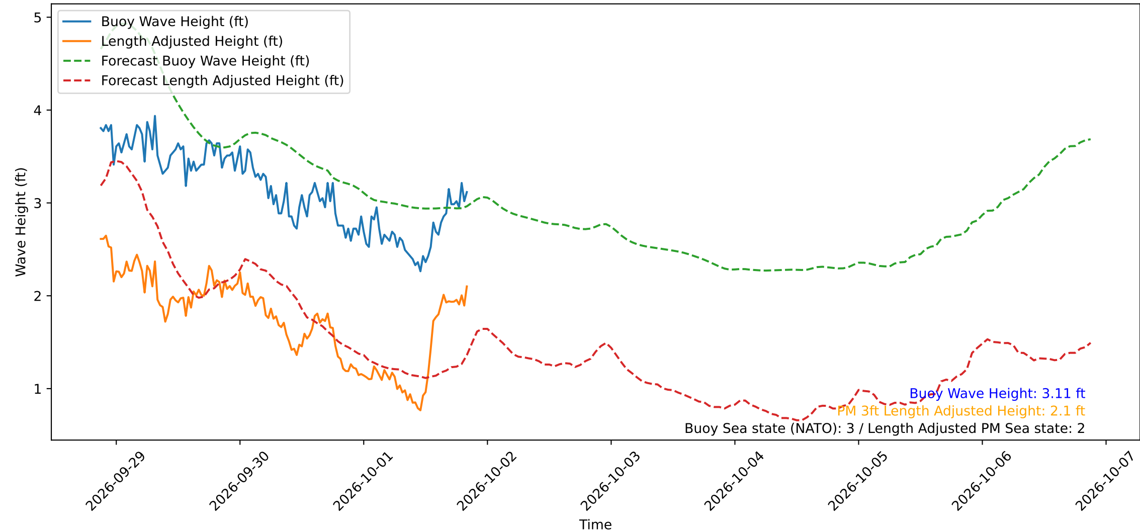
Wave Heights over Time for Oceanside Harbor at 2026-10-01 21:00:30
