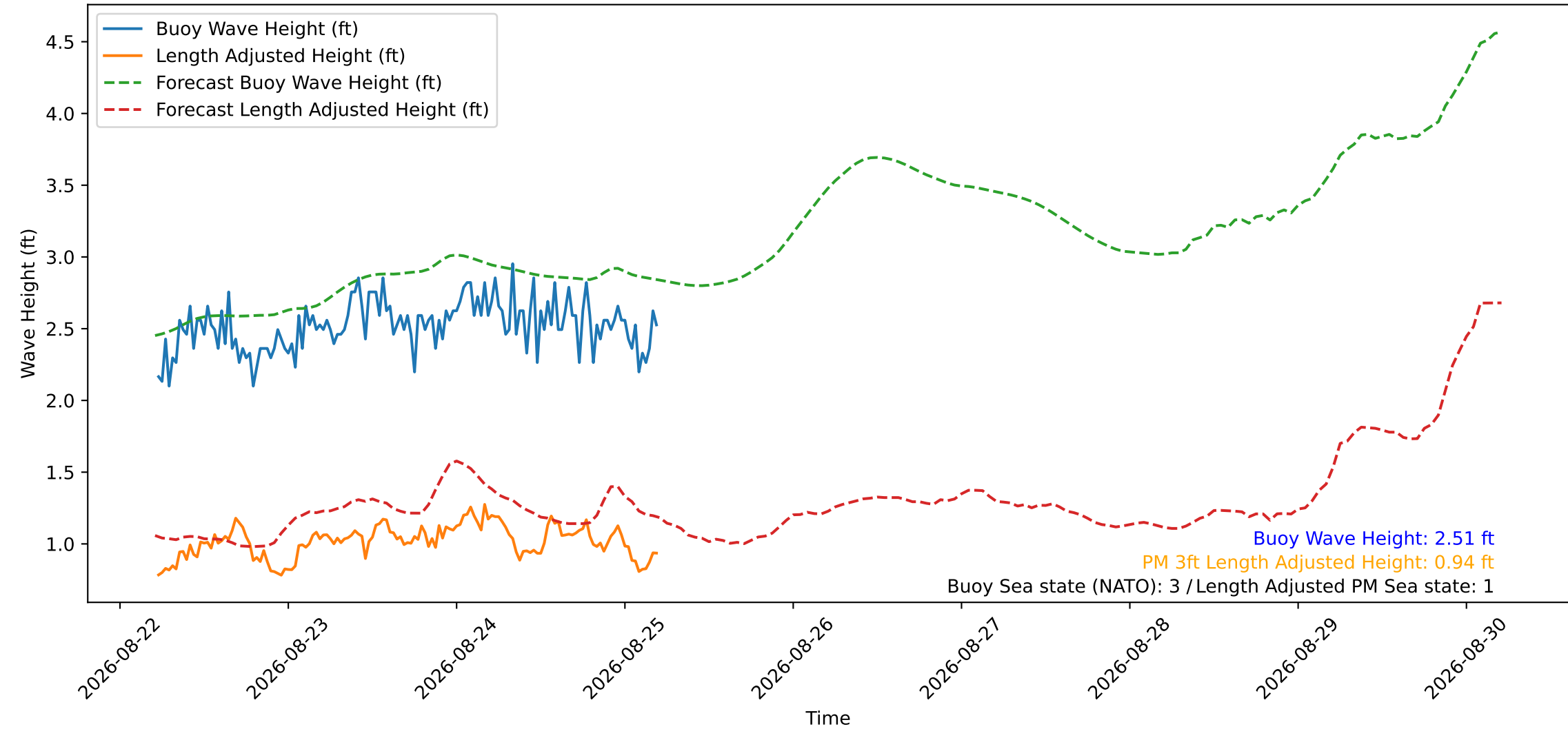
Wave Heights over Time for Red Beach at 2026-08-25 05:20:50
