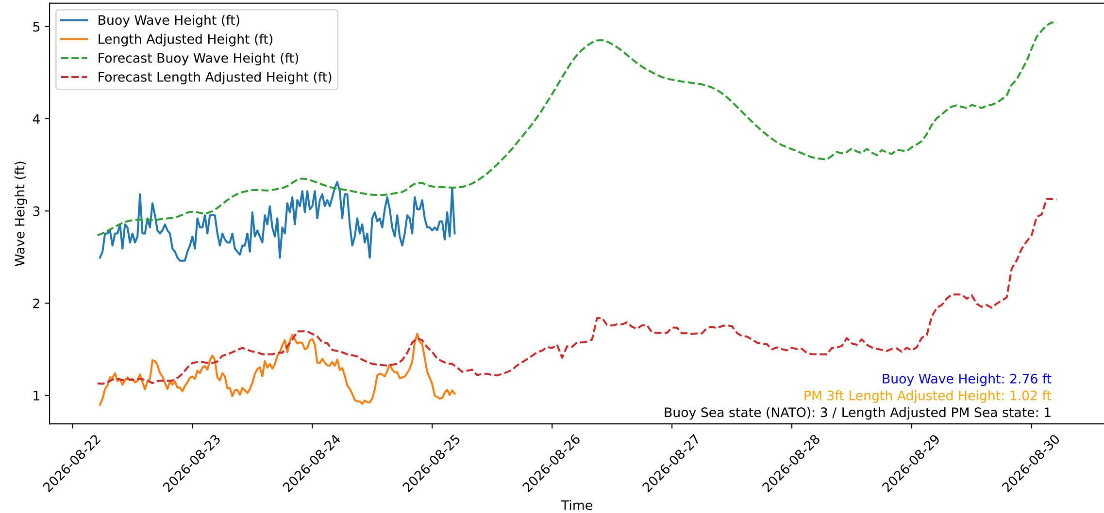
Wave Heights over Time for Green Beach at 2026-08-25 05:21:14
