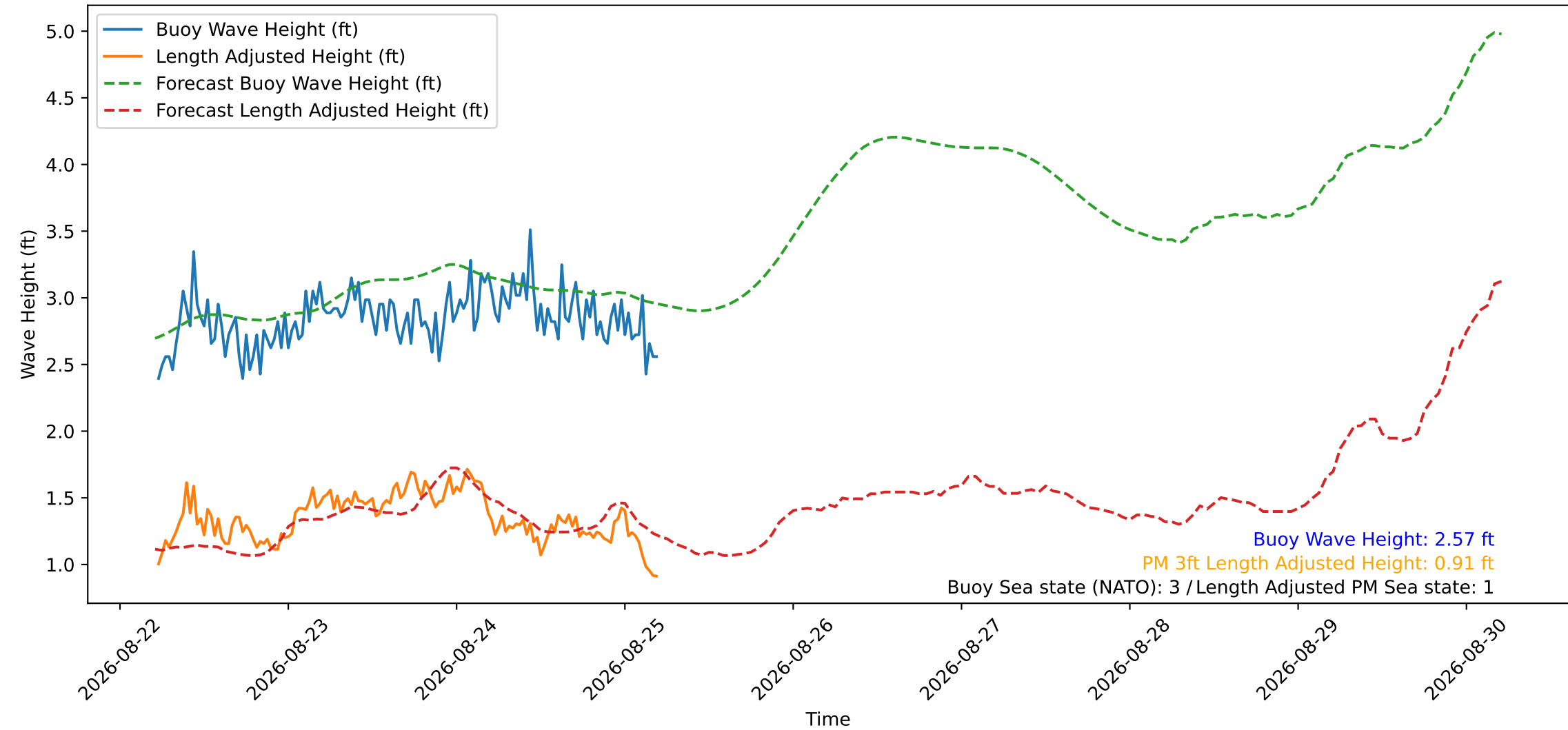
Wave Heights over Time for Oceanside Harbor at 2026-08-25 05:20:29
