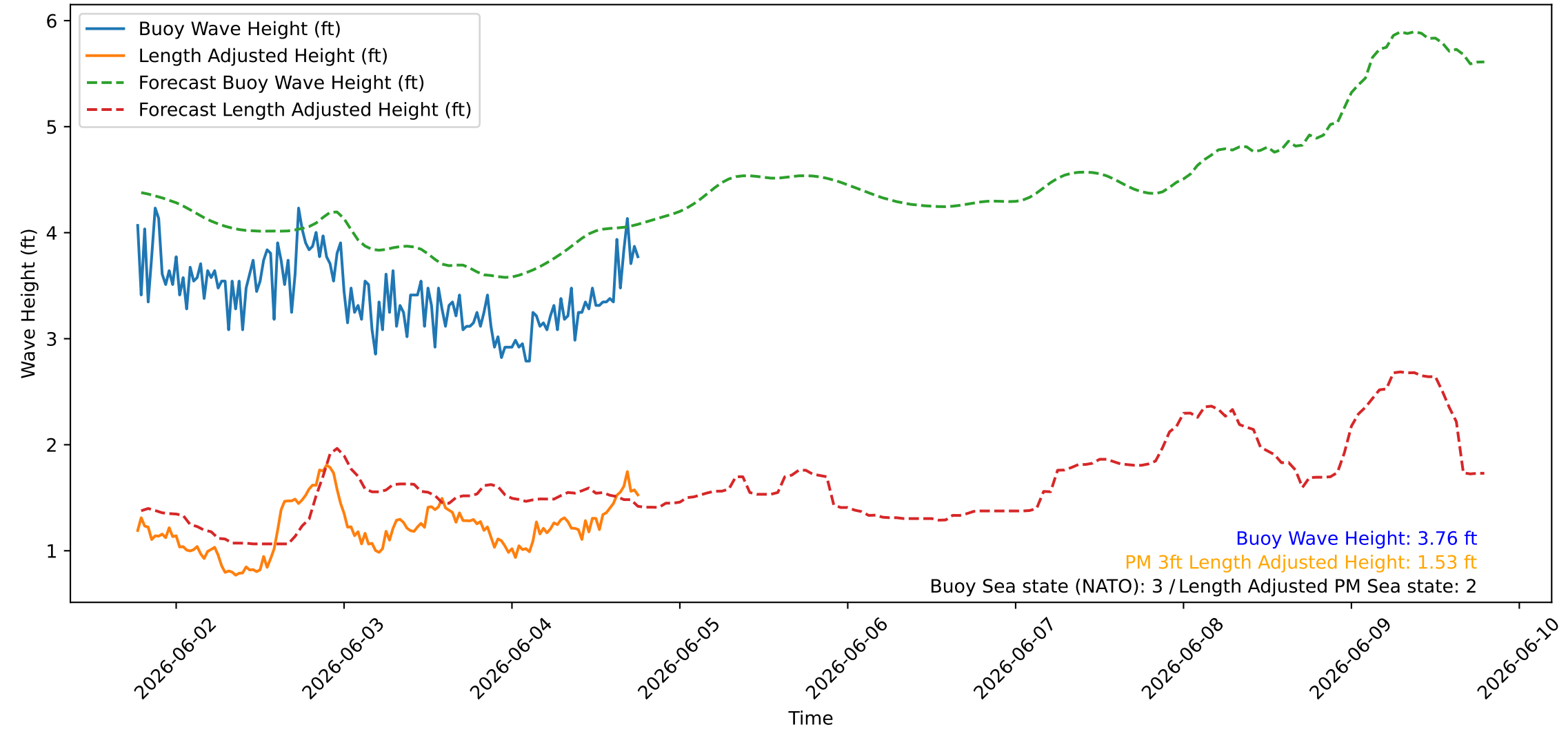
Wave Heights over Time for Green Beach at 2026-06-04 18:41:08
