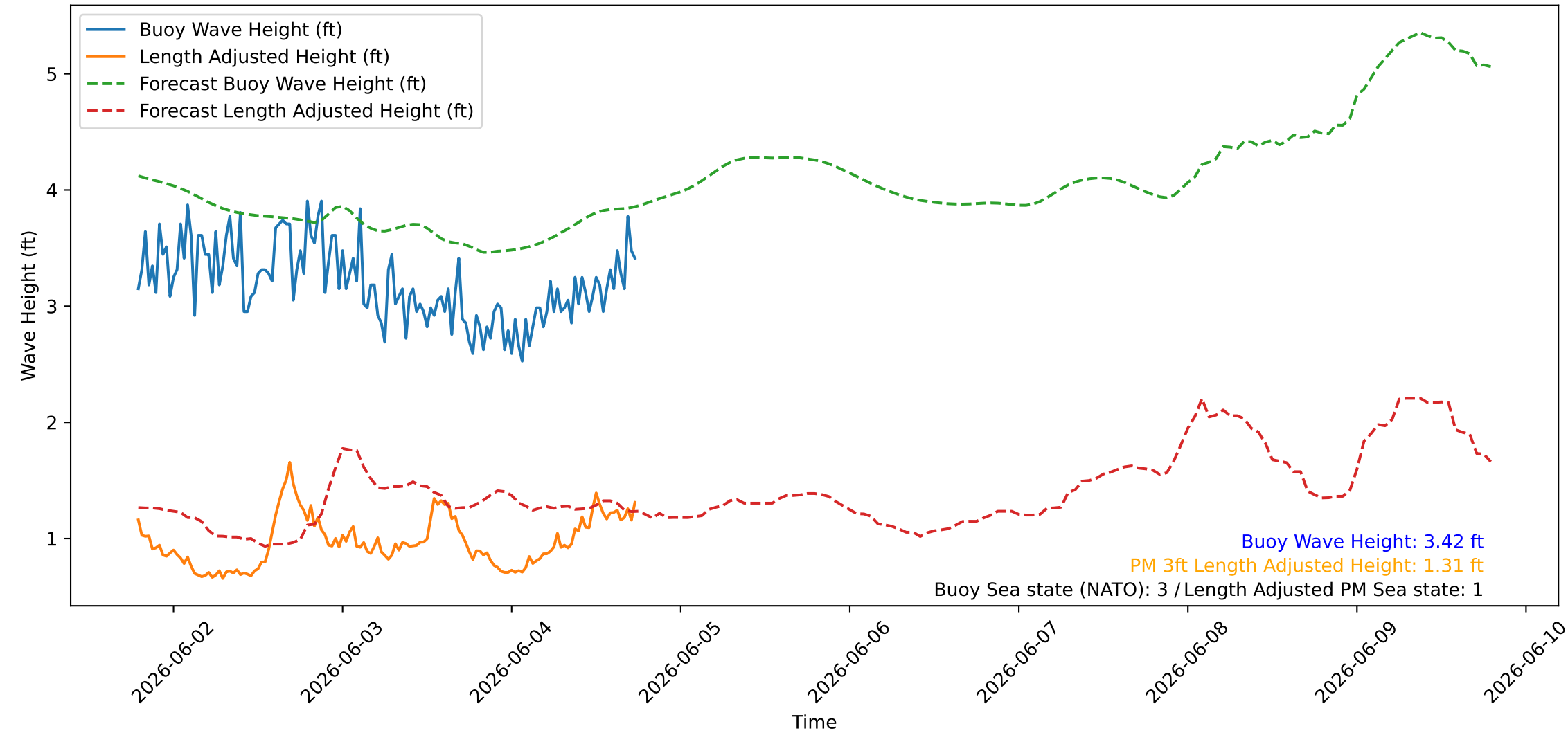
Wave Heights over Time for Red Beach at 2026-06-04 18:40:46
