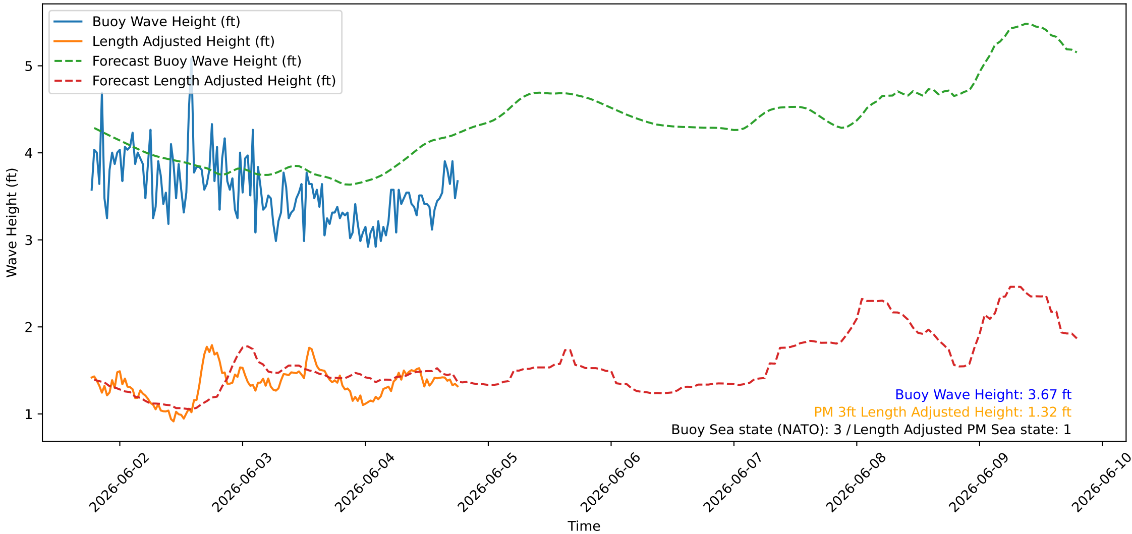
Wave Heights over Time for Oceanside Harbor at 2026-06-04 18:40:26
