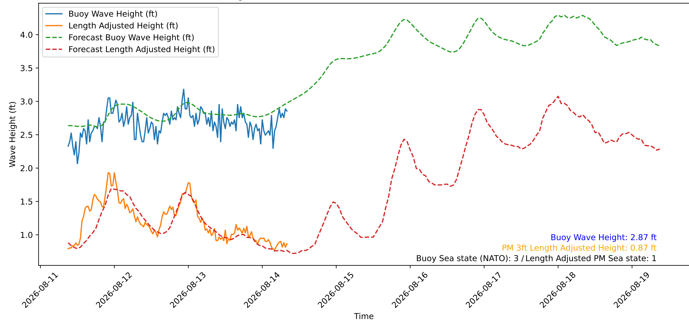
Wave Heights over Time for Oceanside Harbor at 2026-08-14 08:50:26
