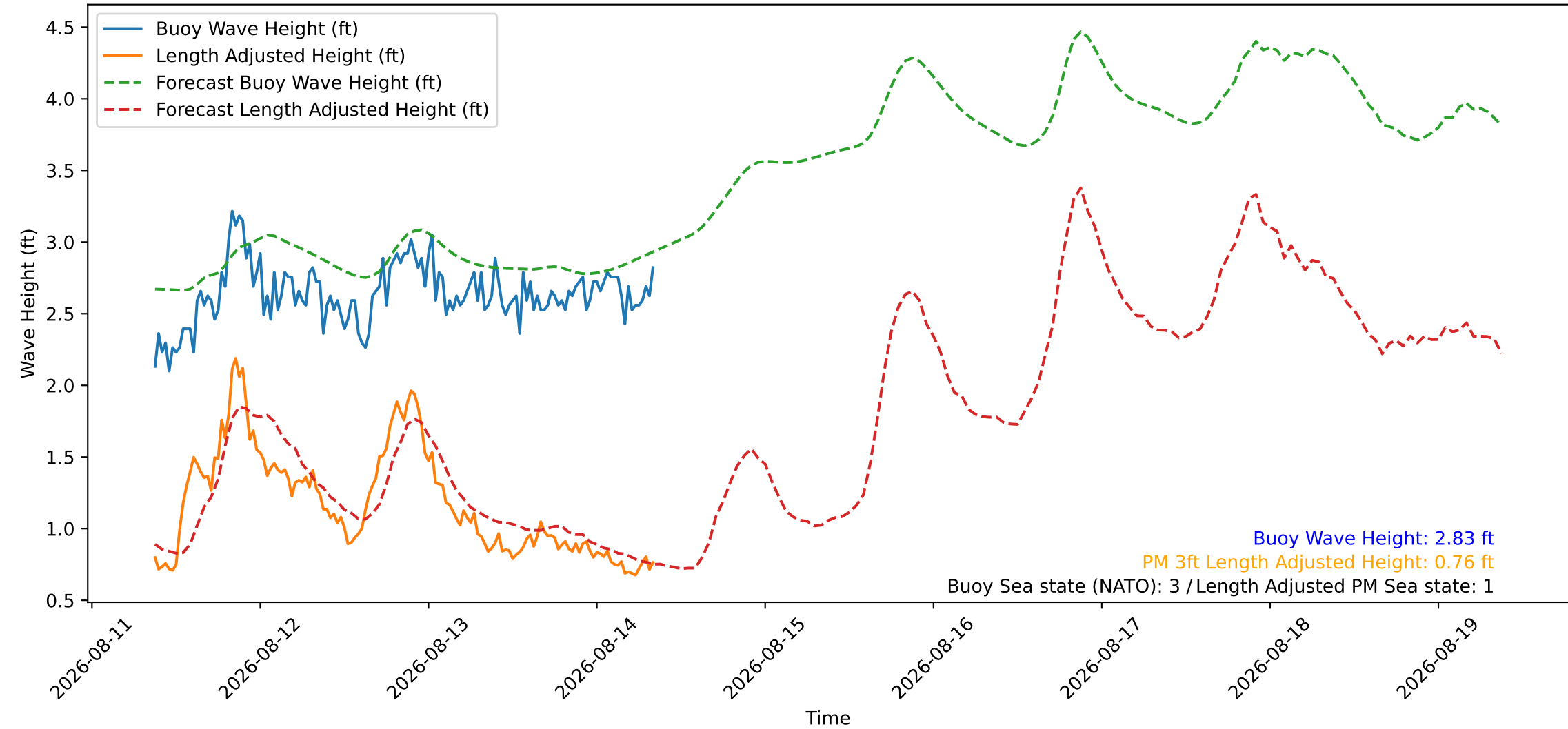
Wave Heights over Time for Green Beach at 2026-08-14 08:51:09
