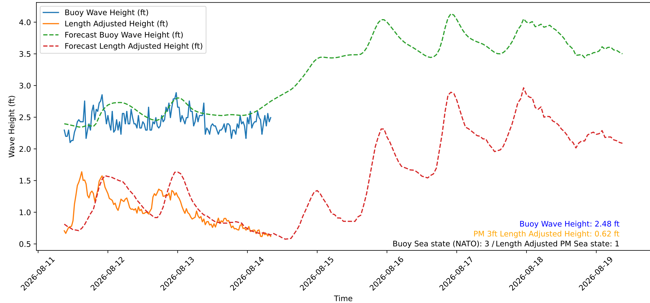
Wave Heights over Time for Red Beach at 2026-08-14 08:50:47
