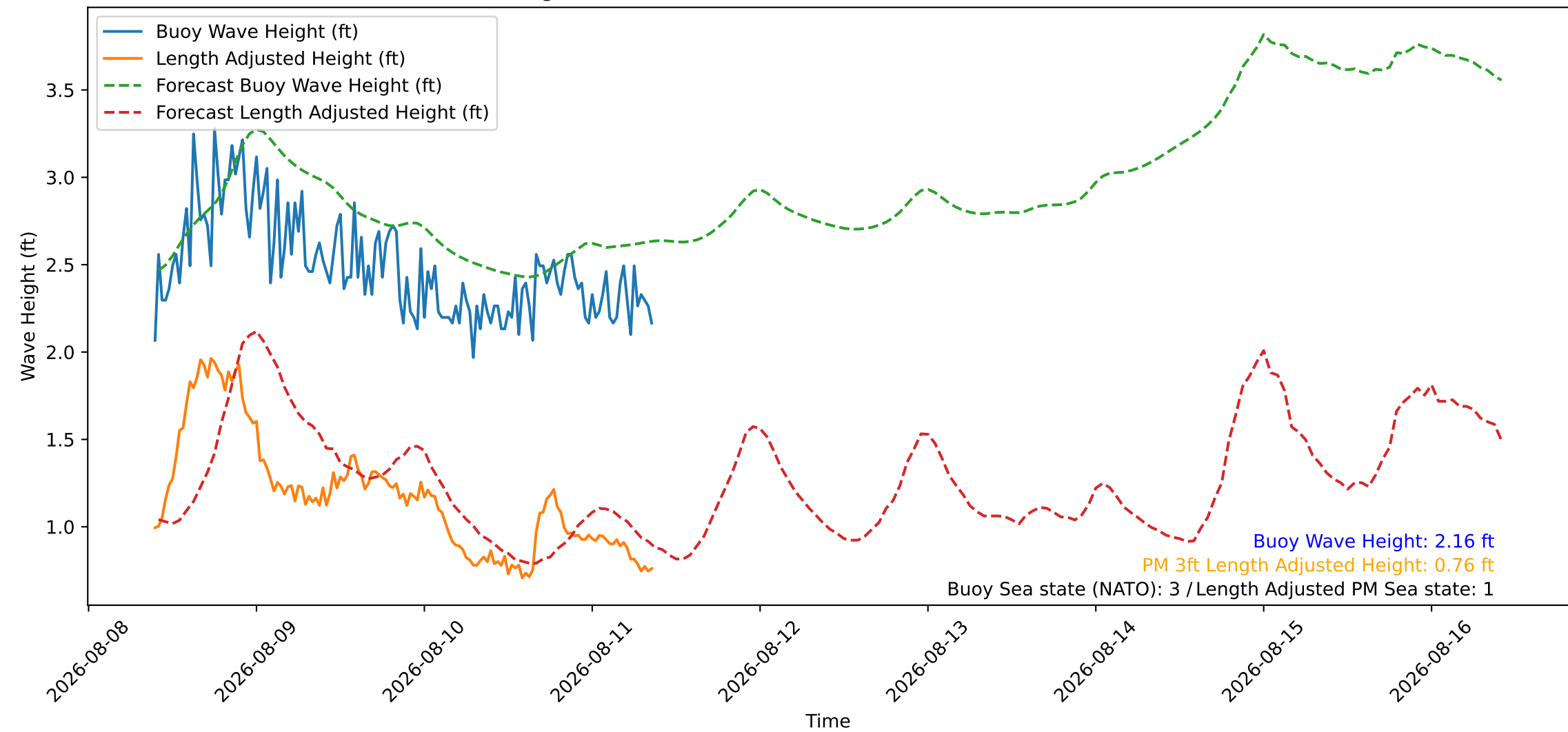
Wave Heights over Time for Oceanside Harbor at 2026-08-11 09:30:27
