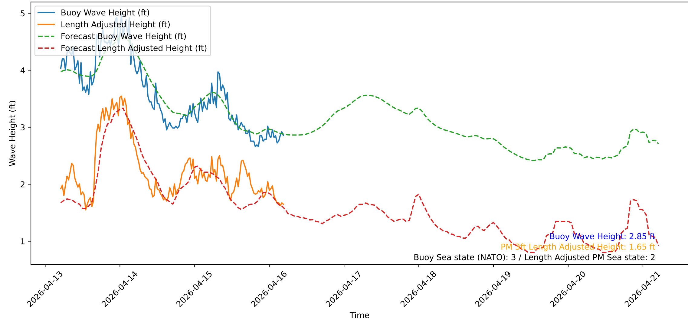
Wave Heights over Time for Green Beach at 2026-04-16 05:11:12
