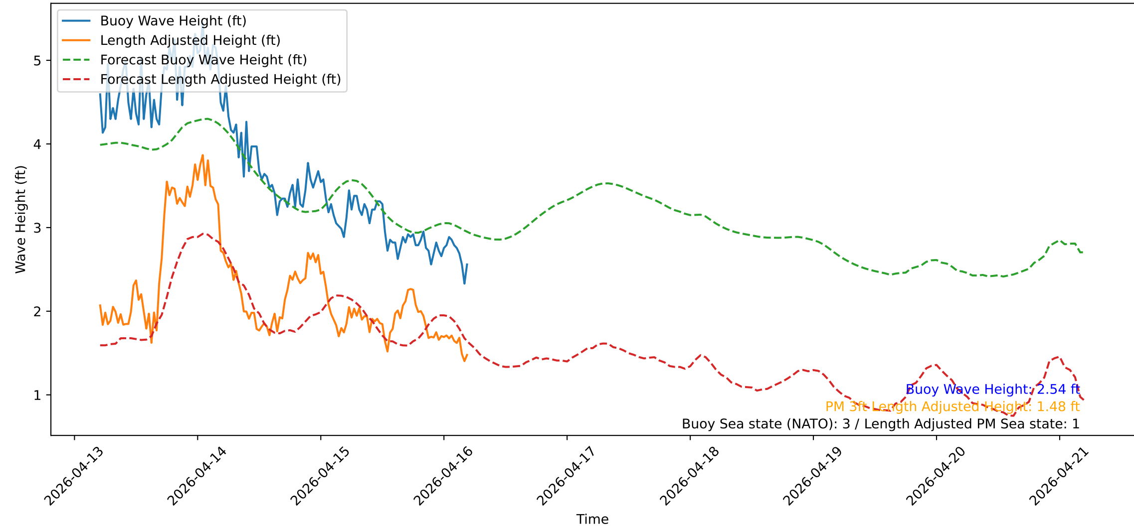
Wave Heights over Time for Oceanside Harbor at 2026-04-16 05:10:31
