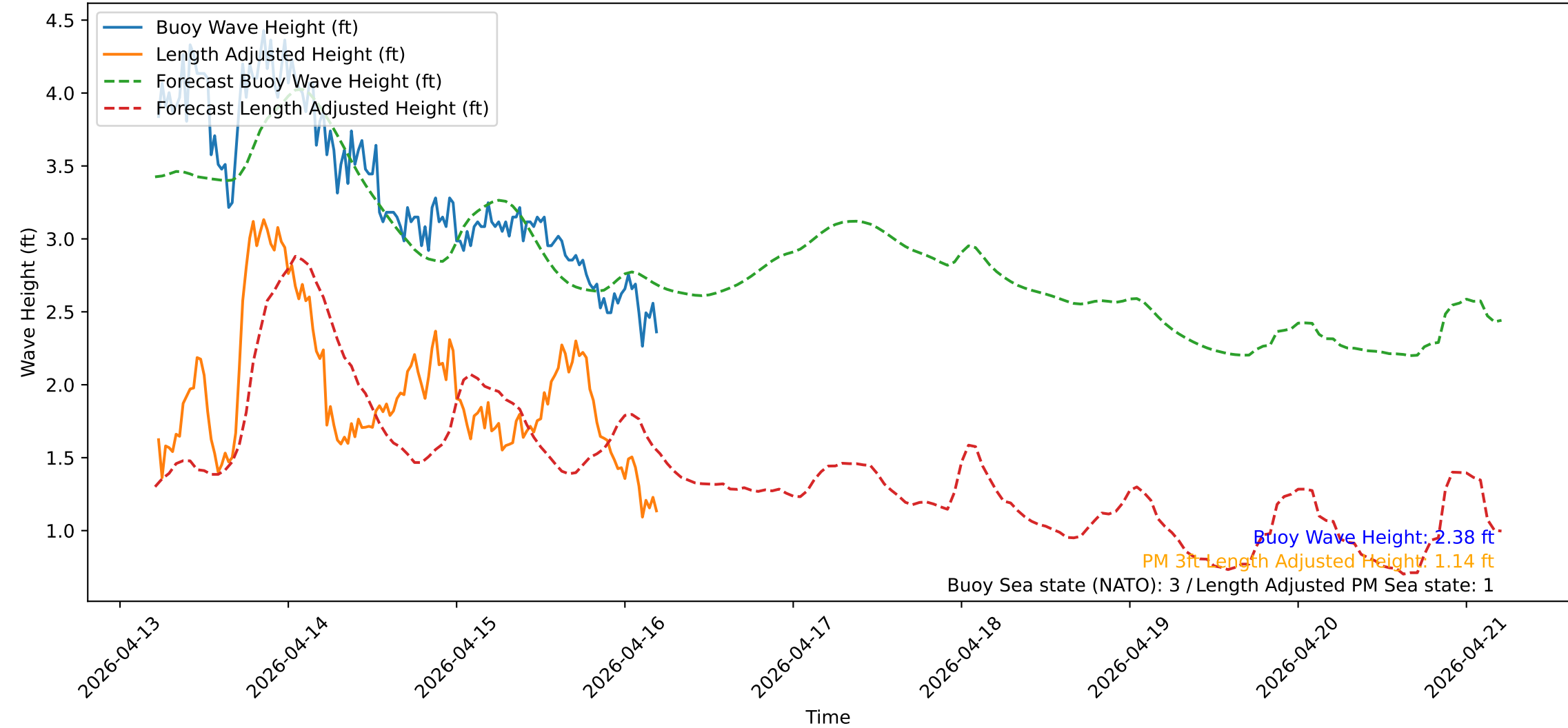
Wave Heights over Time for Red Beach at 2026-04-16 05:10:50
