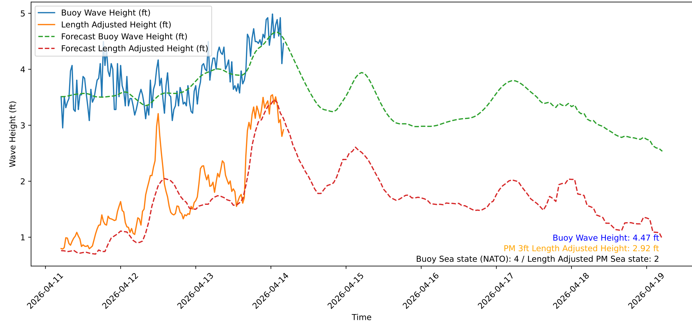
Wave Heights over Time for Green Beach at 2026-04-14 04:51:13
