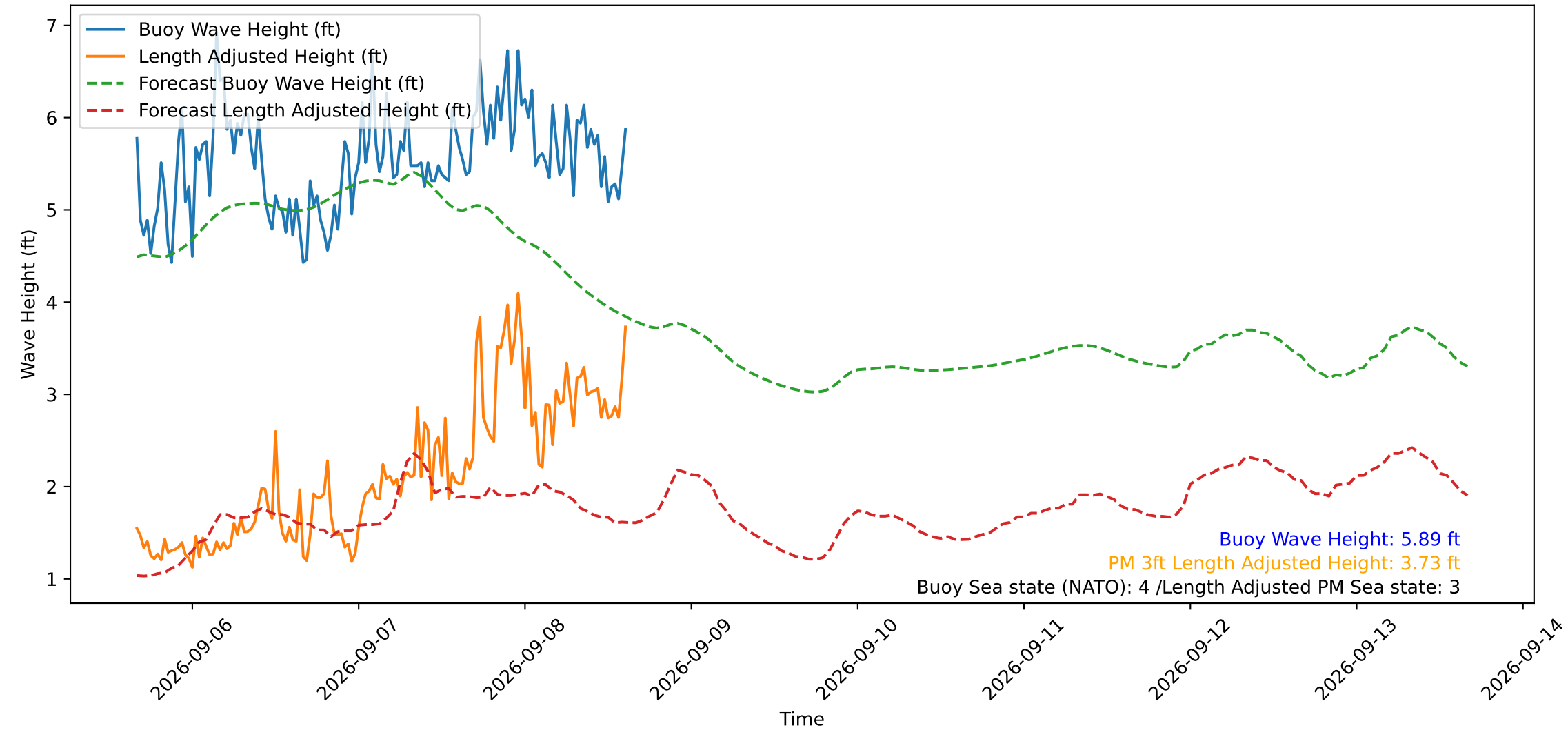
Wave Heights over Time for Red Beach at 2026-09-08 15:30:49
