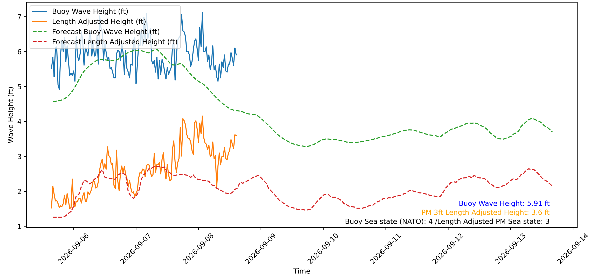
Wave Heights over Time for Oceanside Harbor at 2026-09-08 15:30:29
