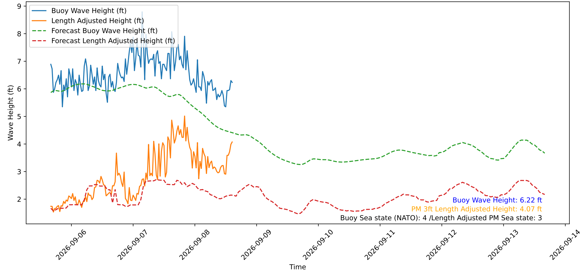
Wave Heights over Time for Green Beach at 2026-09-08 15:31:12
