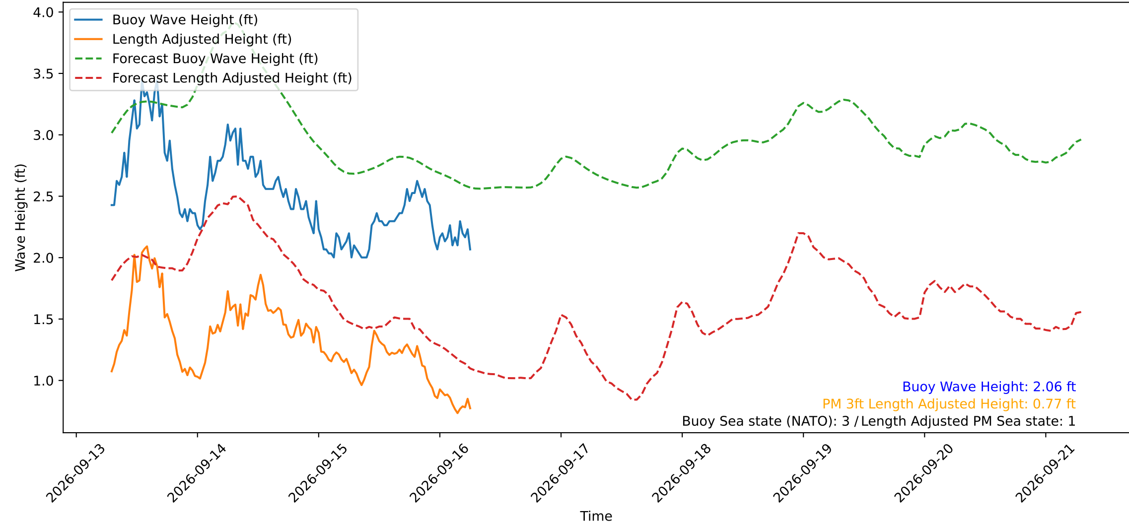
Wave Heights over Time for Red Beach at 2026-09-16 06:40:48
