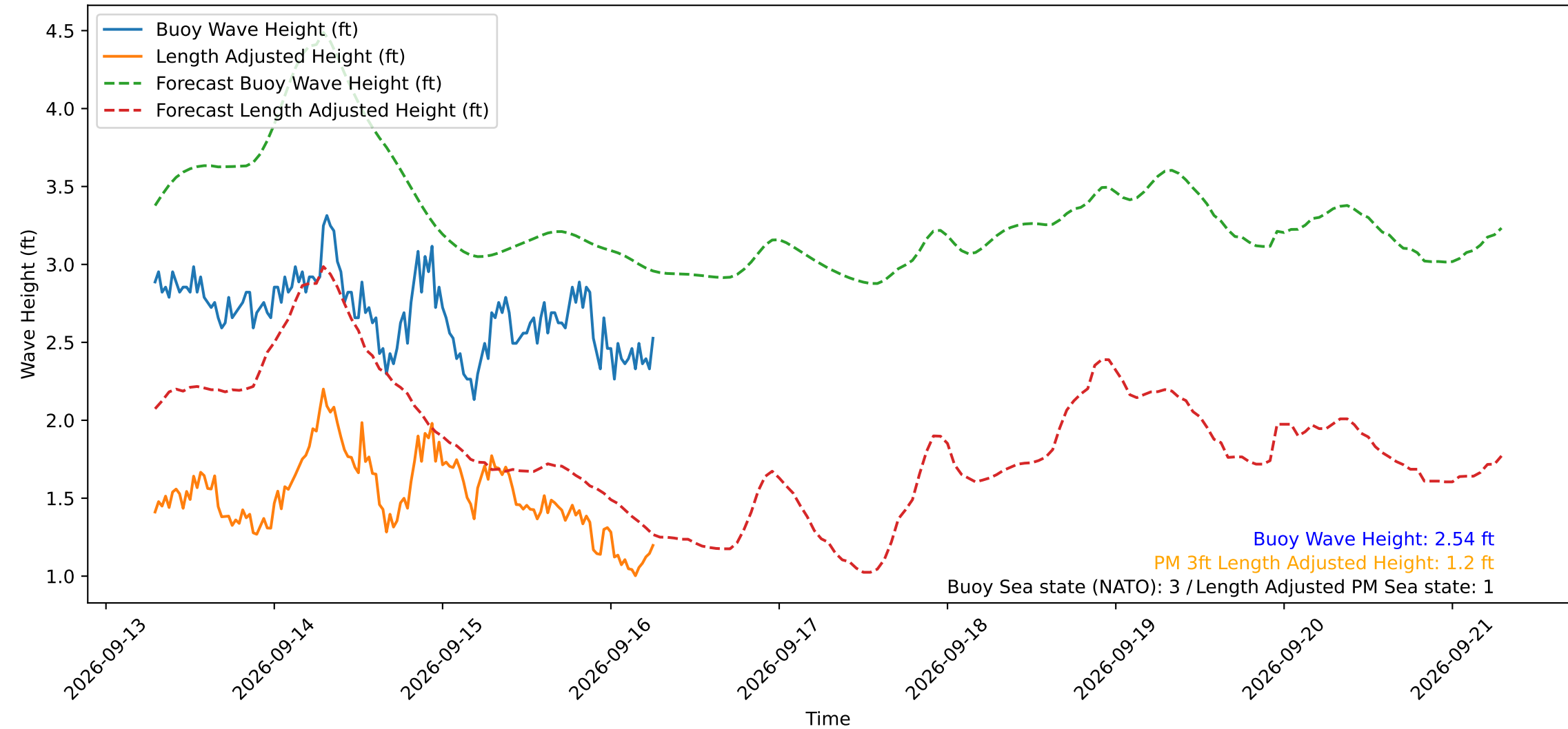
Wave Heights over Time for Green Beach at 2026-09-16 06:41:11
