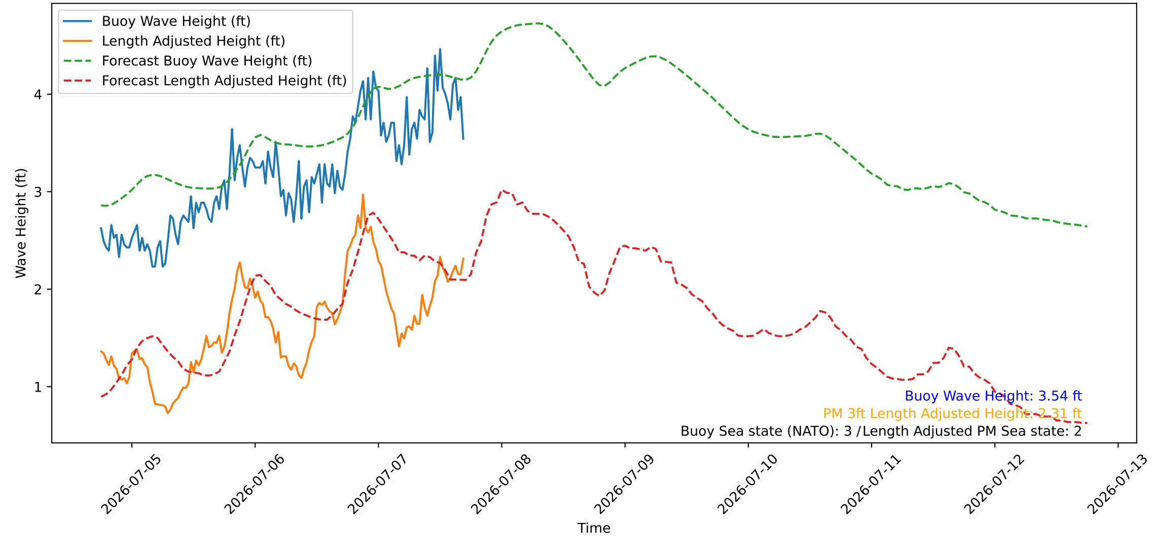
Wave Heights over Time for Red Beach at 2026-07-07 17:50:48
