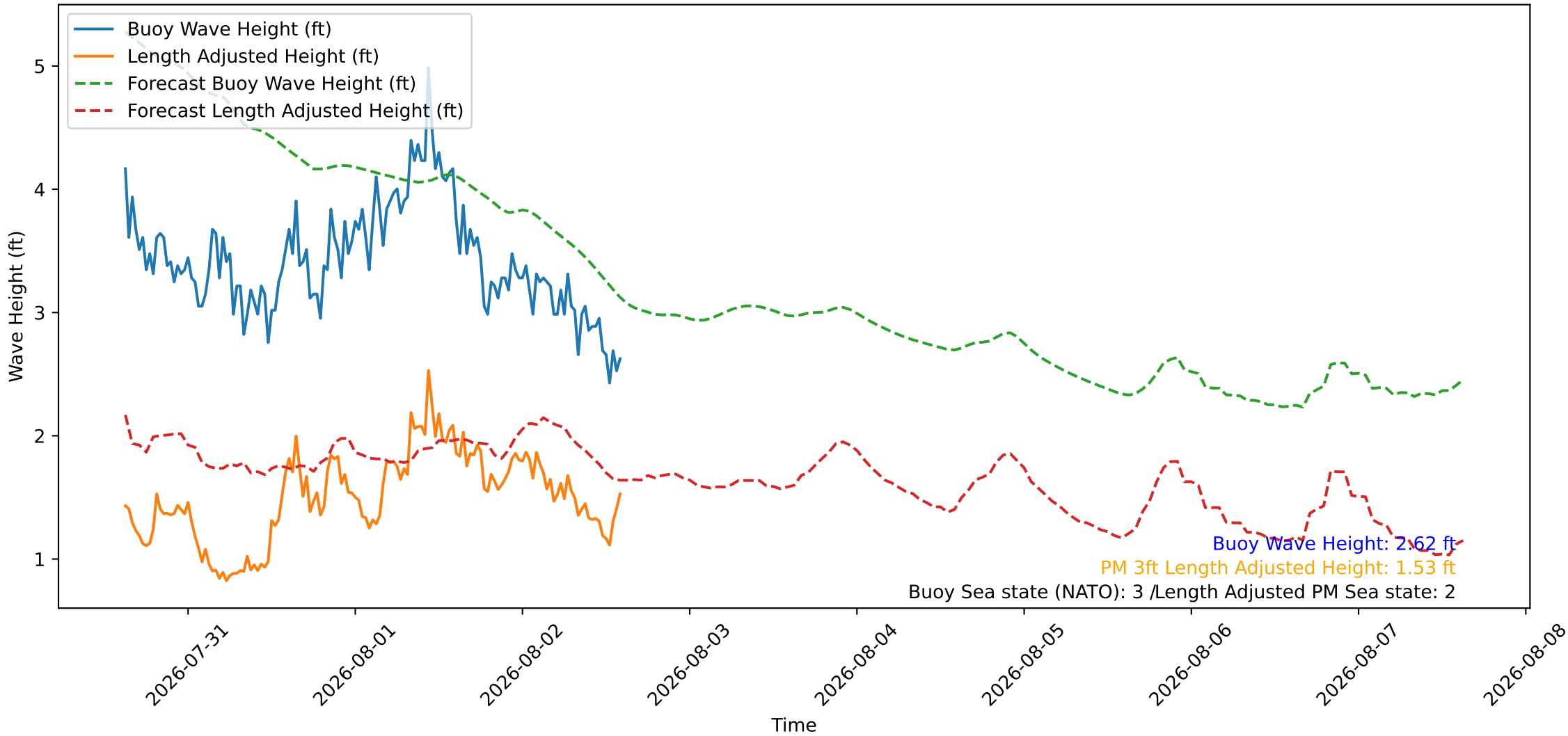
Wave Heights over Time for Green Beach at 2026-08-02 14:51:09
