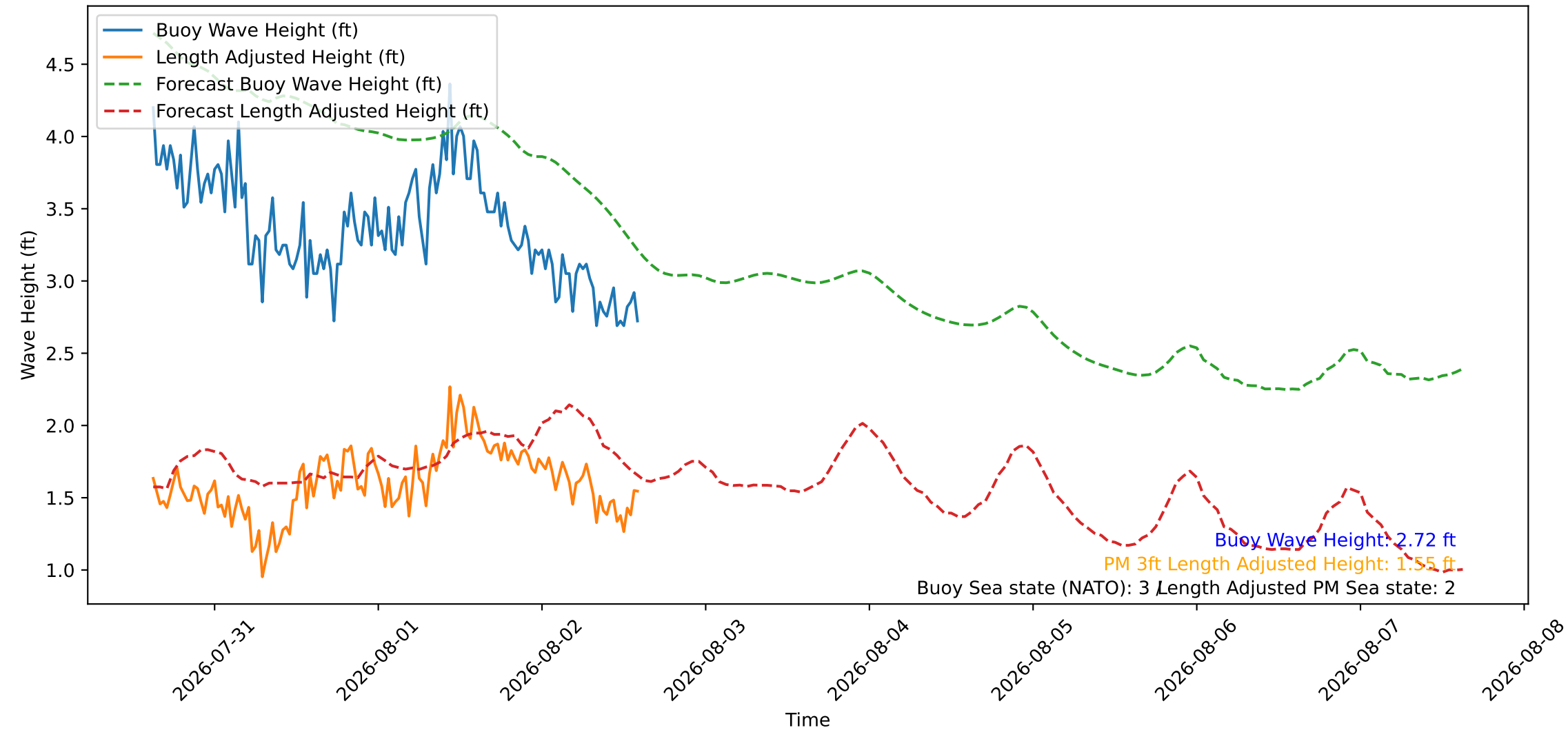
Wave Heights over Time for Oceanside Harbor at 2026-08-02 14:50:26
