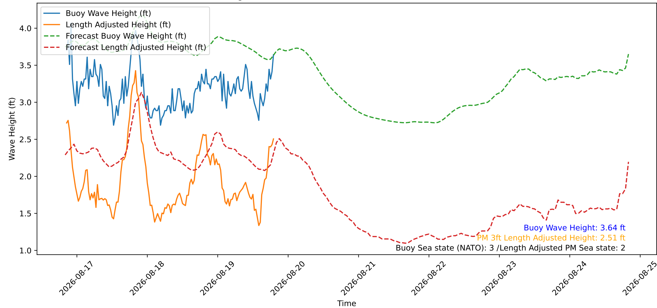
Wave Heights over Time for Green Beach at 2026-08-19 20:01:08
