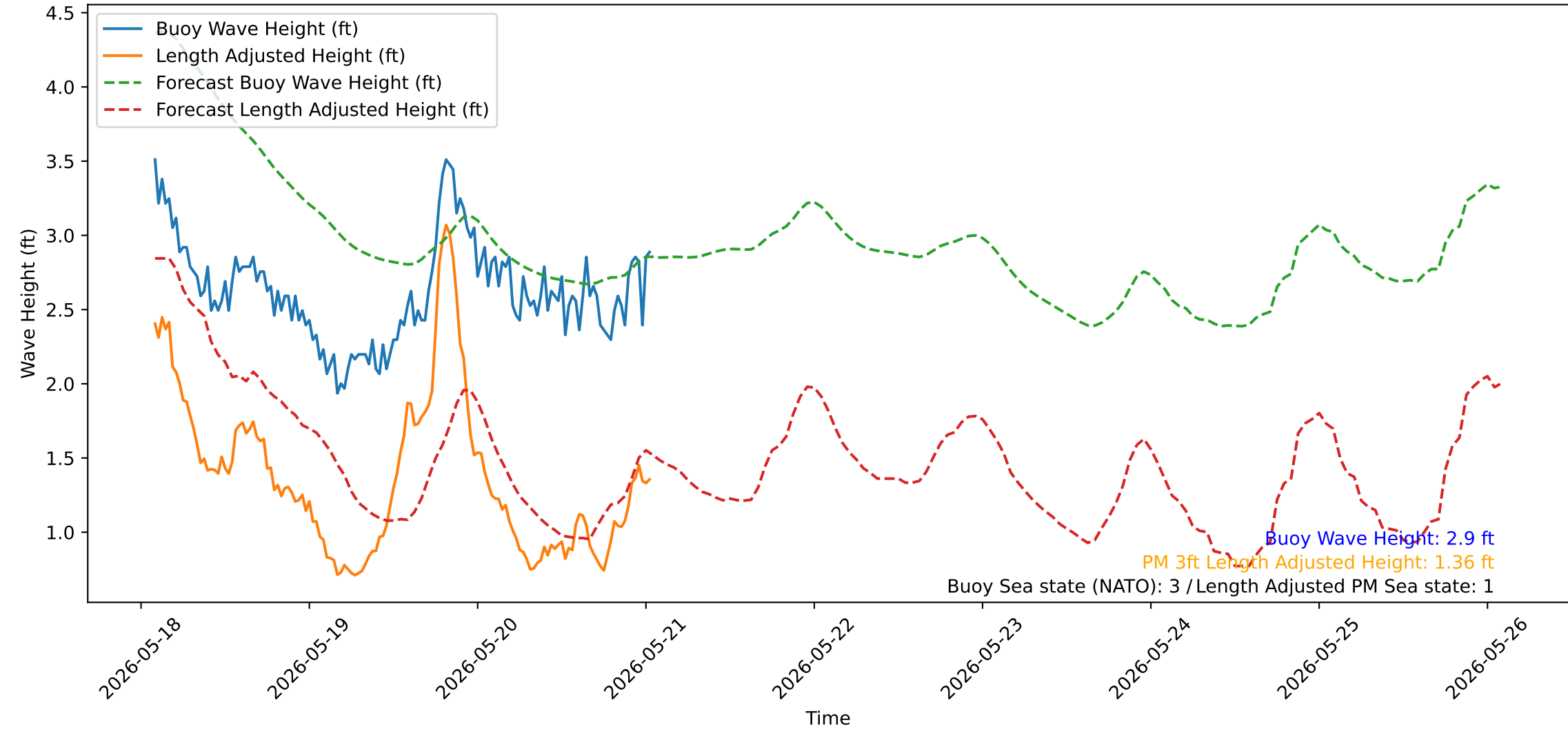
Wave Heights over Time for Red Beach at 2026-05-21 01:30:50
