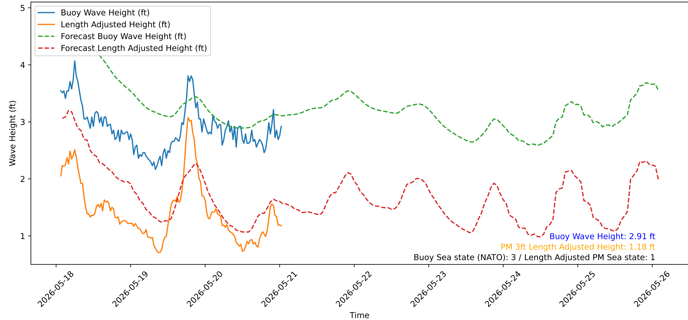
Wave Heights over Time for Green Beach at 2026-05-21 01:31:12
