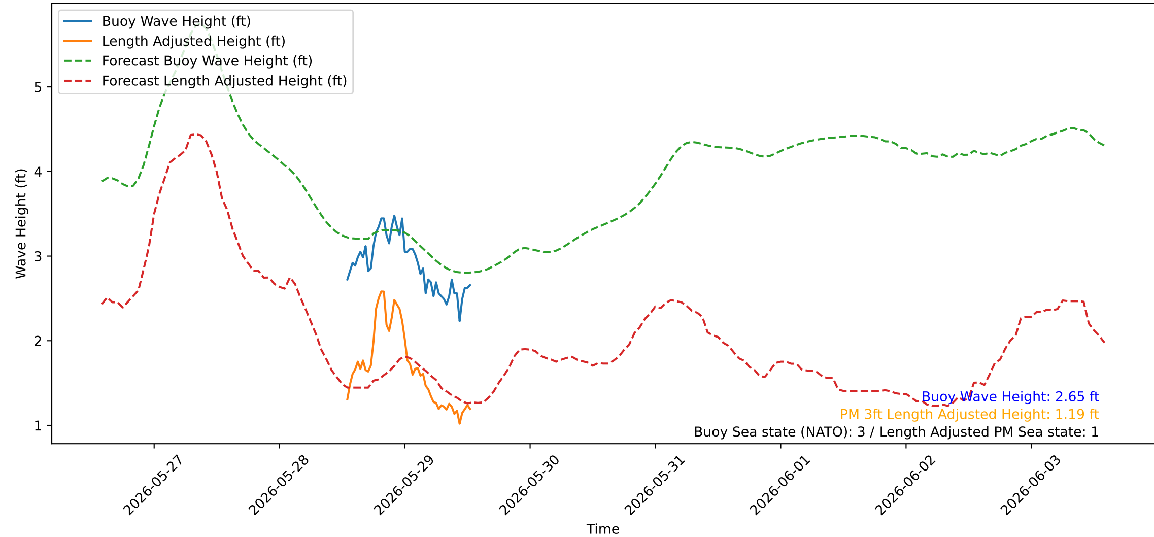
Wave Heights over Time for Oceanside Harbor at 2026-05-29 13:30:21
