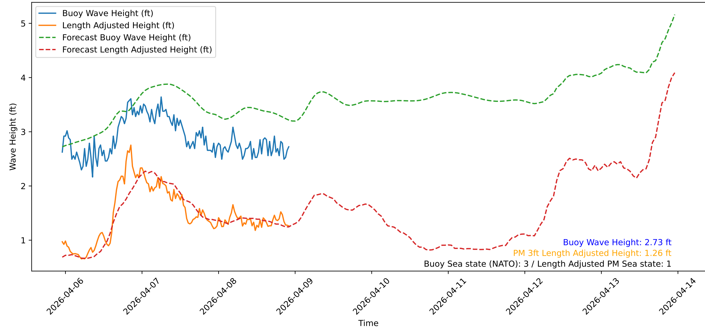
Wave Heights over Time for Oceanside Harbor at 2026-04-08 23:00:31
