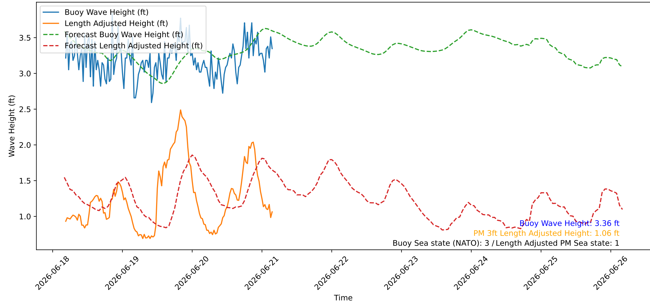
Wave Heights over Time for Red Beach at 2026-06-21 04:20:46
