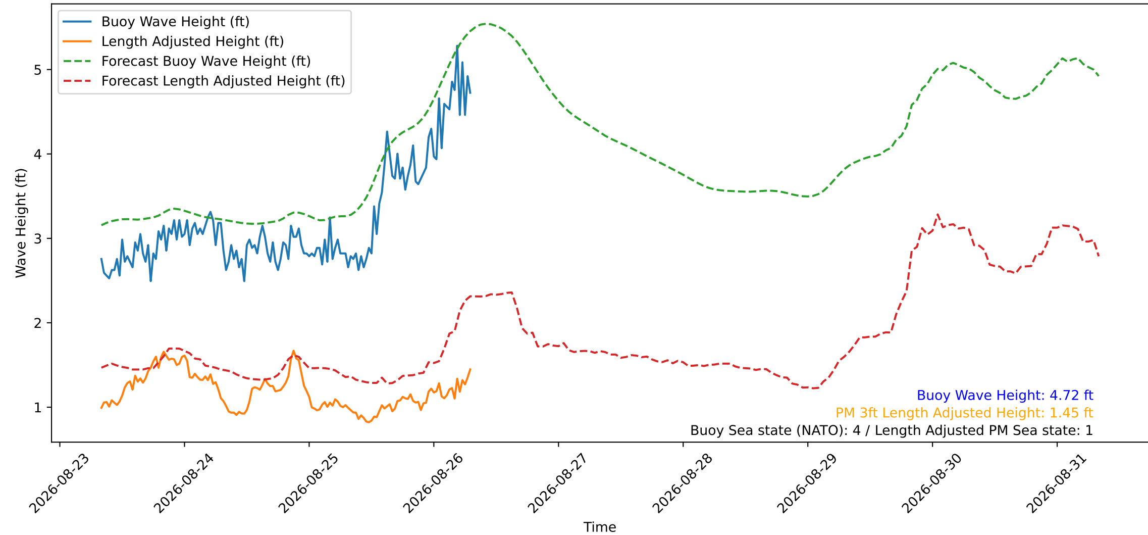
Wave Heights over Time for Green Beach at 2026-08-26 07:51:20
