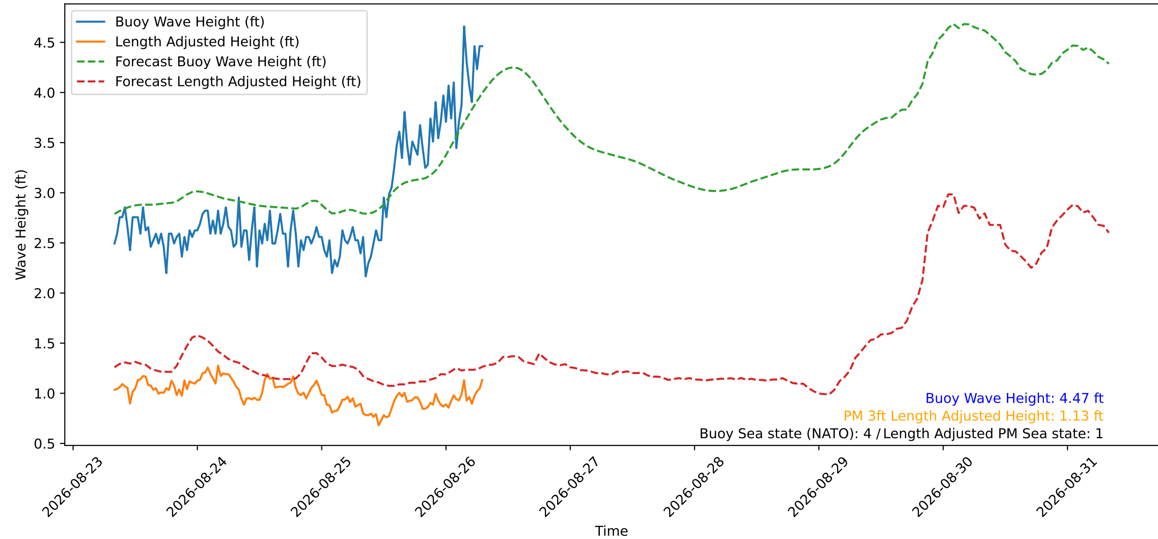
Wave Heights over Time for Red Beach at 2026-08-26 07:50:54
