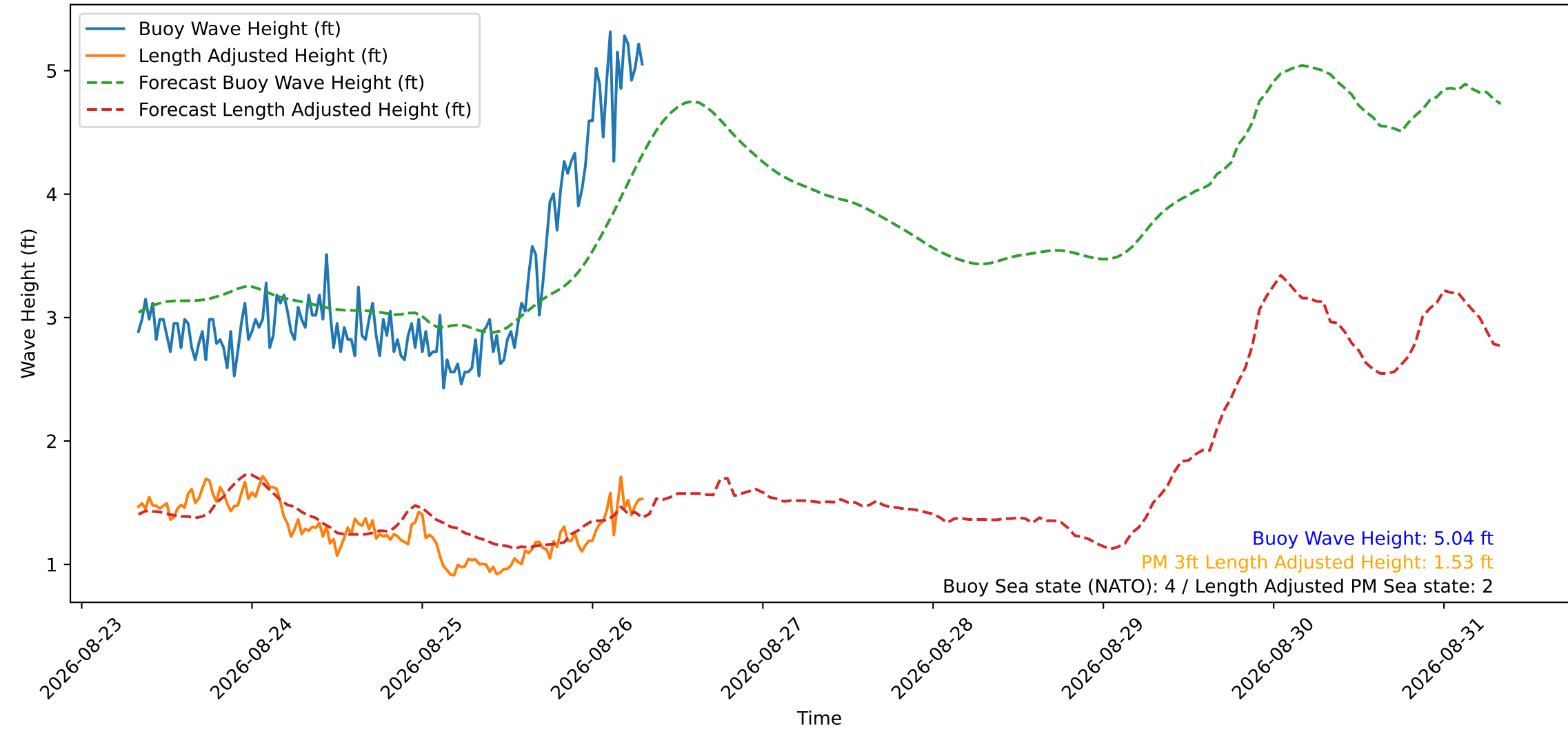
Wave Heights over Time for Oceanside Harbor at 2026-08-26 07:50:31
