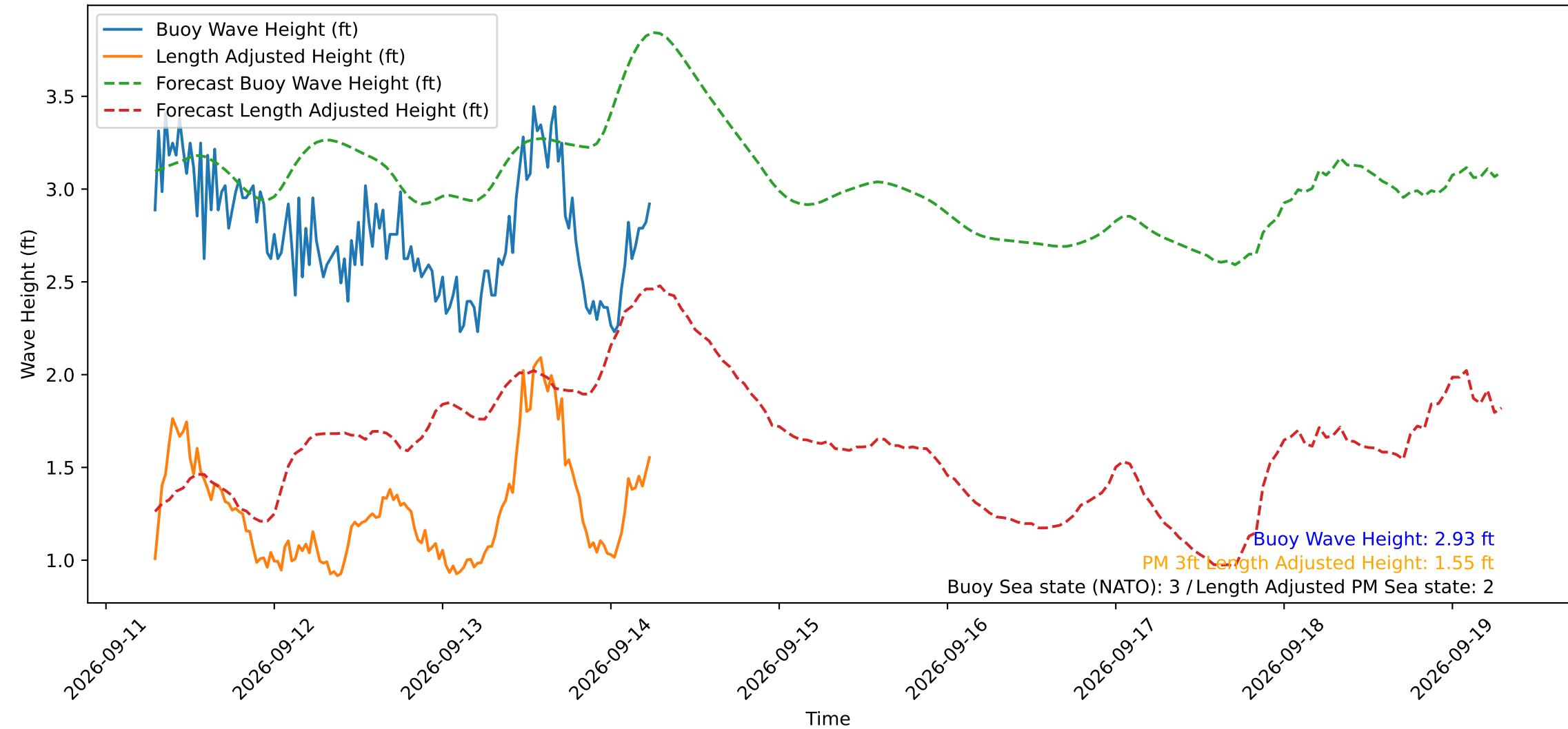
Wave Heights over Time for Red Beach at 2026-09-14 06:30:49
