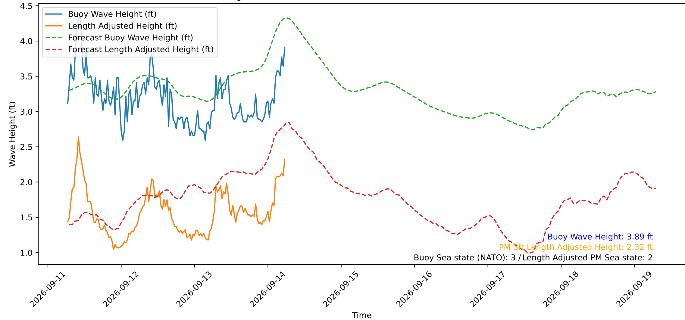
Wave Heights over Time for Oceanside Harbor at 2026-09-14 06:30:29
