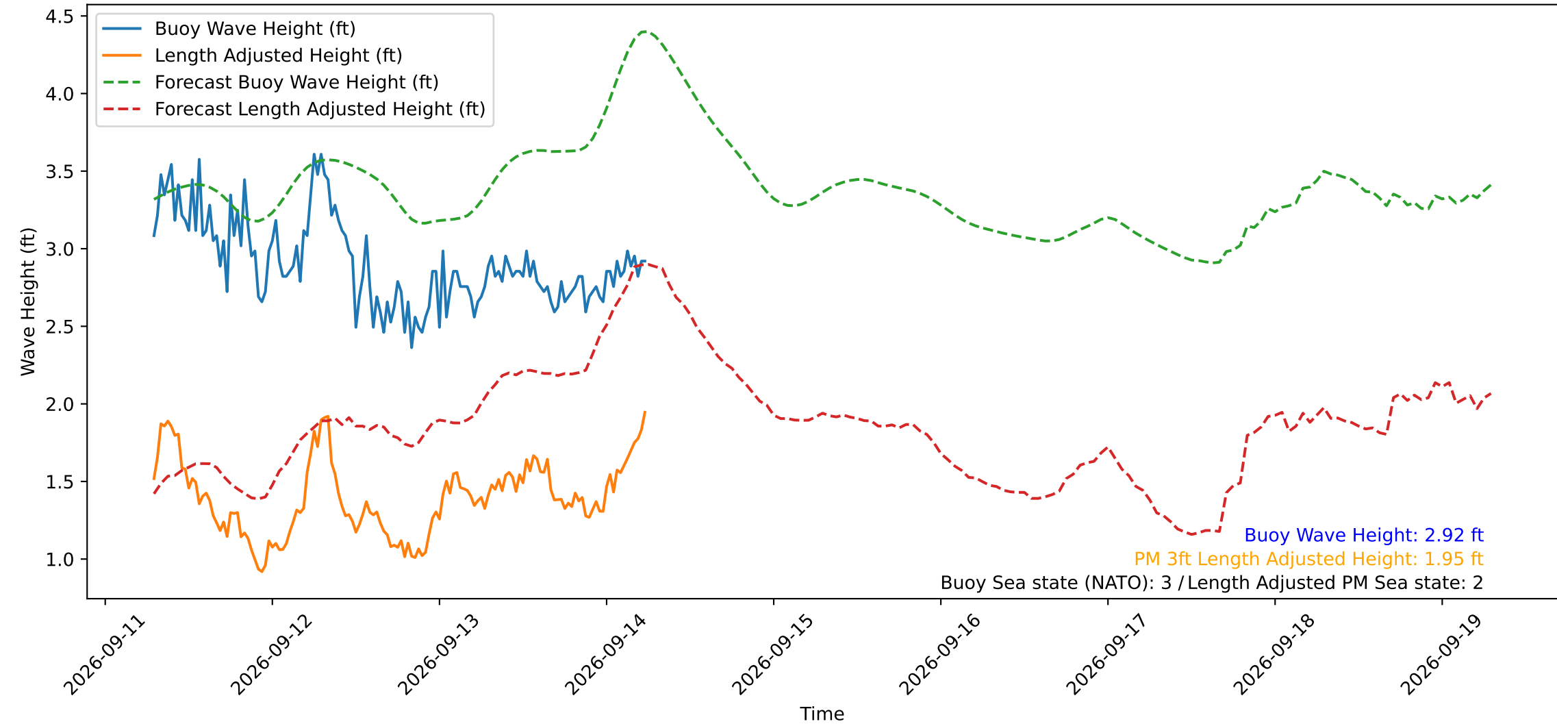
Wave Heights over Time for Green Beach at 2026-09-14 06:31:11
