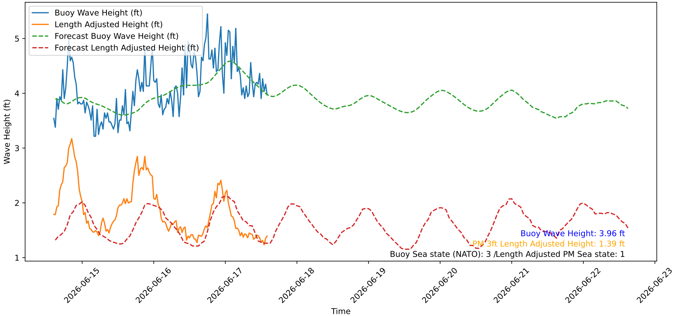
Wave Heights over Time for Oceanside Harbor at 2026-06-17 14:40:26
