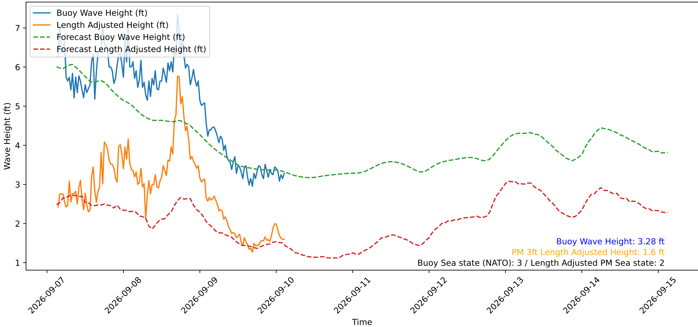
Wave Heights over Time for Oceanside Harbor at 2026-09-10 03:20:29
