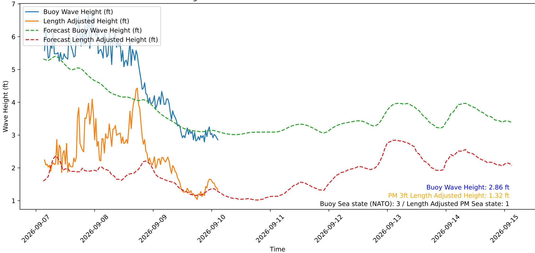
Wave Heights over Time for Red Beach at 2026-09-10 03:20:50
