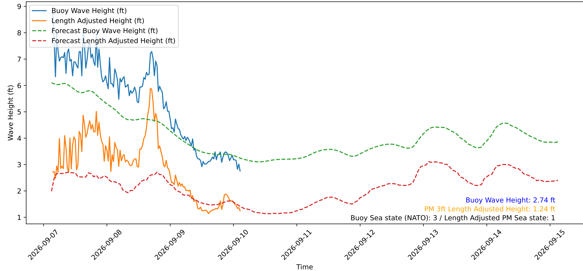
Wave Heights over Time for Green Beach at 2026-09-10 03:21:13
