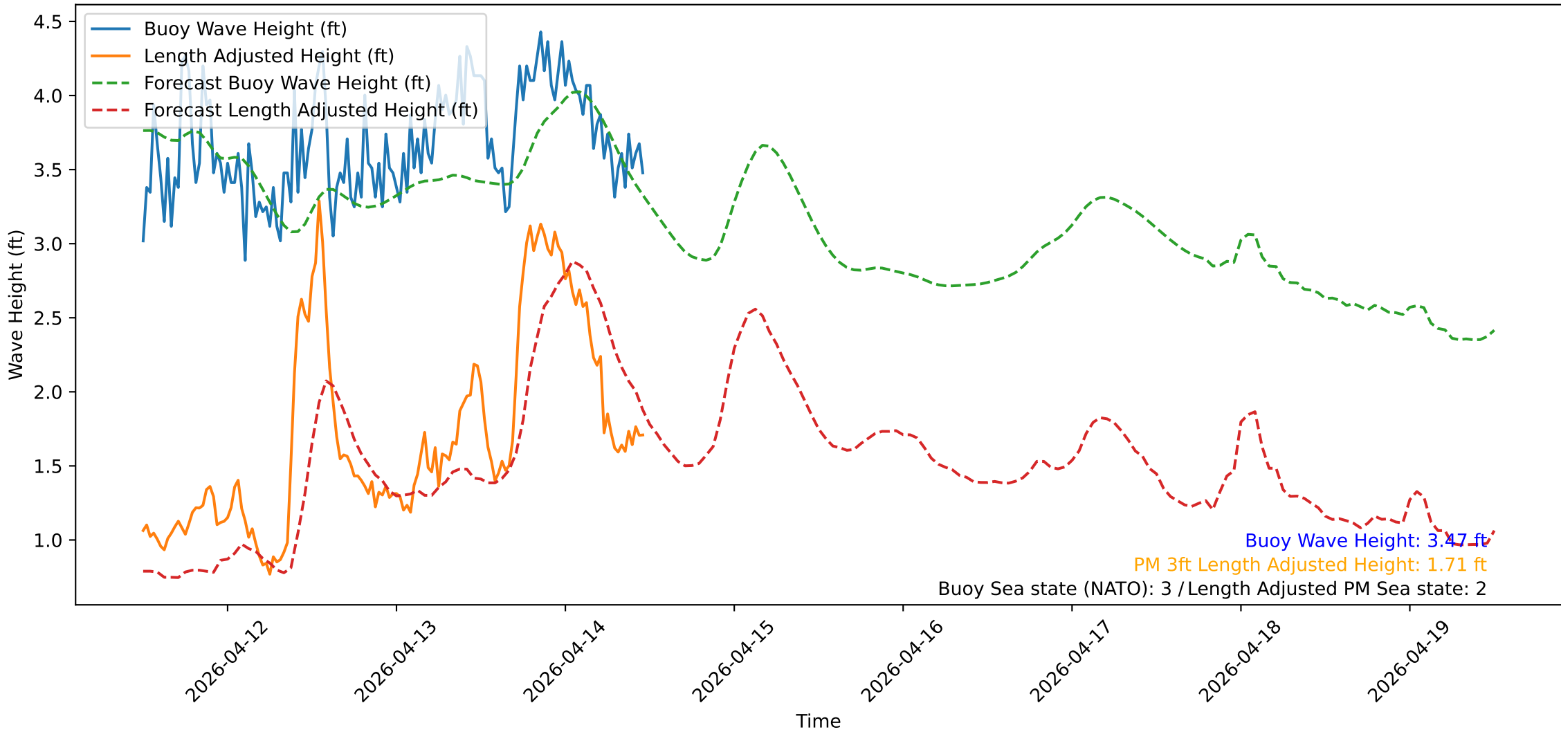
Wave Heights over Time for Red Beach at 2026-04-14 11:40:51
