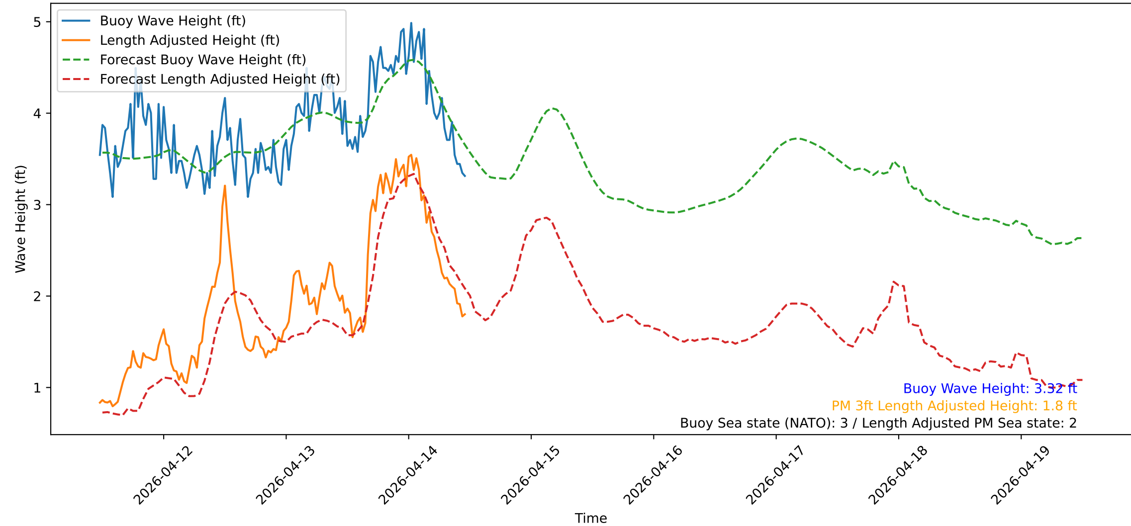
Wave Heights over Time for Green Beach at 2026-04-14 11:41:13
