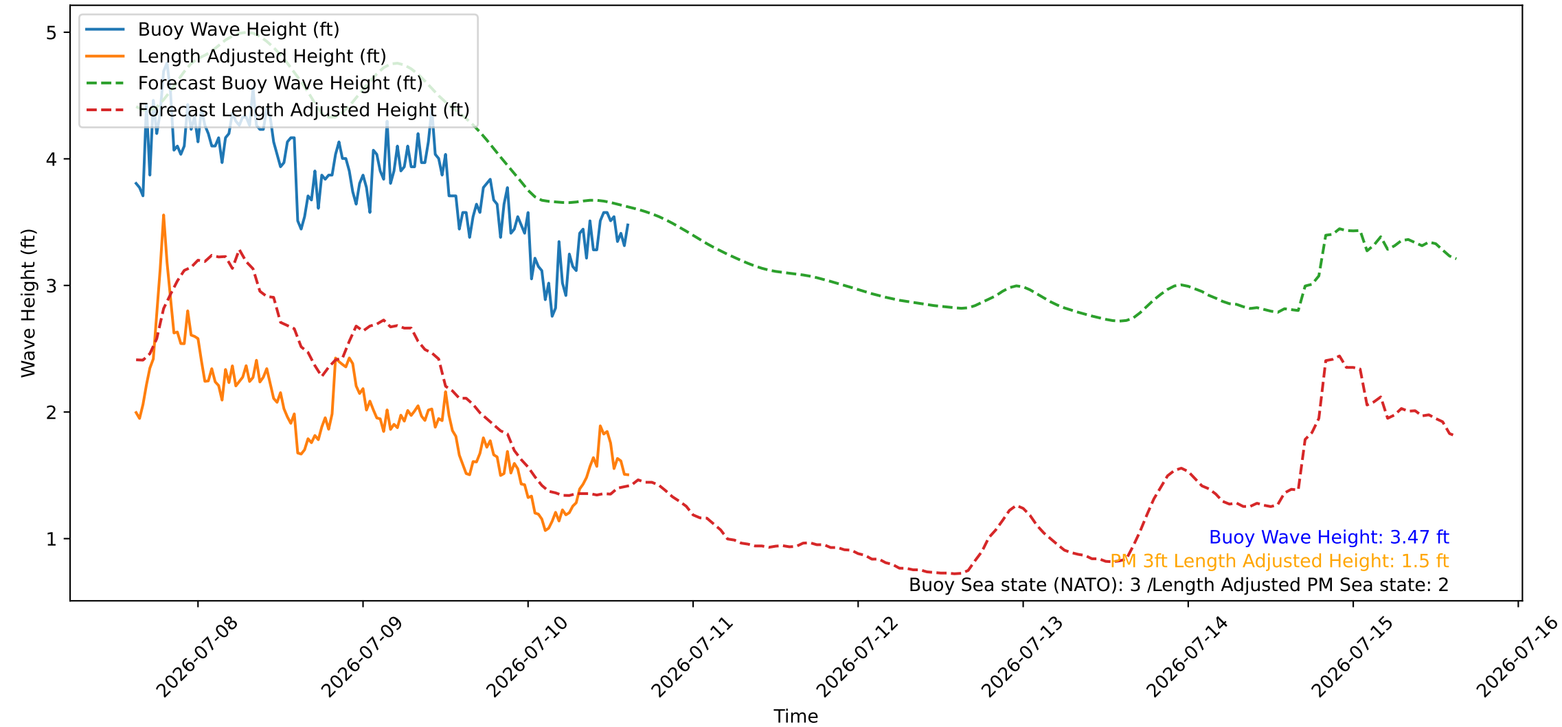
Wave Heights over Time for Green Beach at 2026-07-10 15:11:08
