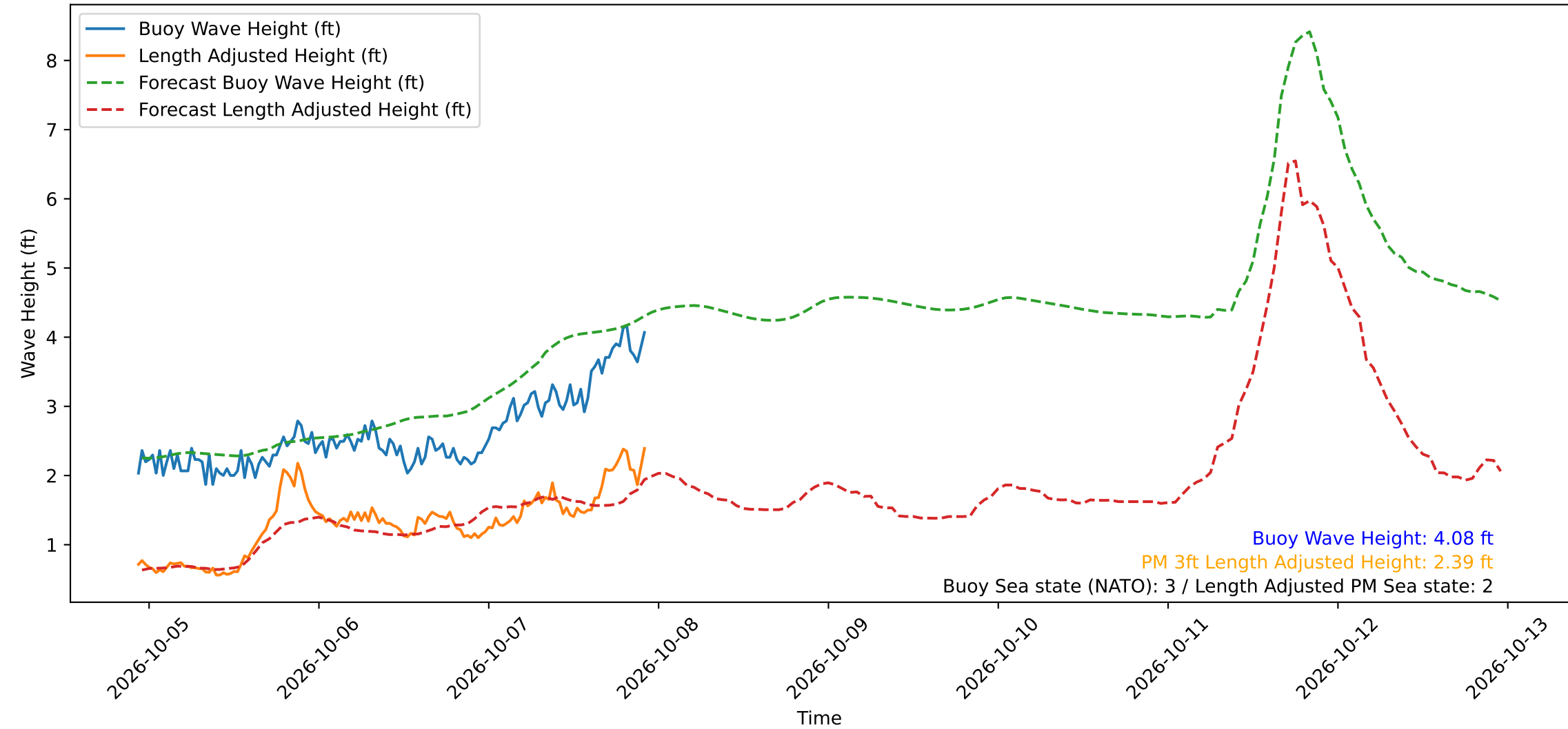
Wave Heights over Time for Oceanside Harbor at 2026-10-07 22:40:30
