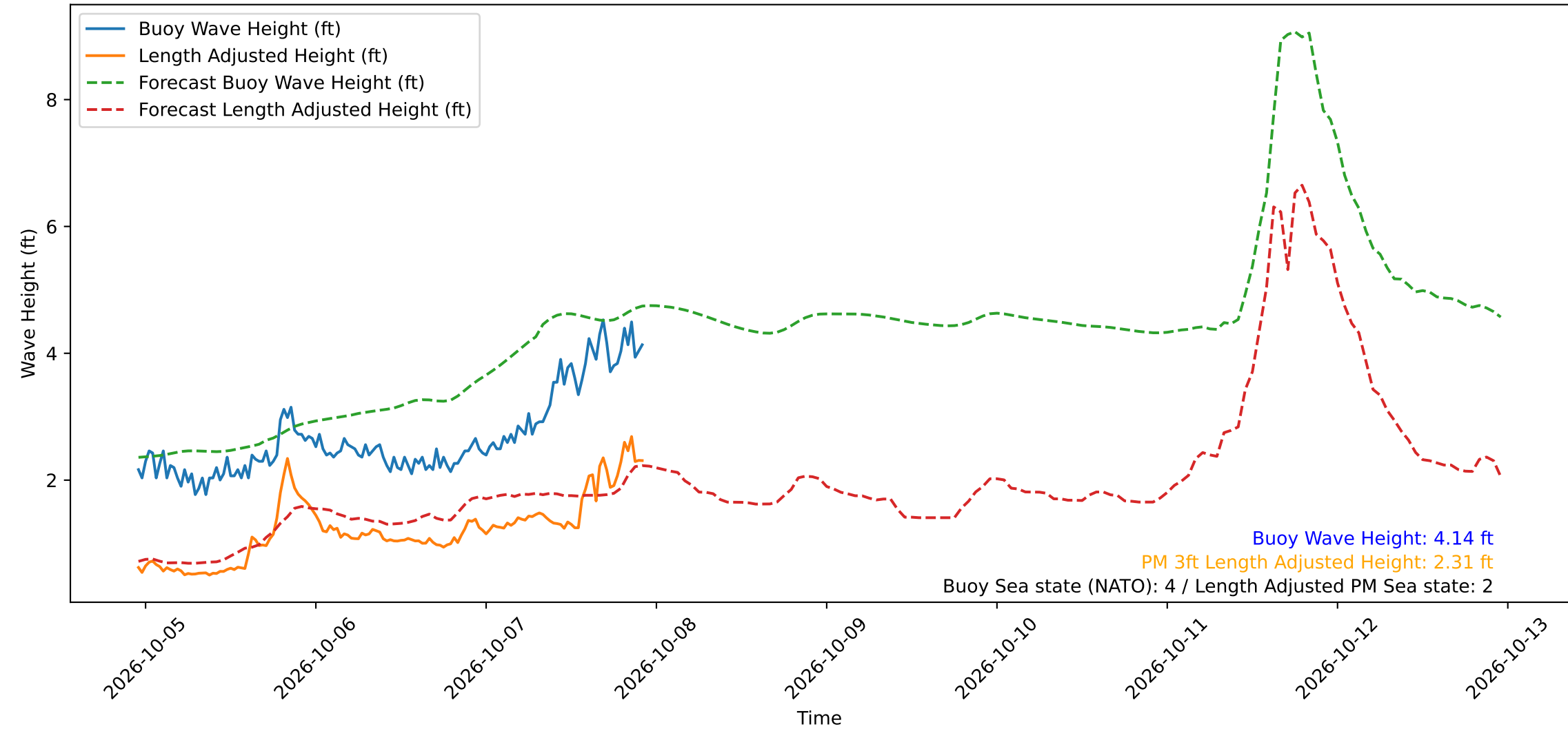
Wave Heights over Time for Green Beach at 2026-10-07 22:41:13
