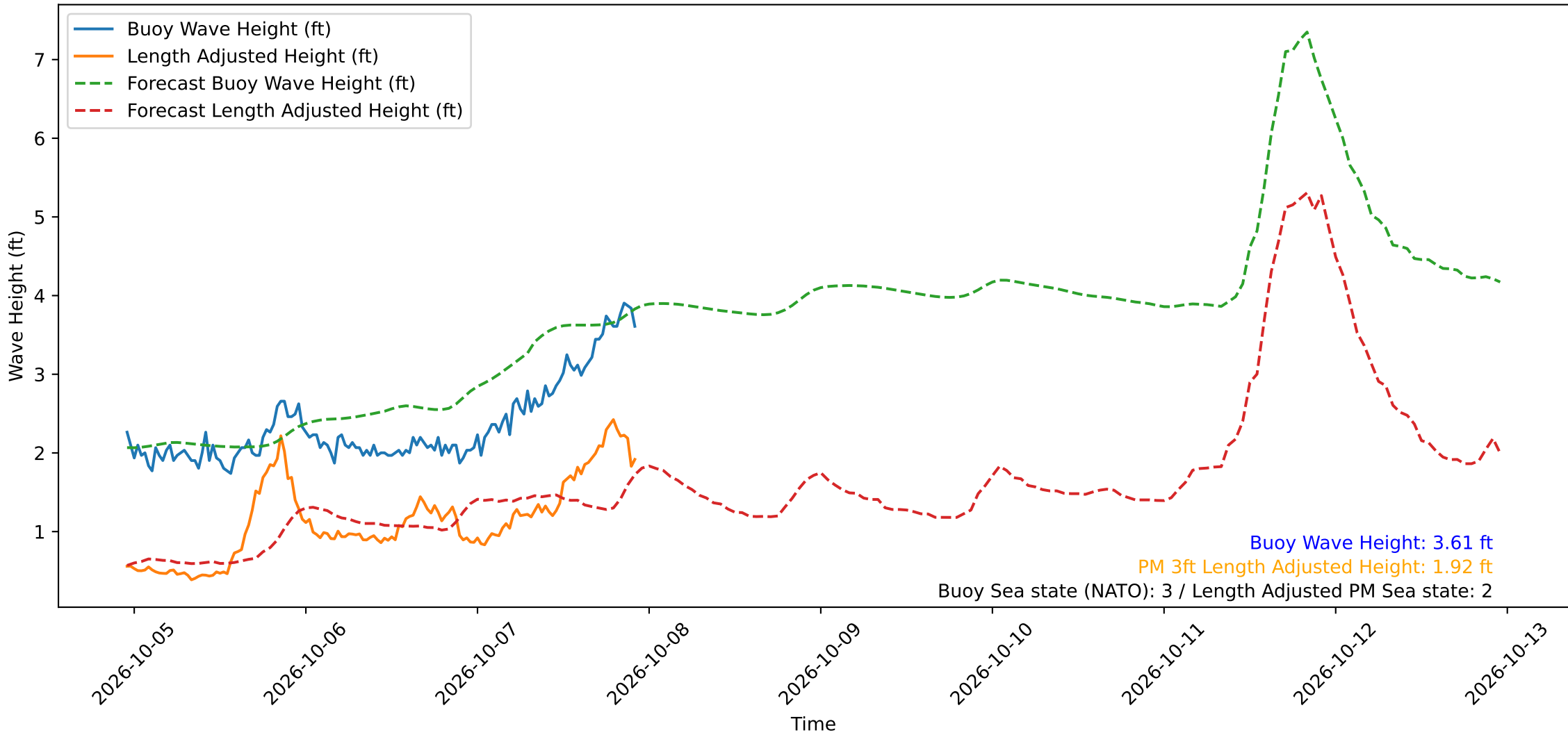
Wave Heights over Time for Red Beach at 2026-10-07 22:40:50
