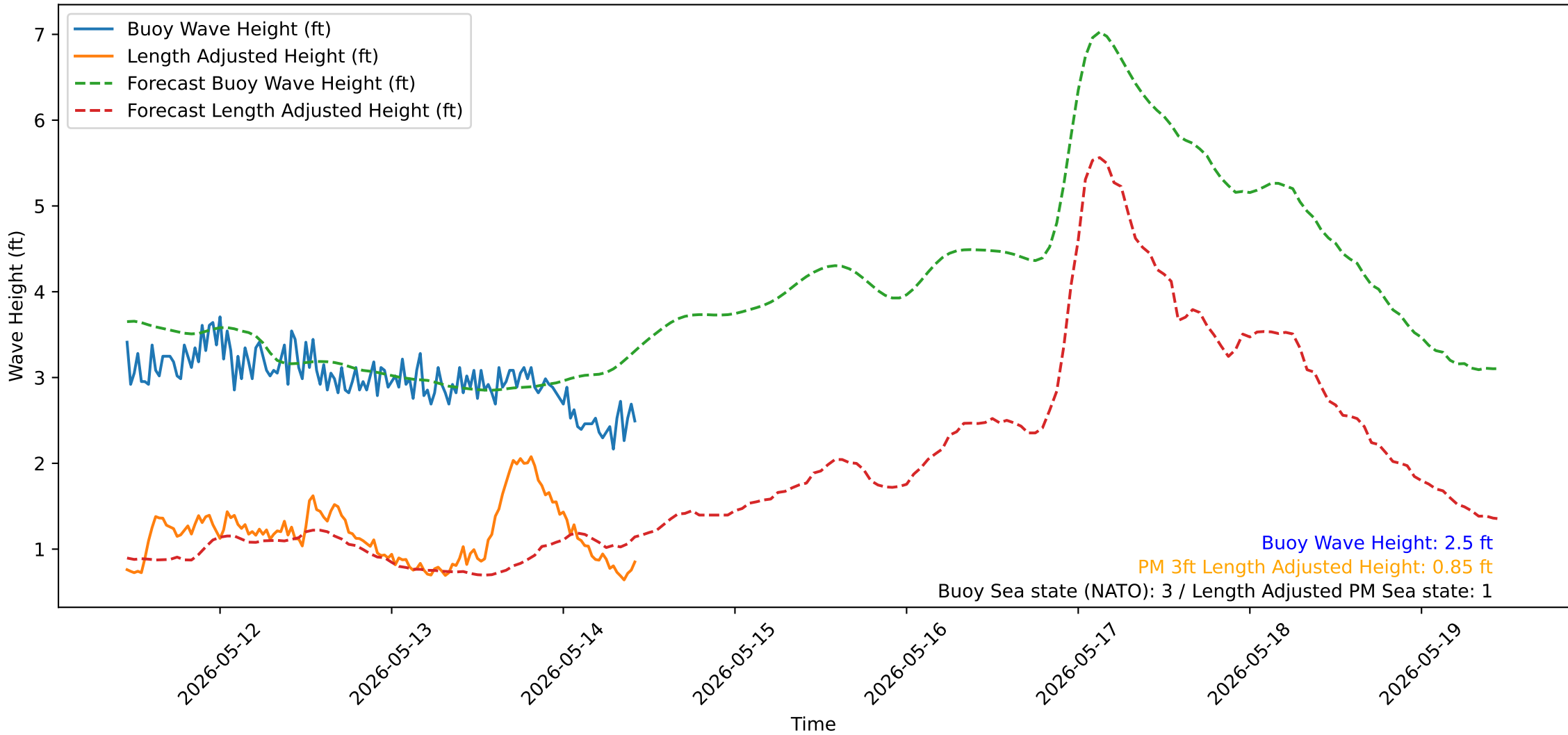
Wave Heights over Time for Oceanside Harbor at 2026-05-14 11:00:31
