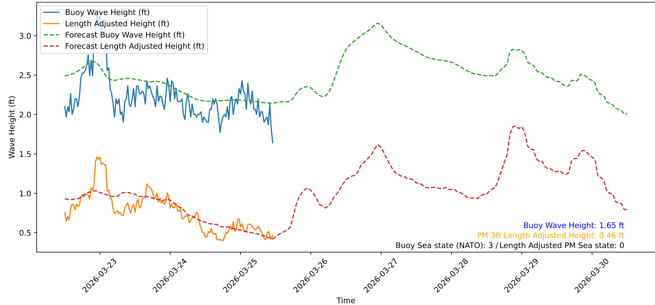
Wave Heights over Time for Green Beach at 2026-03-25 12:01:09
