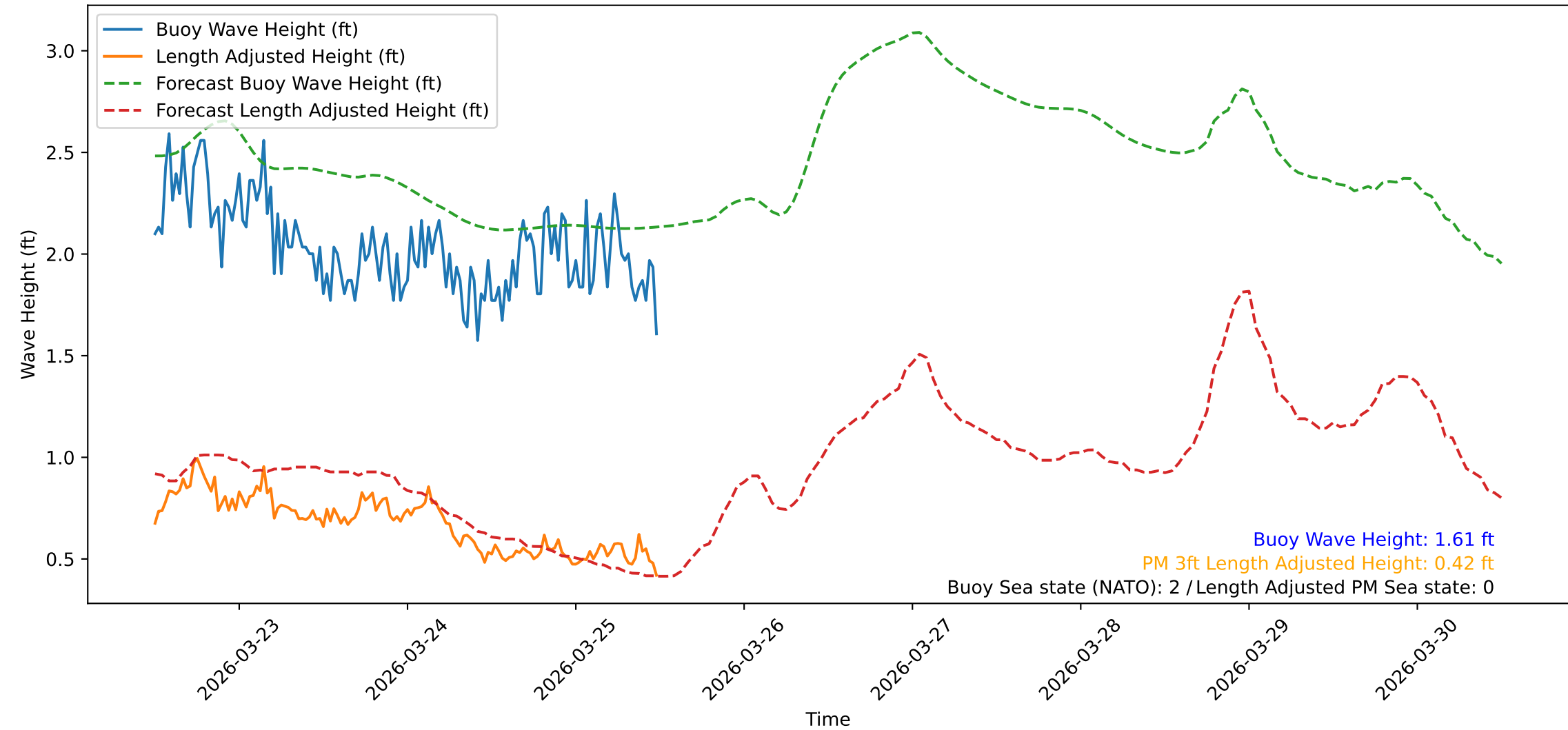
Wave Heights over Time for Oceanside Harbor at 2026-03-25 12:00:31
