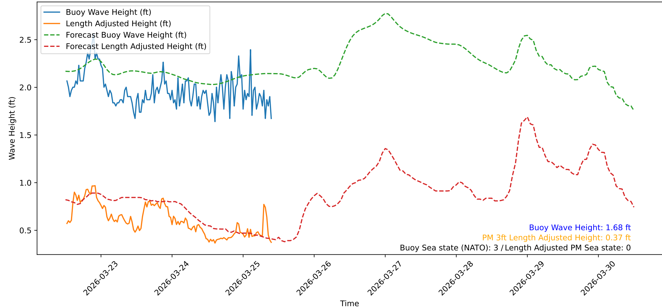
Wave Heights over Time for Red Beach at 2026-03-25 12:00:47
