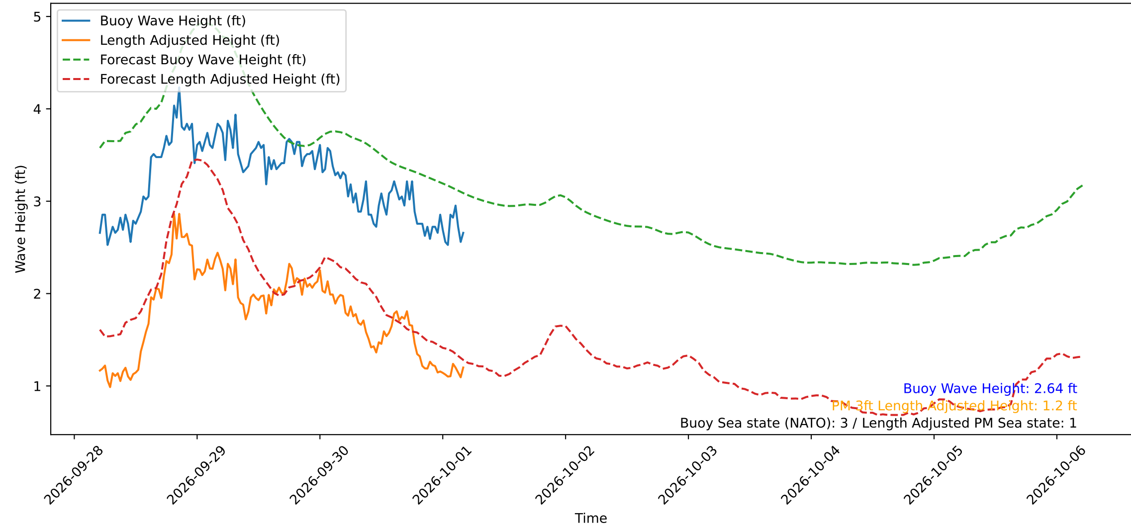
Wave Heights over Time for Oceanside Harbor at 2026-10-01 05:00:29
