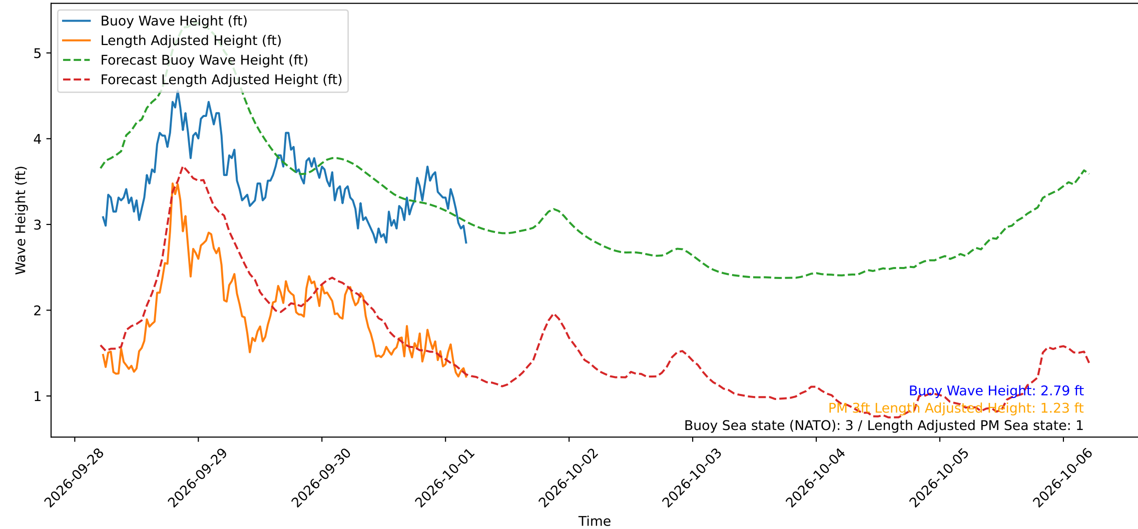
Wave Heights over Time for Green Beach at 2026-10-01 05:01:12
