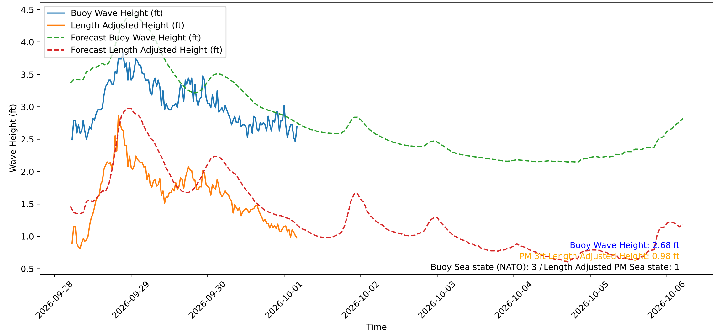
Wave Heights over Time for Red Beach at 2026-10-01 05:00:48
