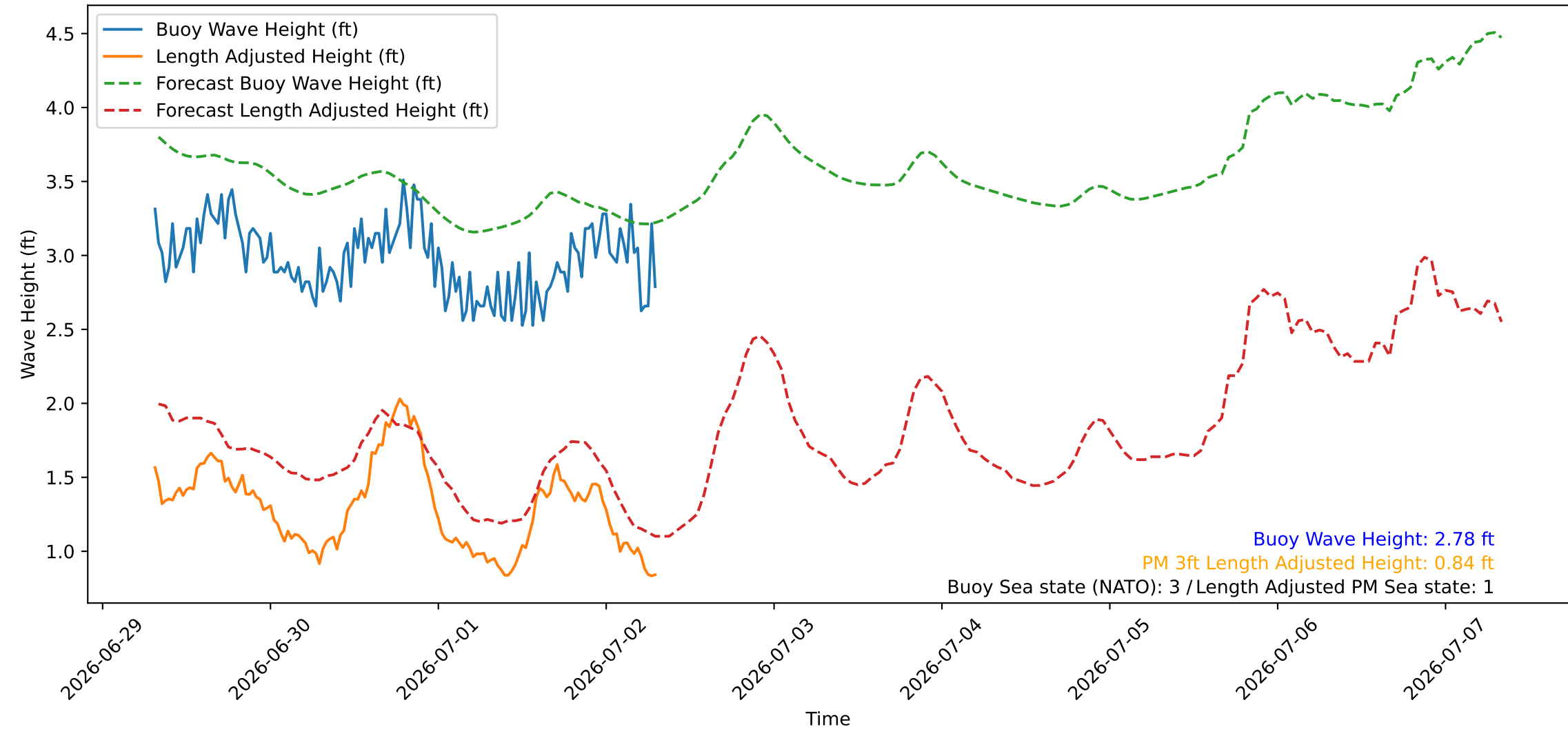
Wave Heights over Time for Green Beach at 2026-07-02 07:41:08
