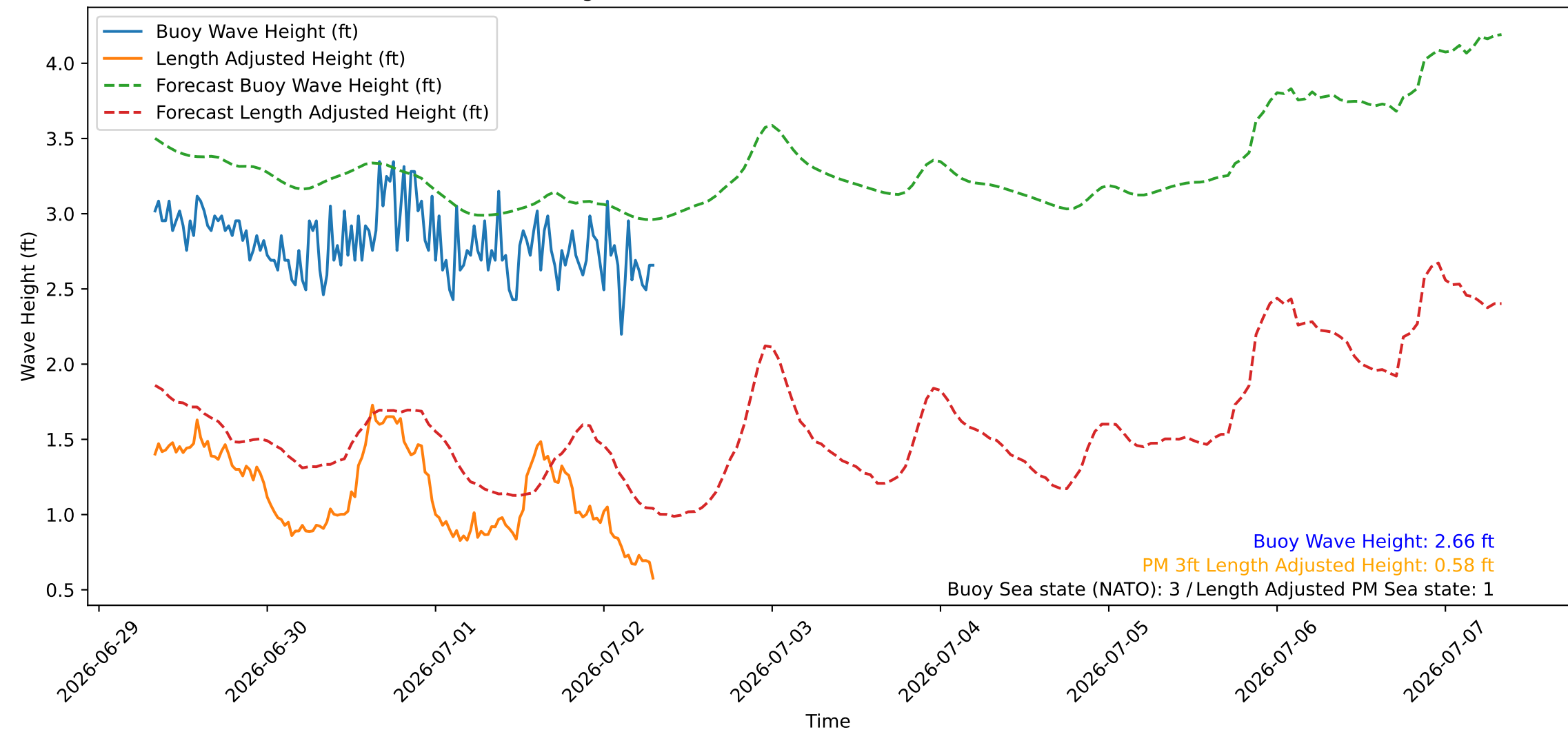
Wave Heights over Time for Red Beach at 2026-07-02 07:40:46
