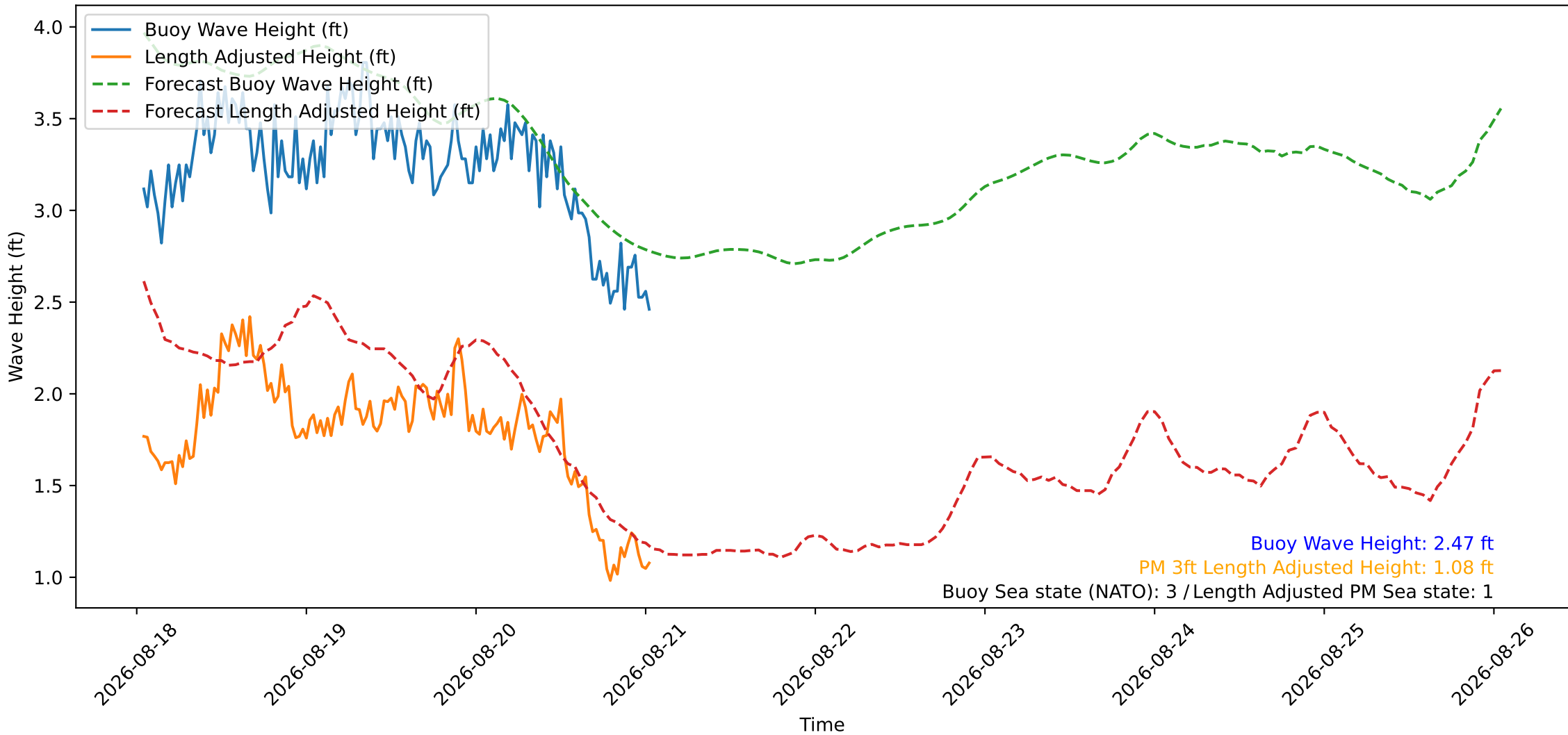
Wave Heights over Time for Oceanside Harbor at 2026-08-21 01:10:26
