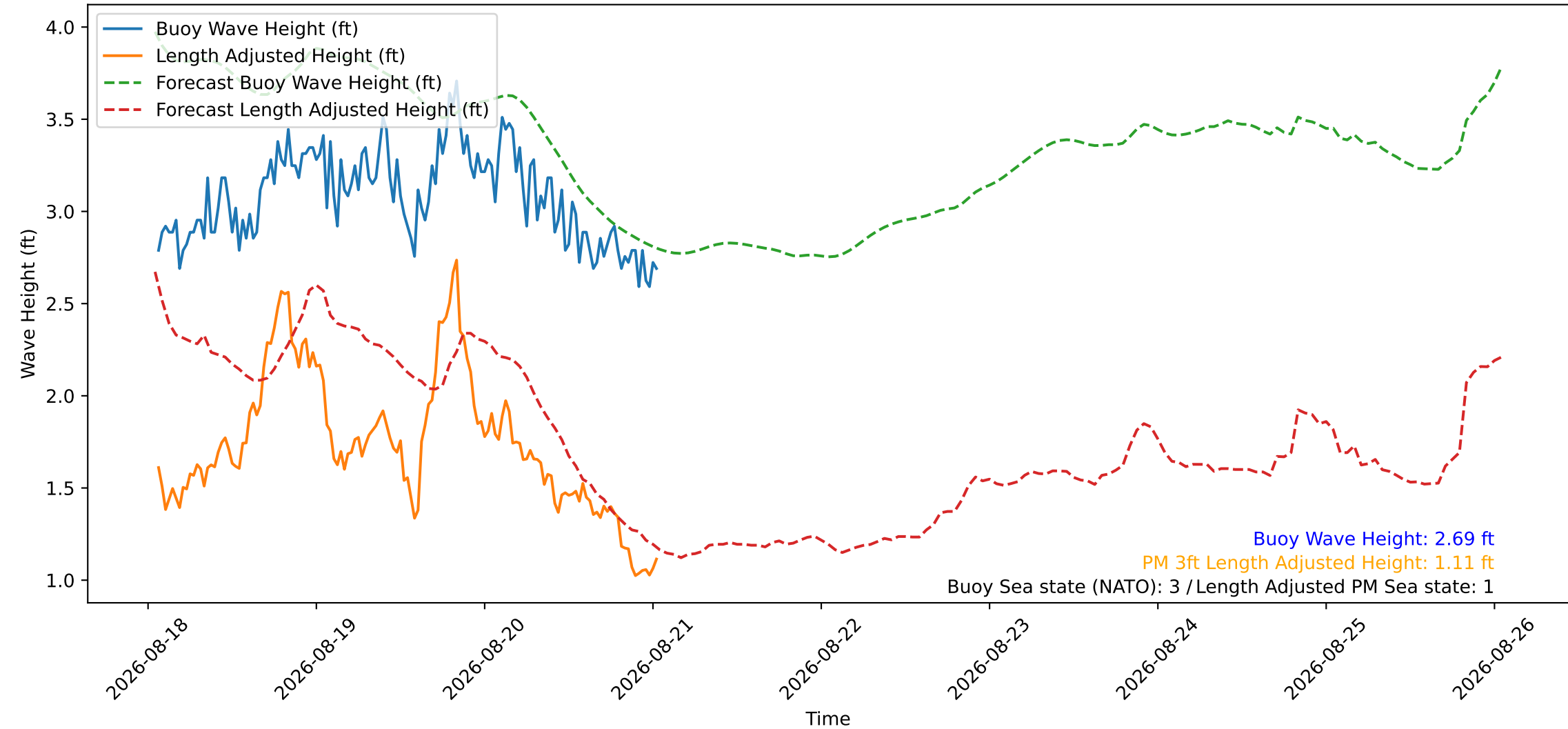
Wave Heights over Time for Green Beach at 2026-08-21 01:11:08
