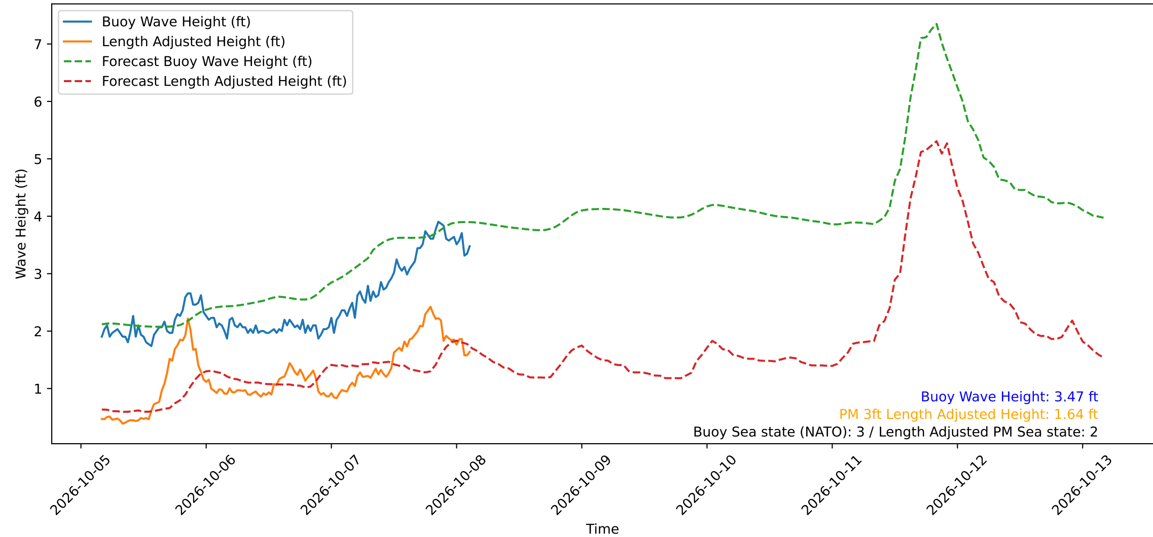
Wave Heights over Time for Red Beach at 2026-10-08 03:30:49
