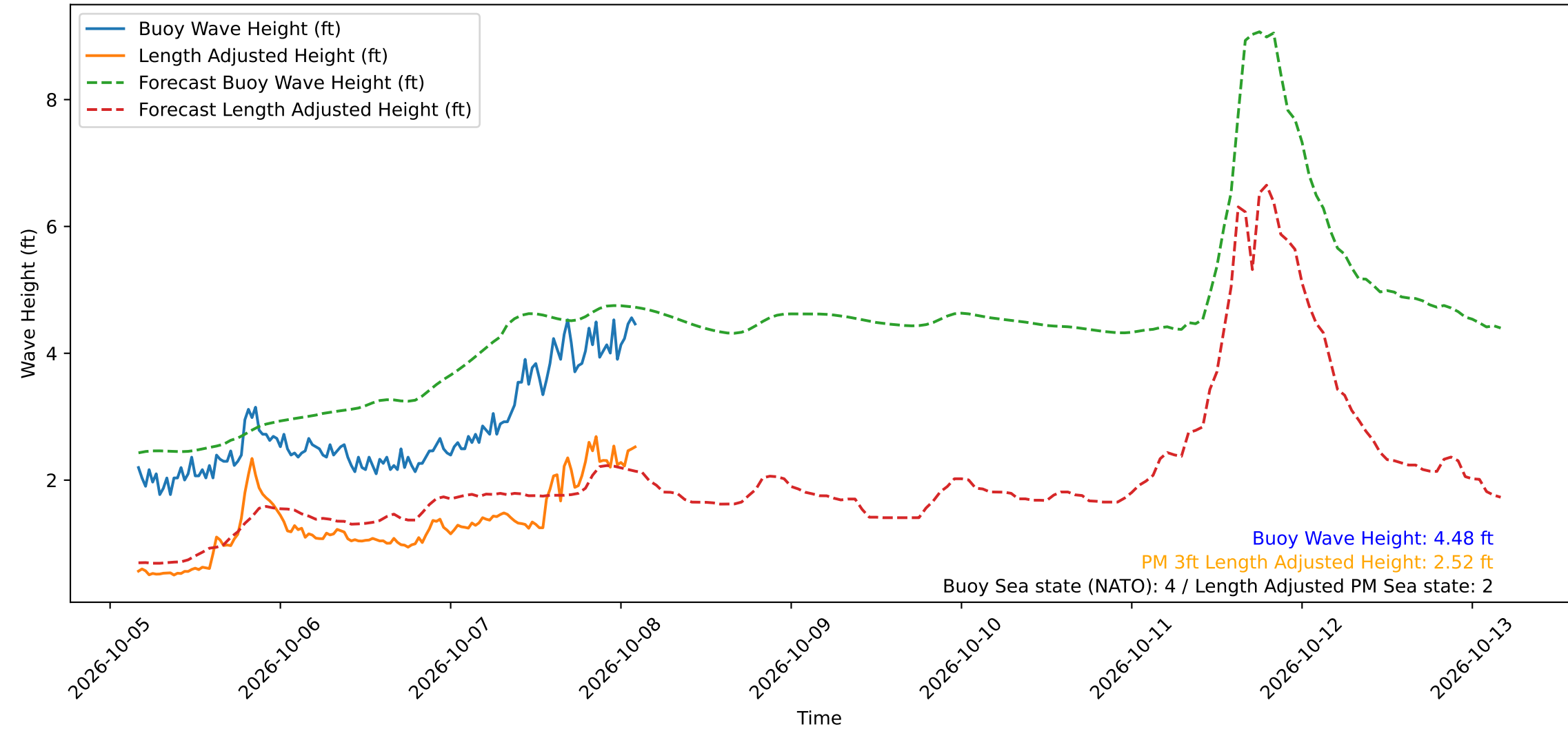
Wave Heights over Time for Green Beach at 2026-10-08 03:31:12
