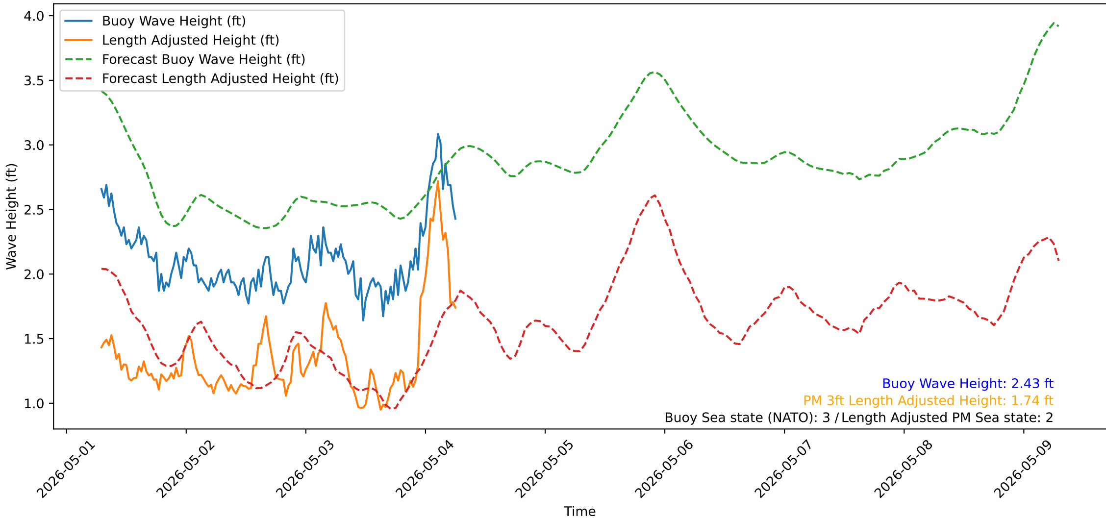
Wave Heights over Time for Oceanside Harbor at 2026-05-04 07:00:31
