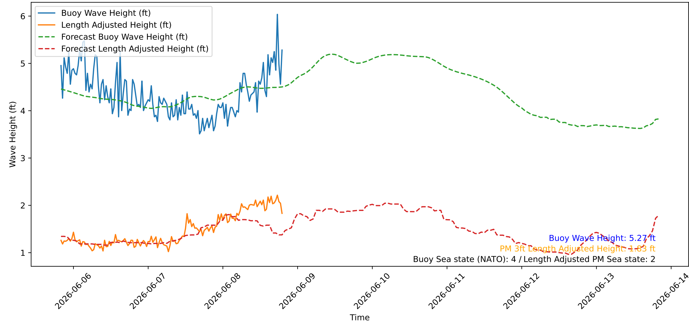
Wave Heights over Time for Oceanside Harbor at 2026-06-08 19:50:26
