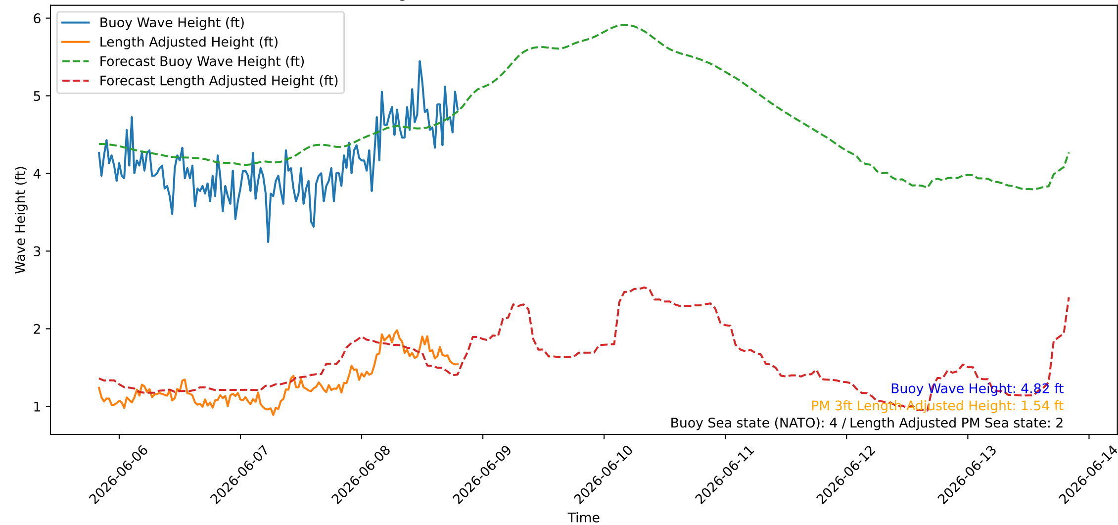
Wave Heights over Time for Green Beach at 2026-06-08 19:51:11
