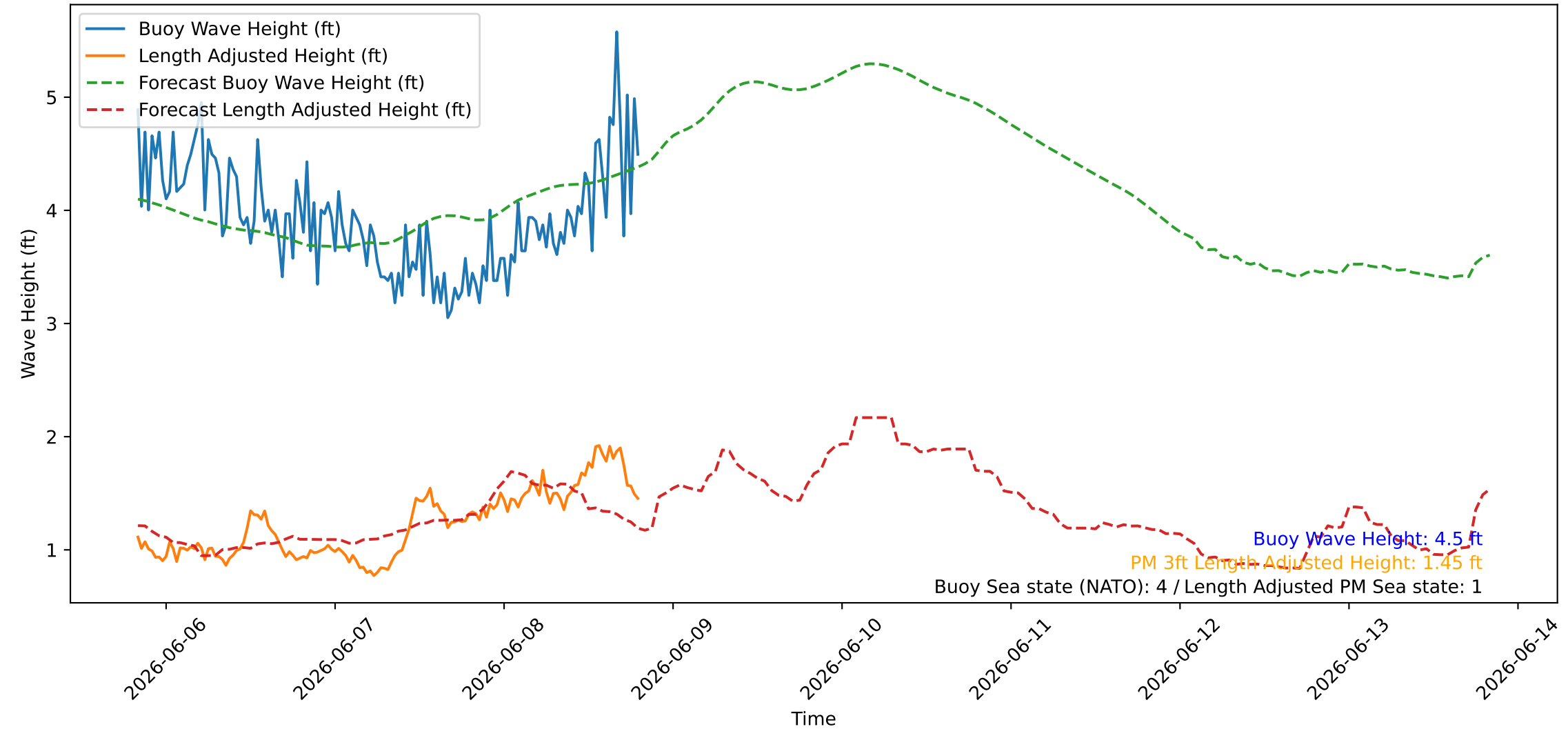
Wave Heights over Time for Red Beach at 2026-06-08 19:50:48
