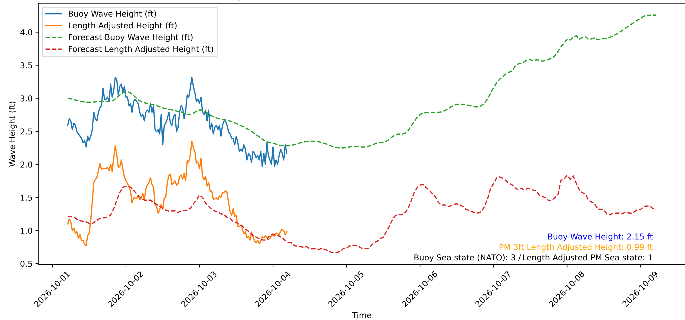
Wave Heights over Time for Oceanside Harbor at 2026-10-04 05:10:29
