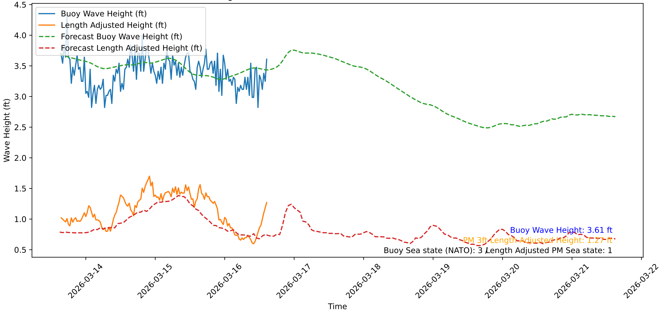
Wave Heights over Time for Green Beach at 2026-03-16 15:21:40
