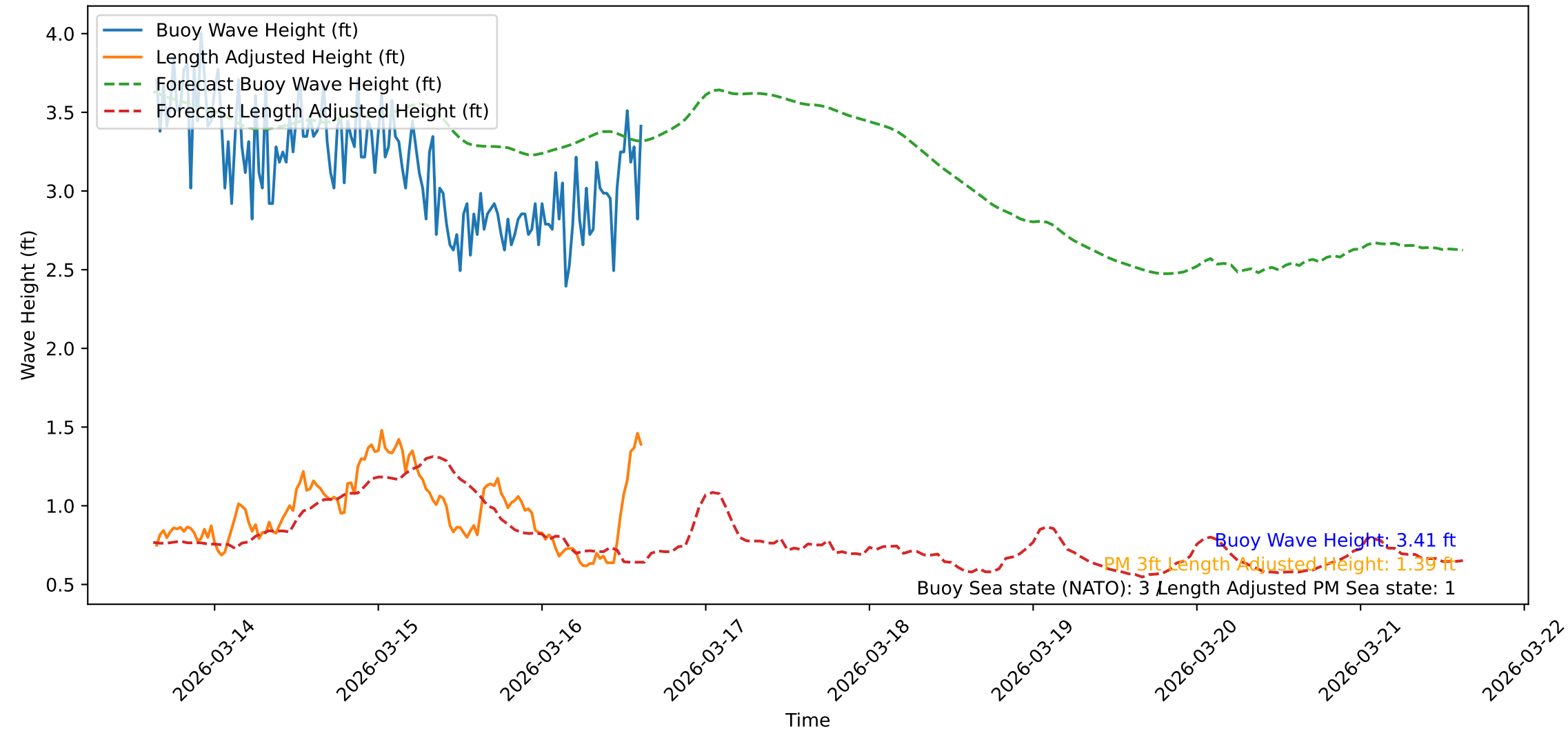
Wave Heights over Time for Oceanside Harbor at 2026-03-16 15:20:43
