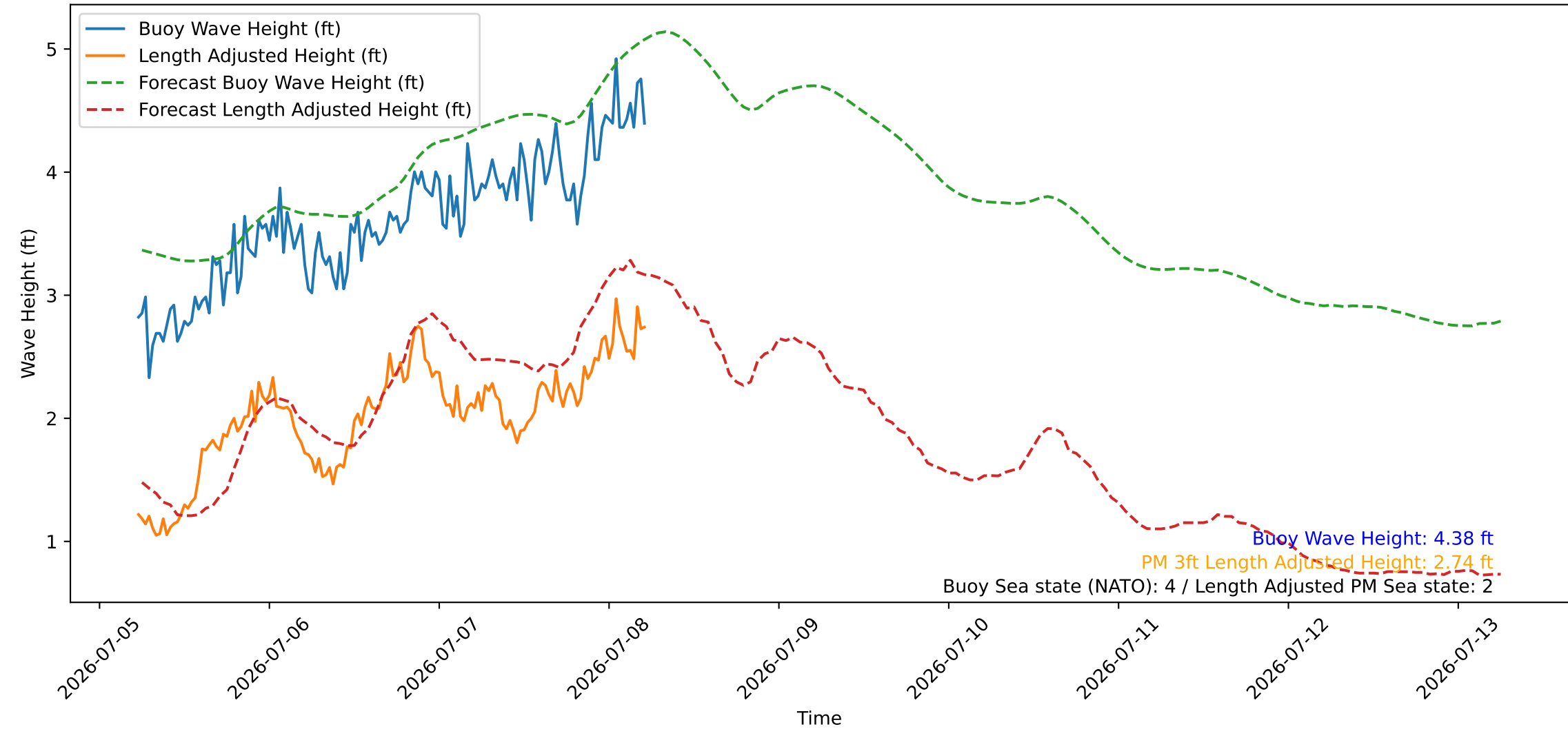
Wave Heights over Time for Oceanside Harbor at 2026-07-08 05:30:26
