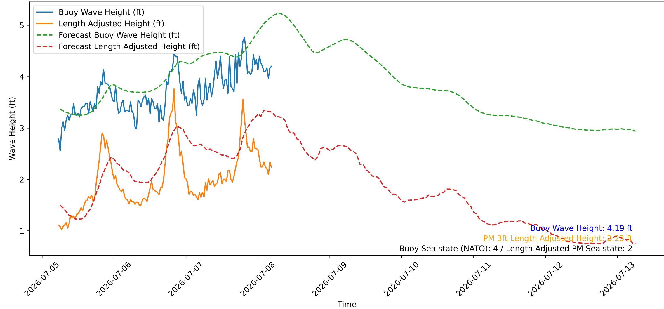
Wave Heights over Time for Green Beach at 2026-07-08 05:31:08
