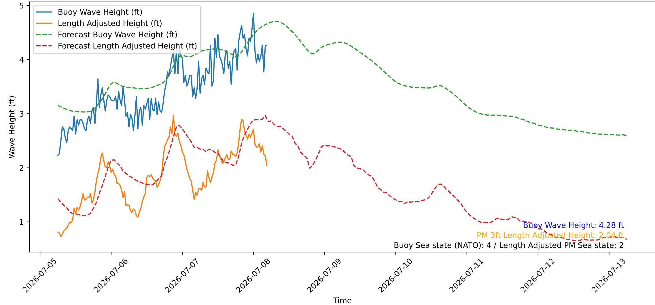
Wave Heights over Time for Red Beach at 2026-07-08 05:30:45
