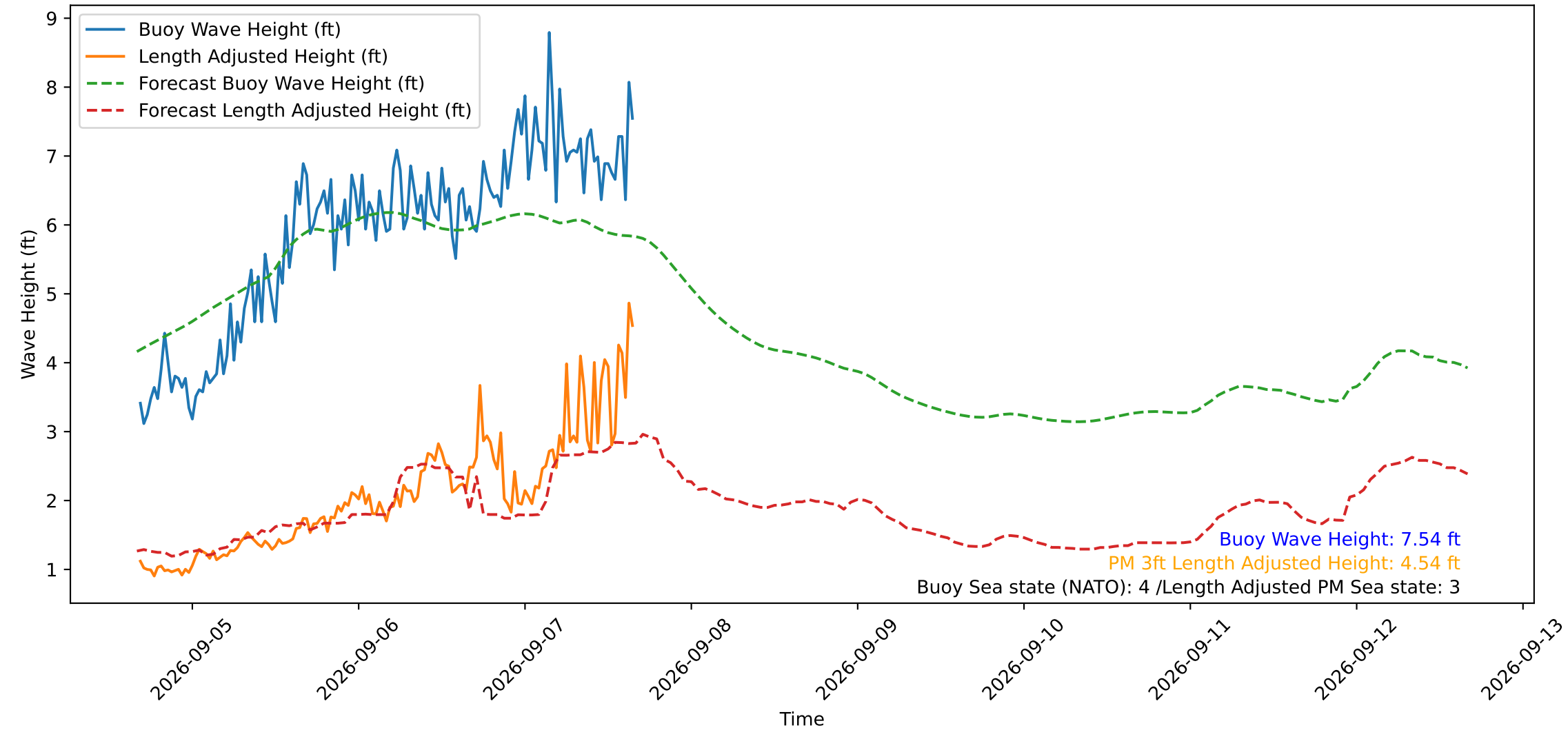
Wave Heights over Time for Green Beach at 2026-09-07 16:11:12
