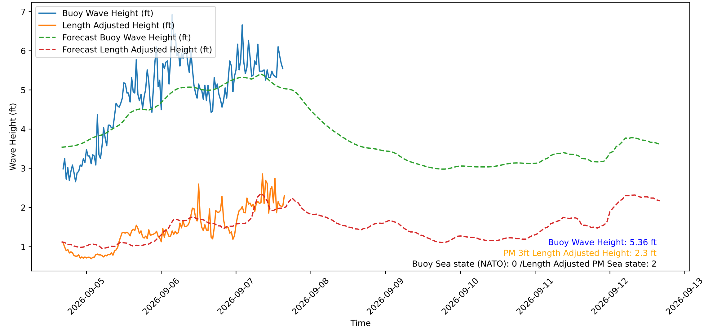
Wave Heights over Time for Red Beach at 2026-09-07 16:10:49
