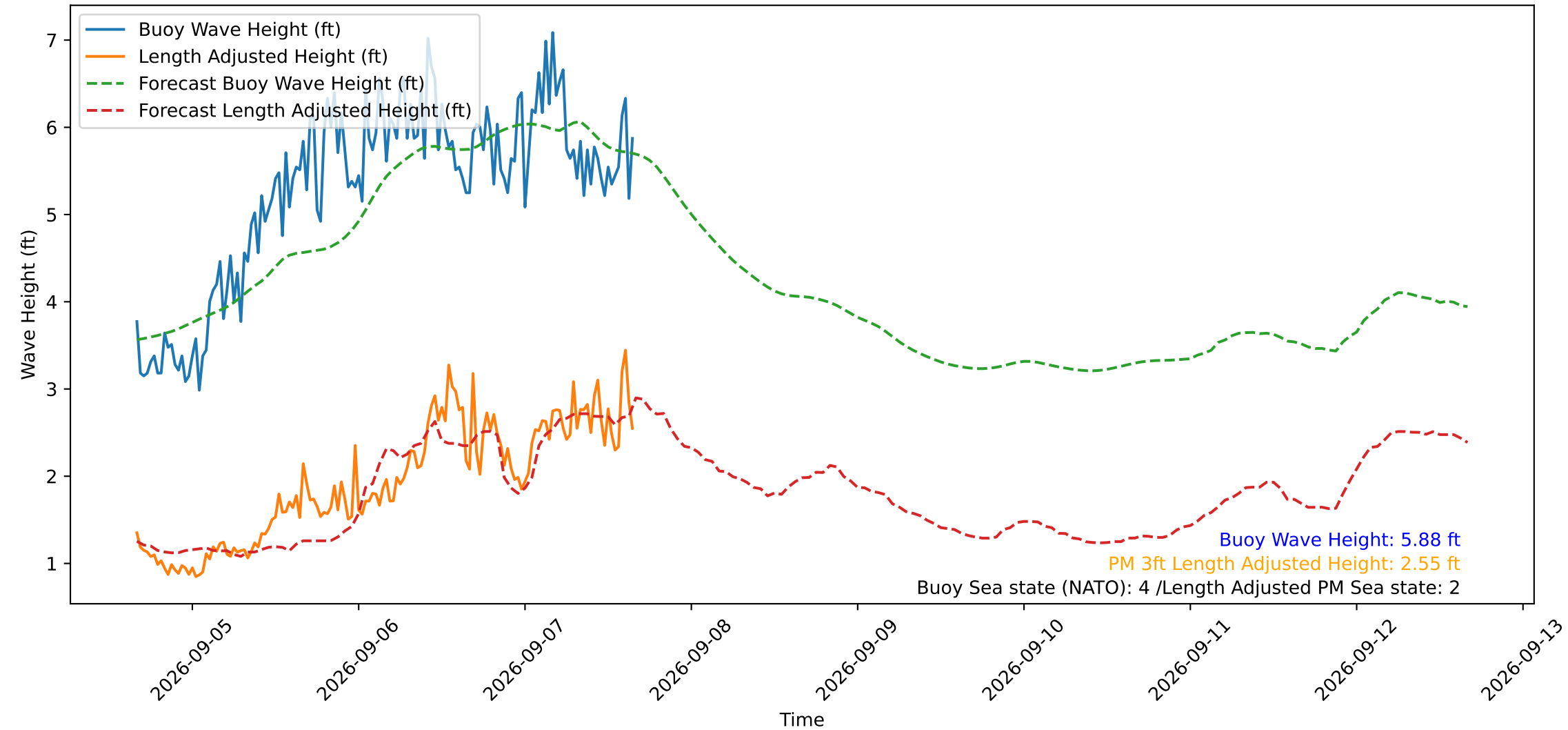
Wave Heights over Time for Oceanside Harbor at 2026-09-07 16:10:29
