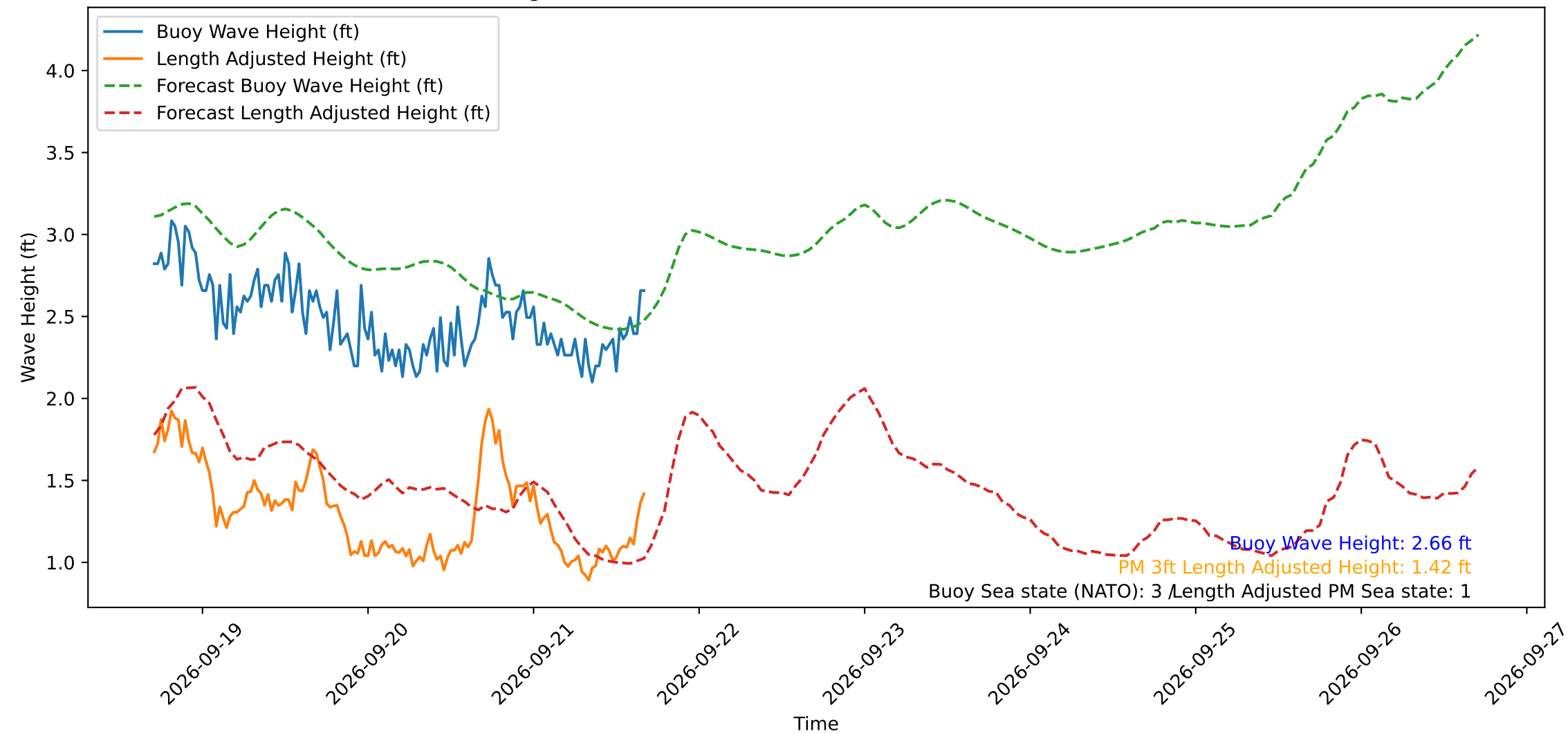
Wave Heights over Time for Oceanside Harbor at 2026-09-21 17:10:29
