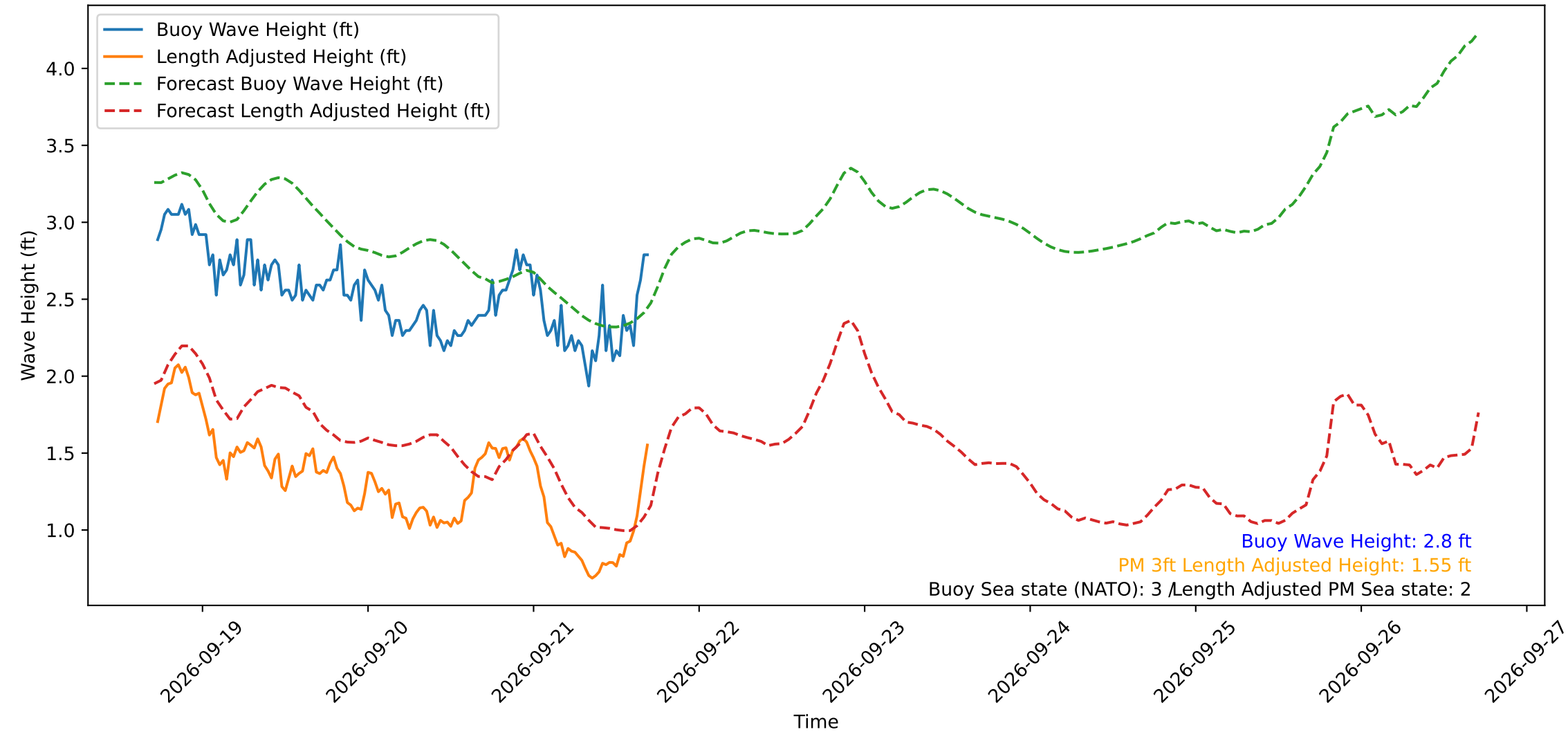
Wave Heights over Time for Green Beach at 2026-09-21 17:11:11
