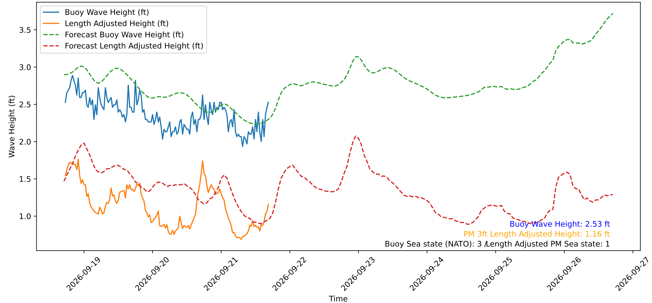
Wave Heights over Time for Red Beach at 2026-09-21 17:10:49
