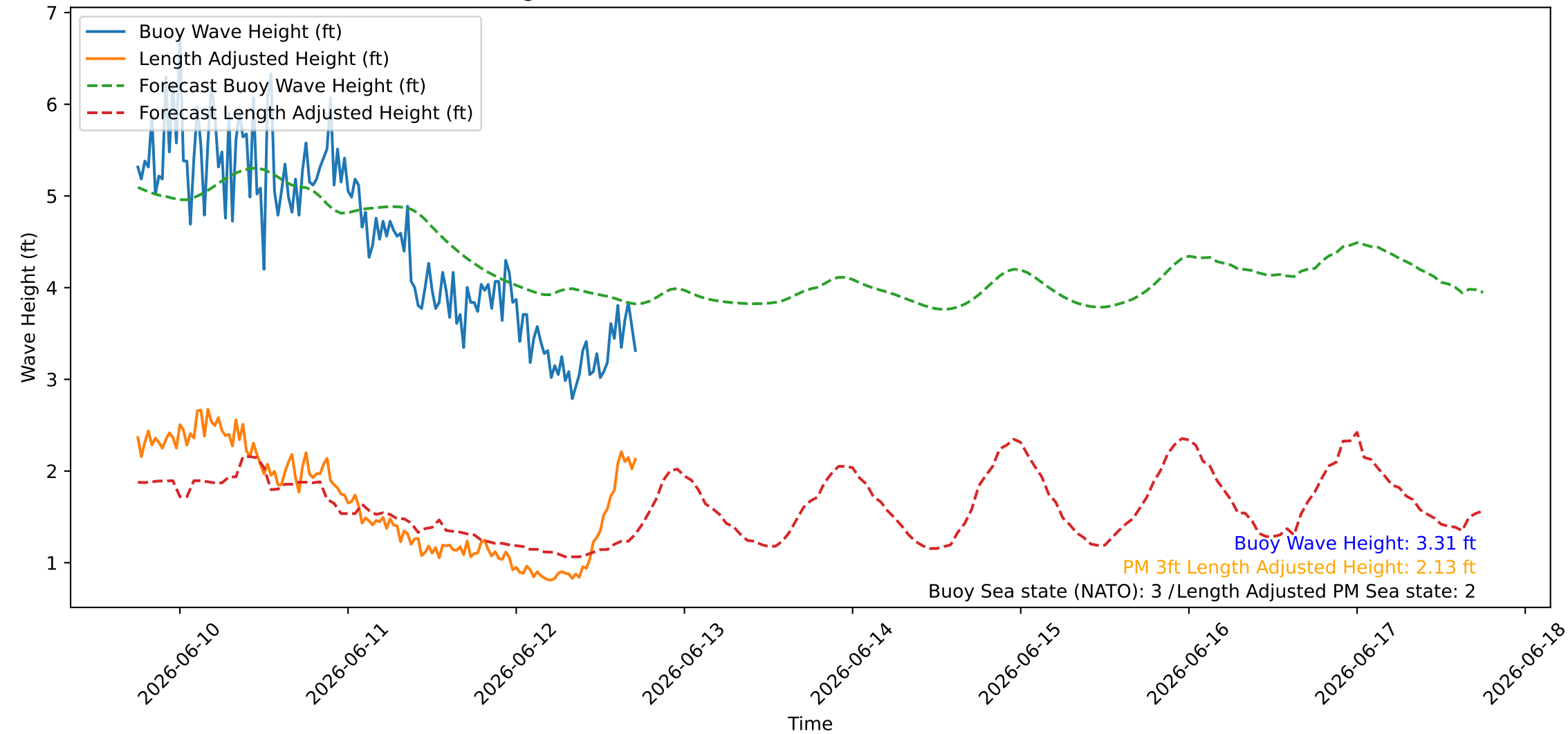
Wave Heights over Time for Oceanside Harbor at 2026-06-12 17:50:26
