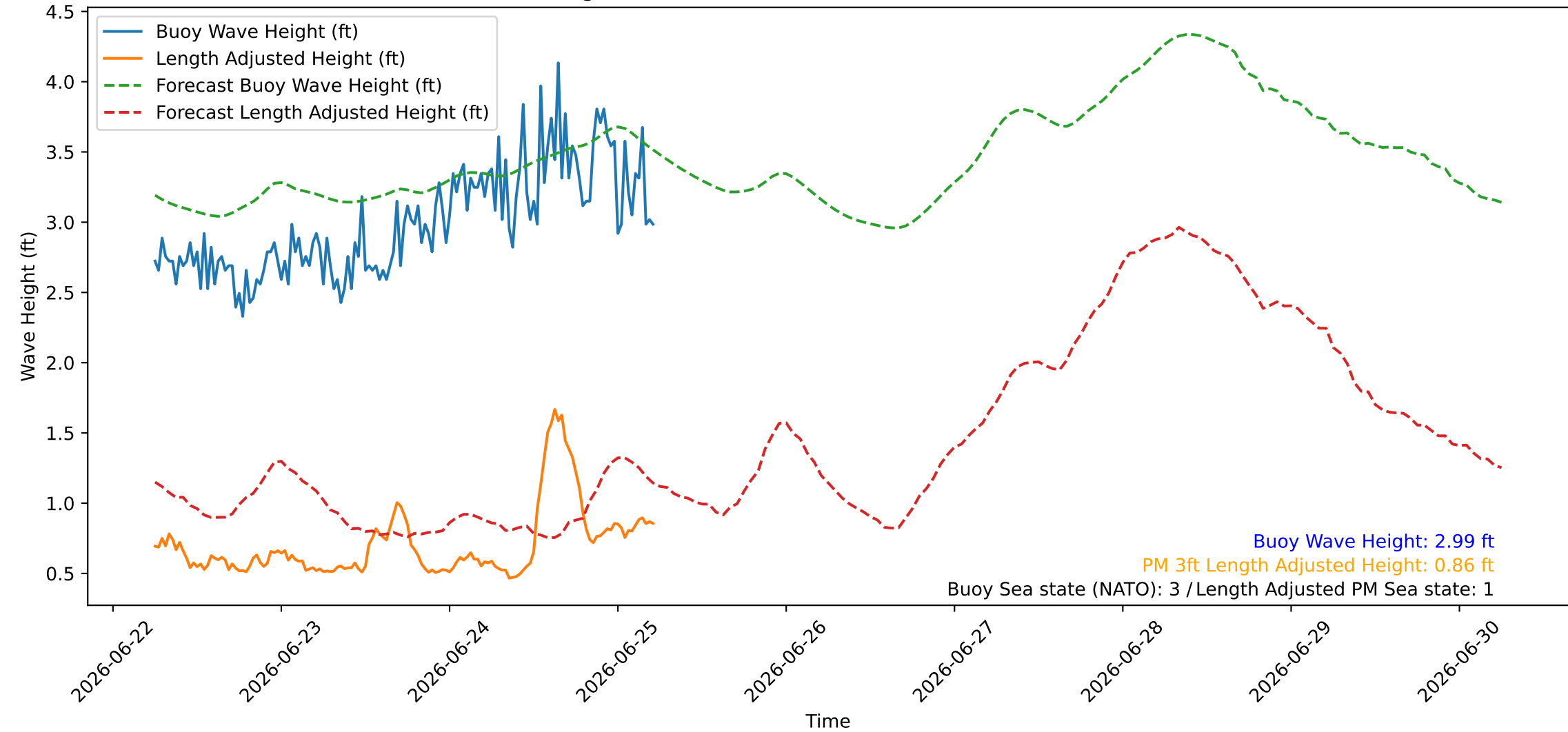
Wave Heights over Time for Red Beach at 2026-06-25 05:40:45
