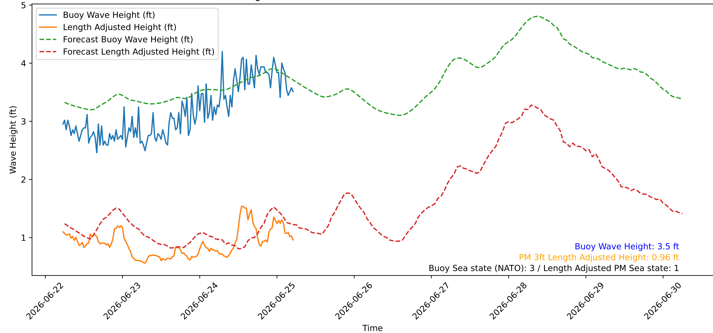
Wave Heights over Time for Green Beach at 2026-06-25 05:41:08
