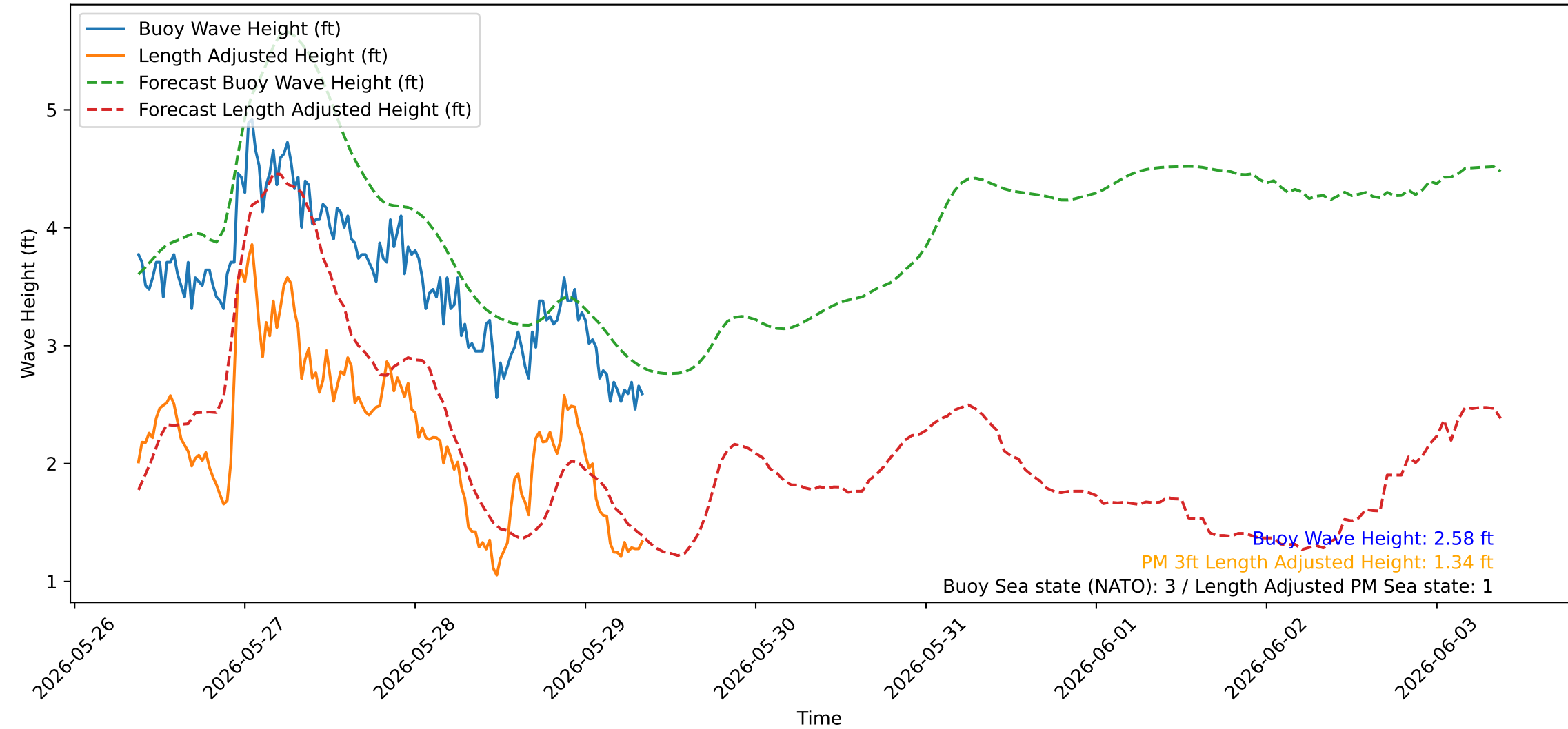
Wave Heights over Time for Green Beach at 2026-05-29 08:51:05
