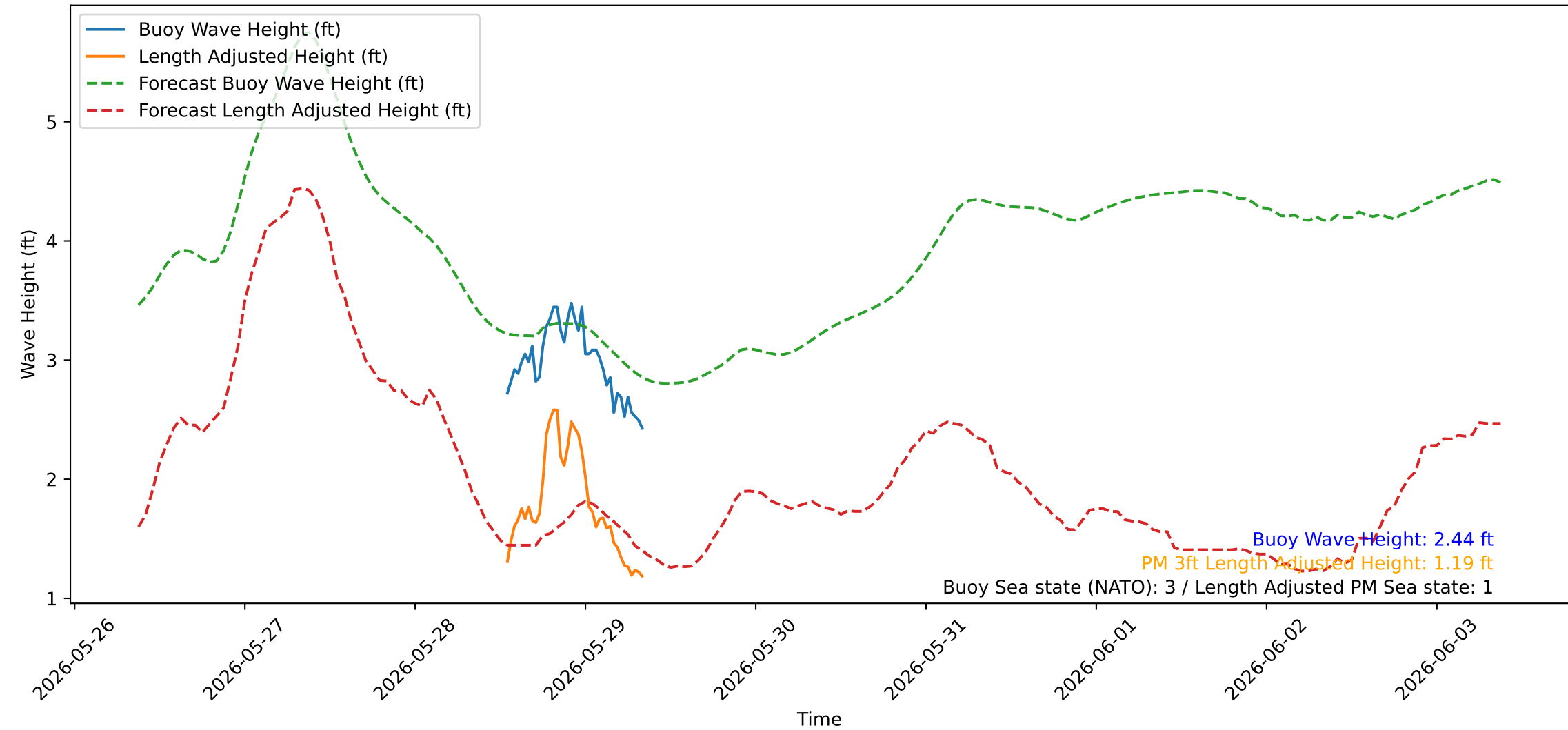
Wave Heights over Time for Oceanside Harbor at 2026-05-29 08:50:21
