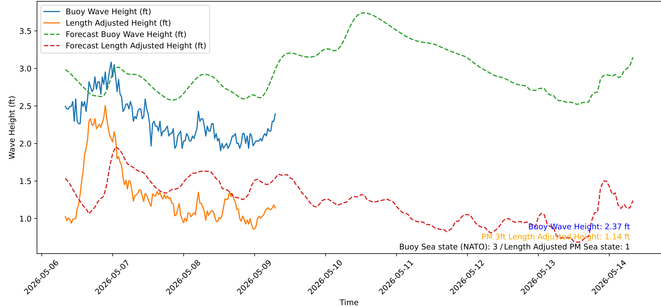
Wave Heights over Time for Red Beach at 2026-05-09 07:50:52
