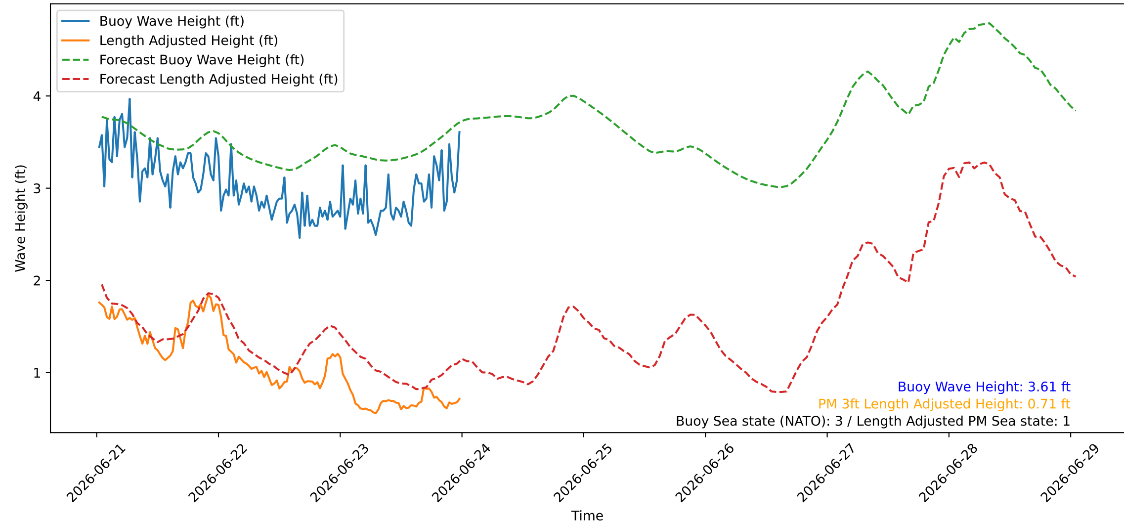
Wave Heights over Time for Green Beach at 2026-06-24 00:31:07
