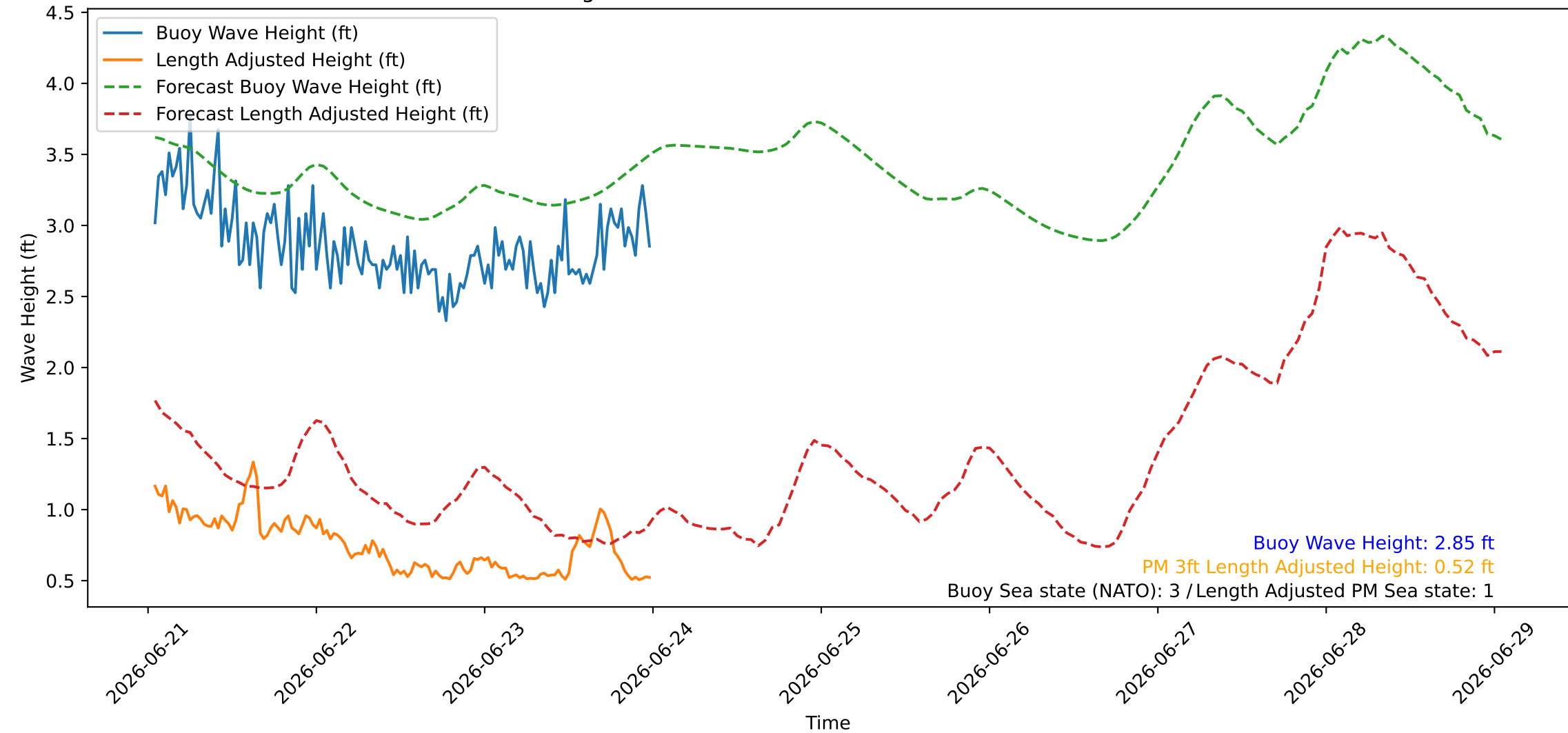
Wave Heights over Time for Red Beach at 2026-06-24 00:30:45
