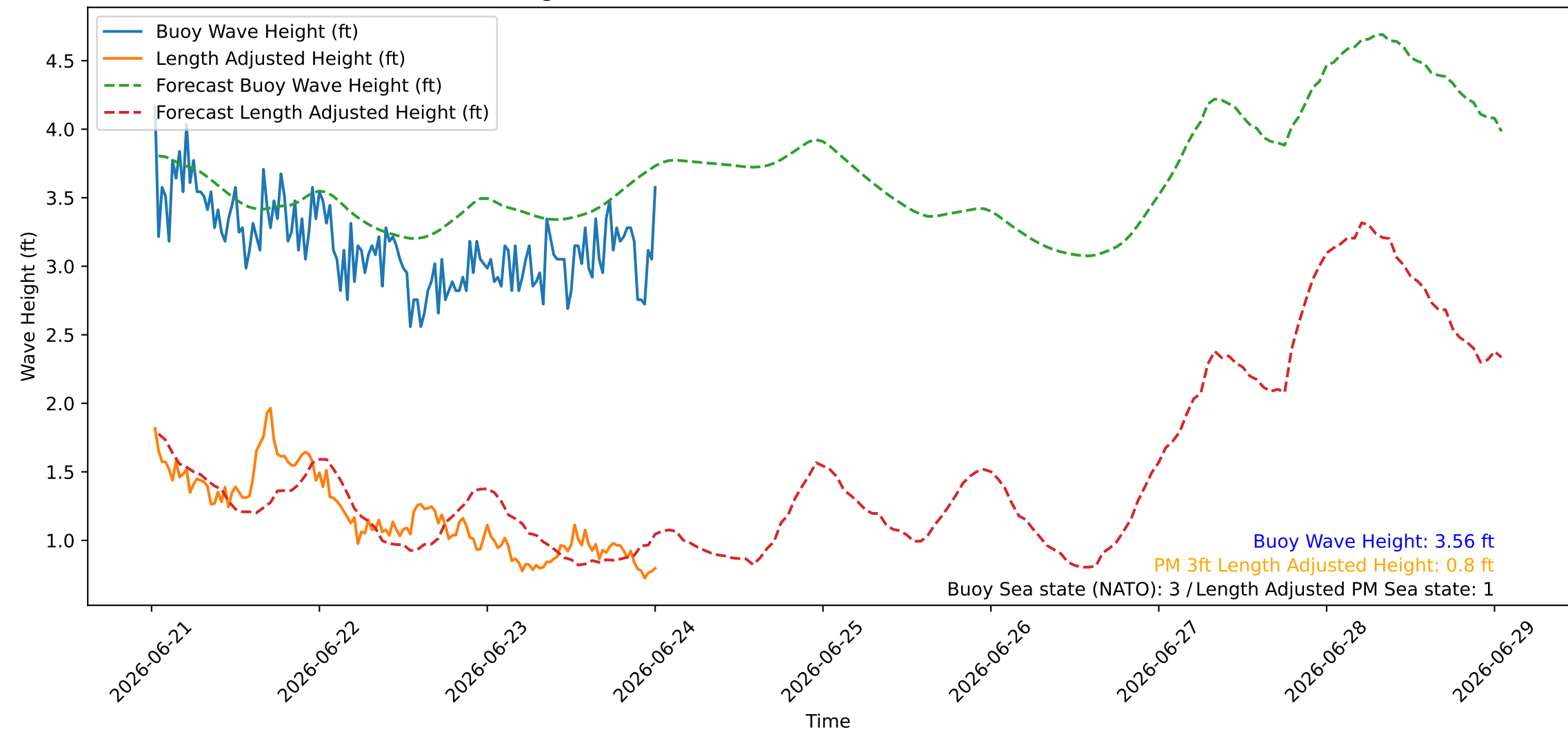
Wave Heights over Time for Oceanside Harbor at 2026-06-24 00:30:26
