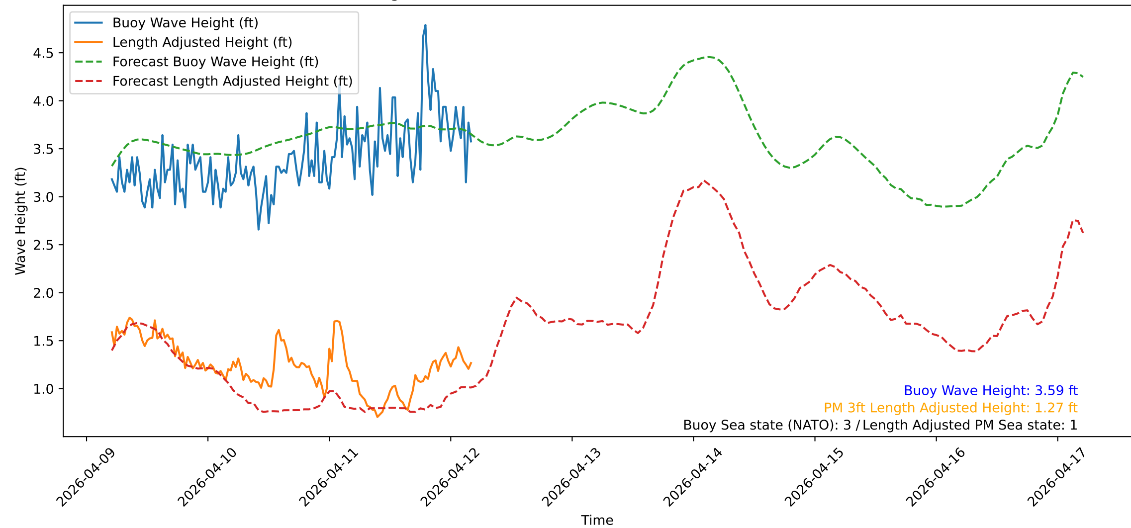
Wave Heights over Time for Oceanside Harbor at 2026-04-12 05:10:31
