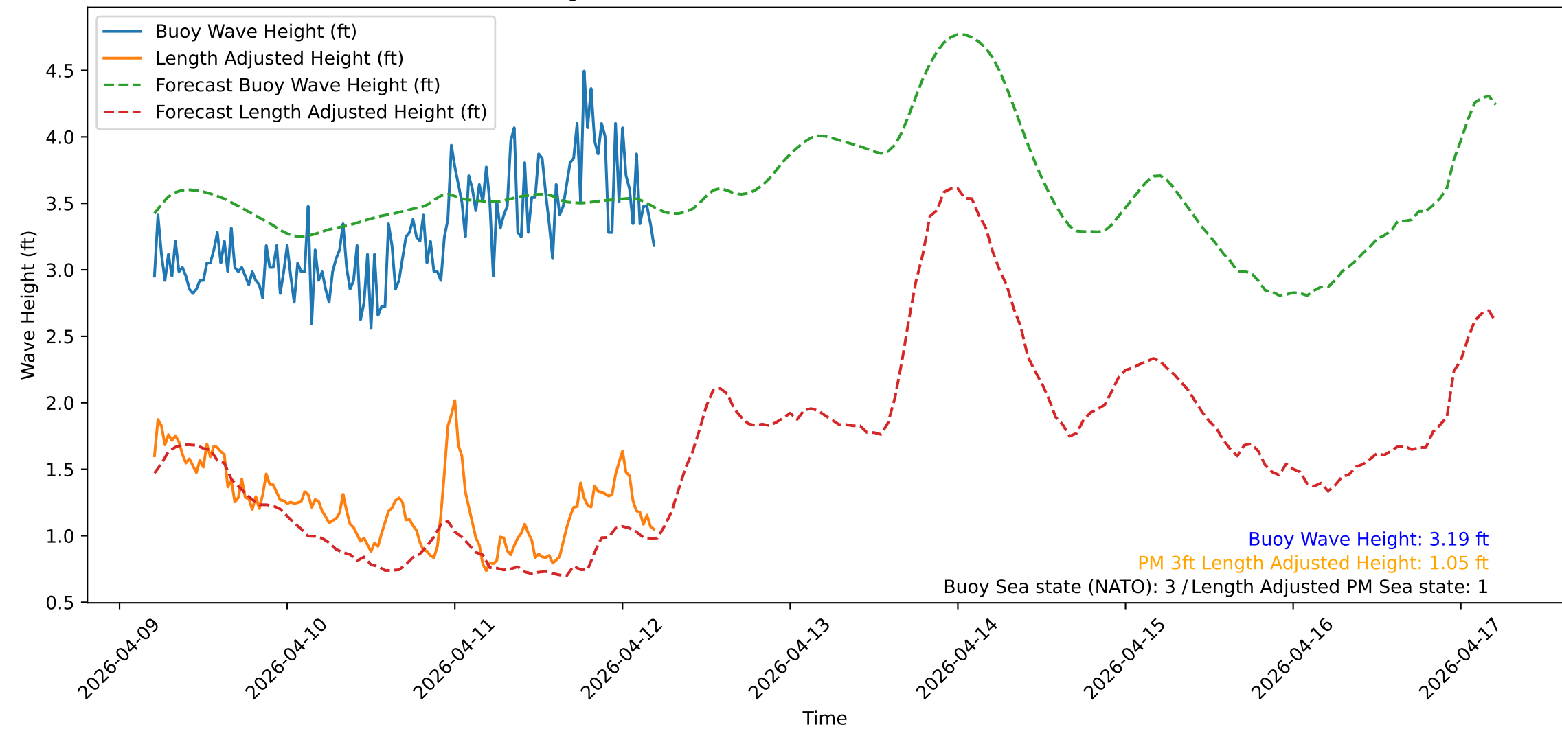
Wave Heights over Time for Green Beach at 2026-04-12 05:11:12
