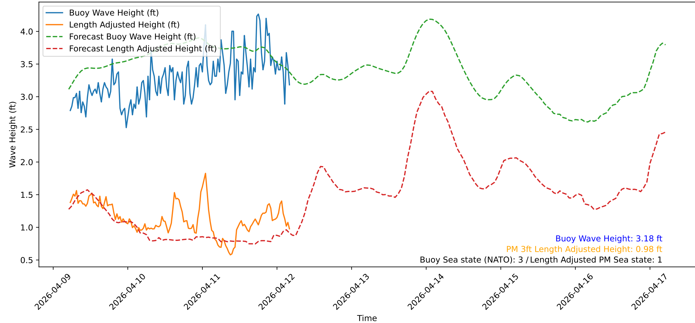
Wave Heights over Time for Red Beach at 2026-04-12 05:10:50
